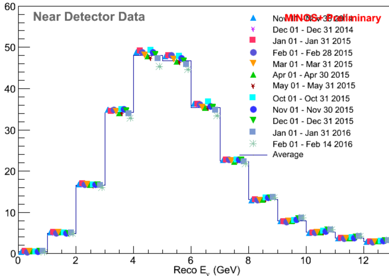
Neutrino Energy Spectrum Stability (PQ and NQ)
