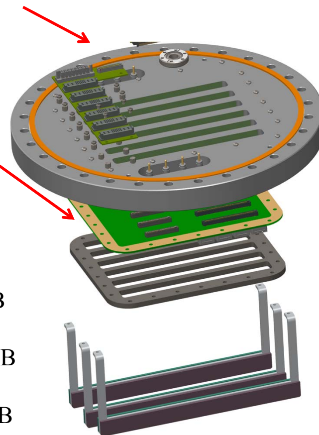
Example of CE flange/ feedthrough design
