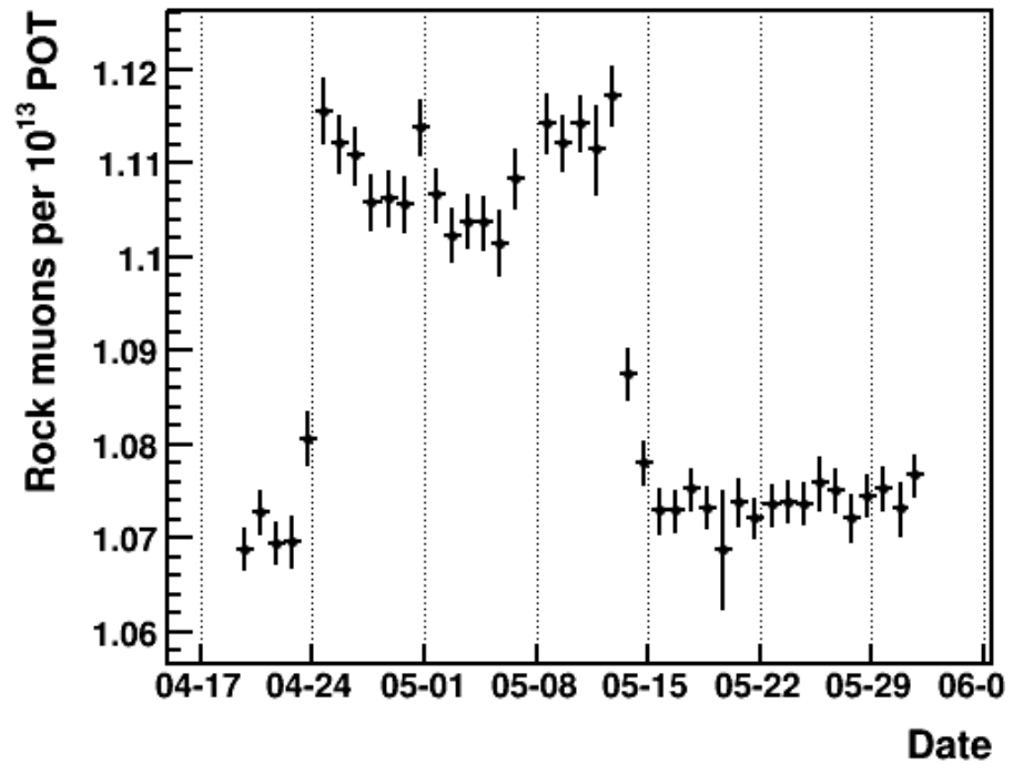
Rock Muons/POT
