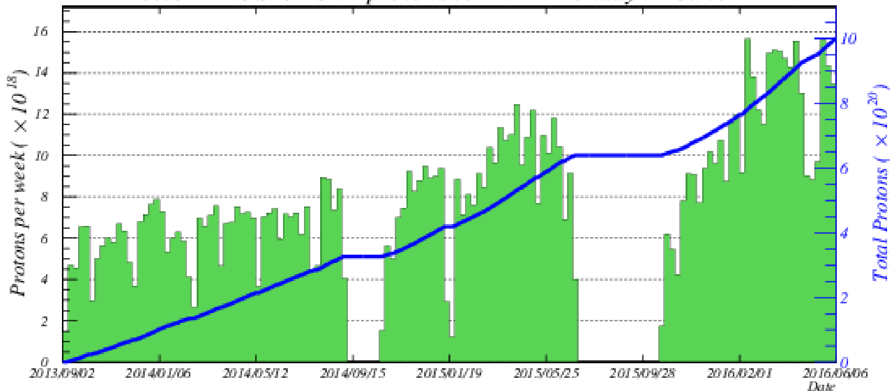
Total MINOS+/NOvA protons to 00:00 Monday 06 June 2016
