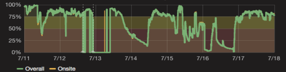
CPU Efficiency
