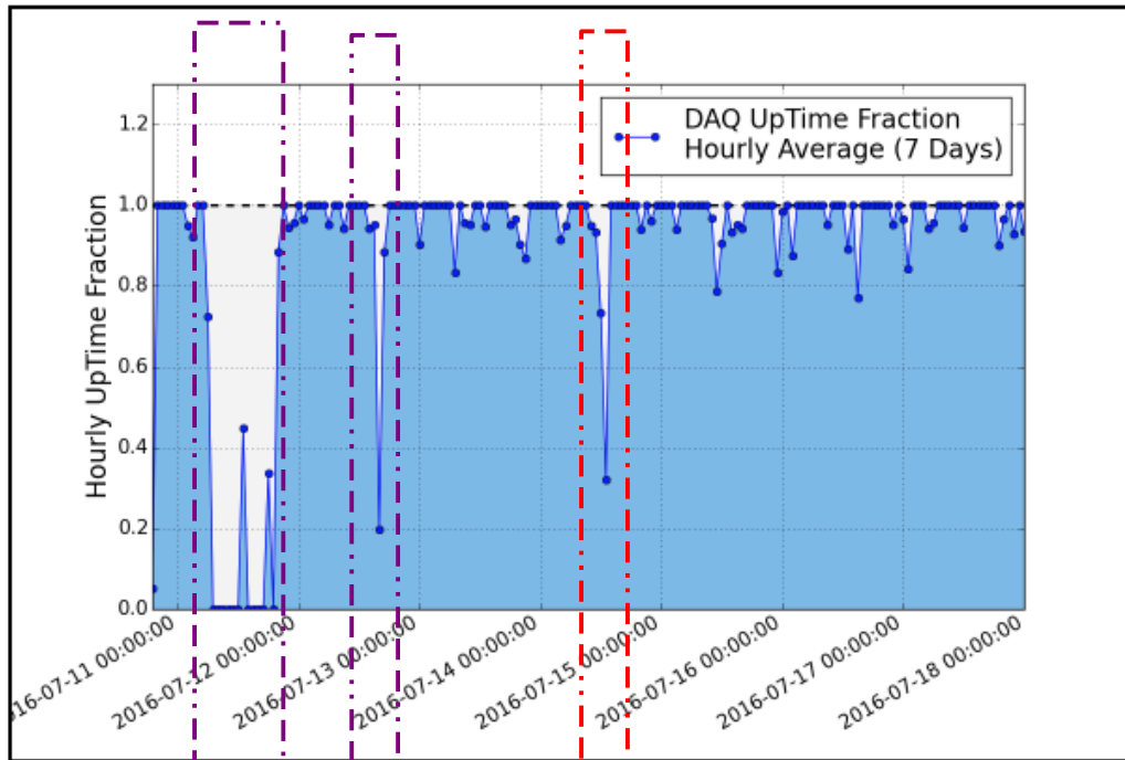
DAQ UpTime (Hourly, Past Week)
