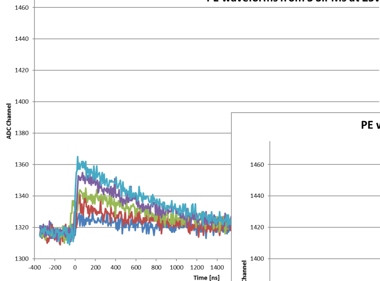
PE waveforms from 3 SiPMs at 25v
