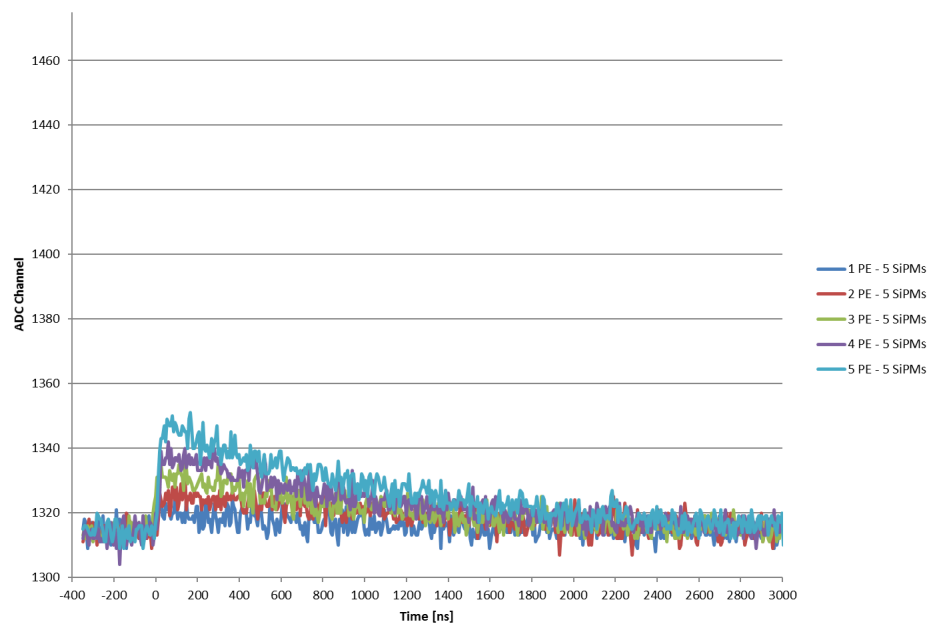
PE waveforms from 5 SiPMs at 25v
