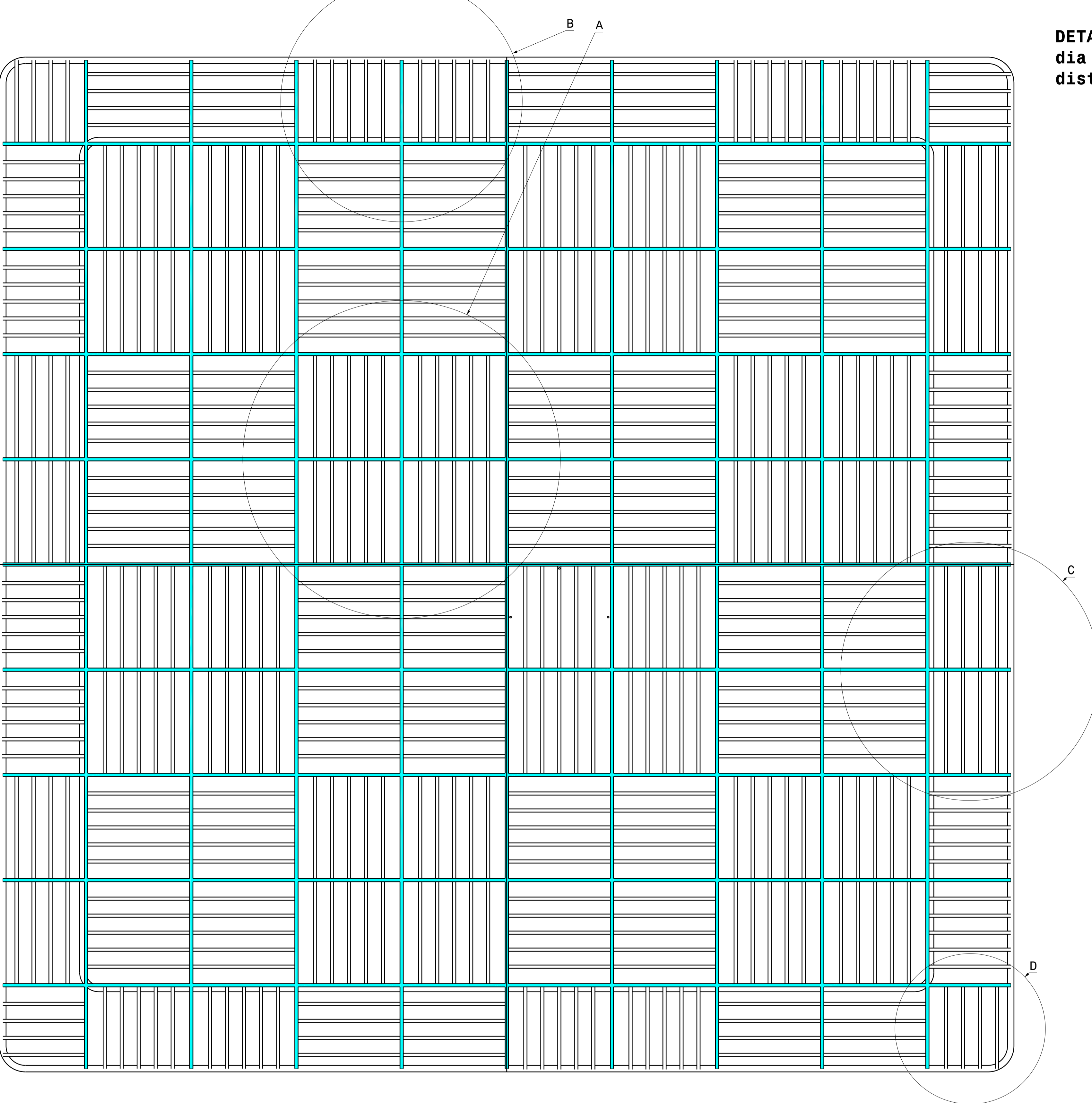
DETAIL D: #4 times dia pipes 20mm distanse 105
