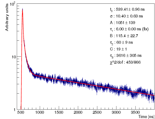
Scintillation time in GAR (1000 mBar, 215 K)
