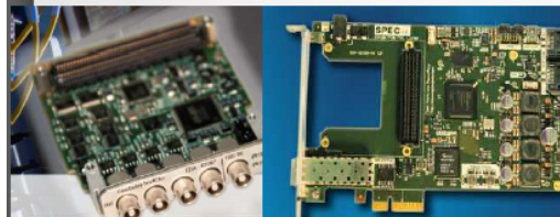
FMC Fine Delay 1 ns 4 channels
