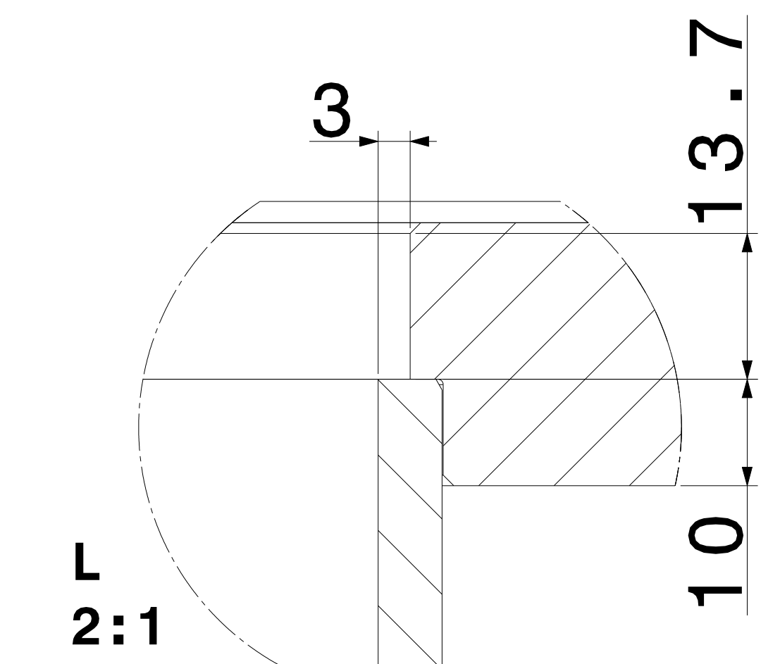
Flange CF-250
