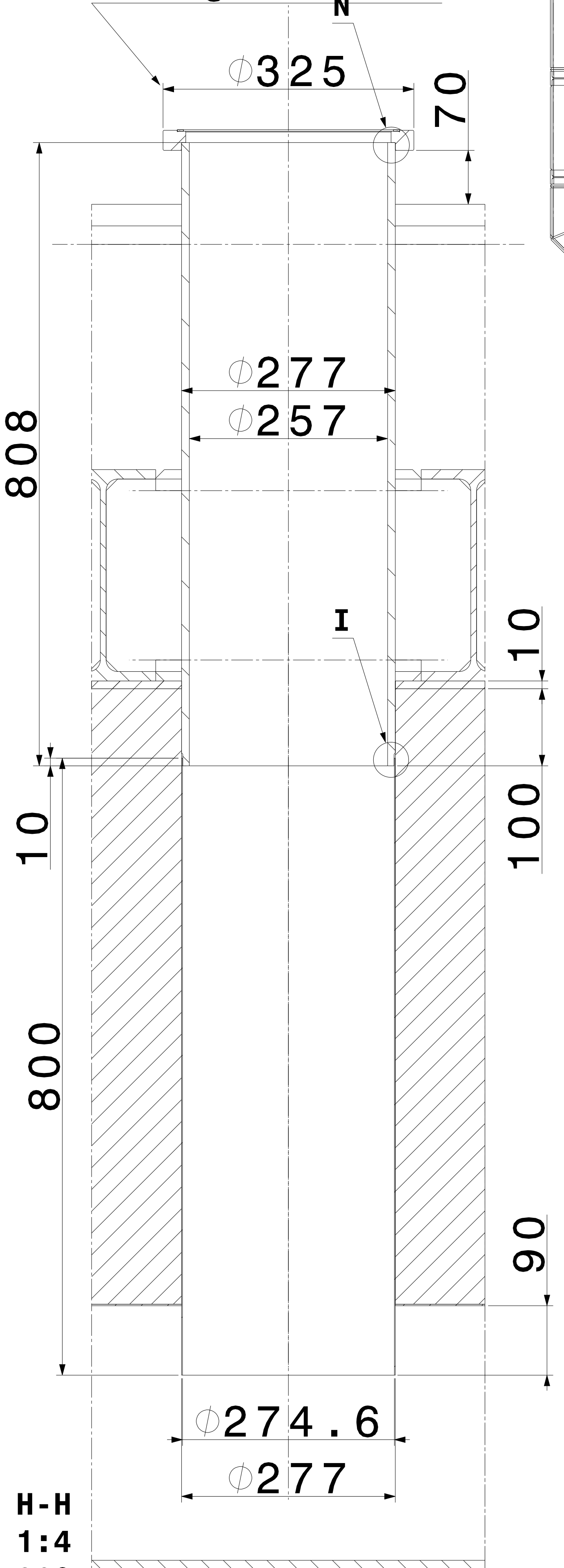
Flange CF-273
