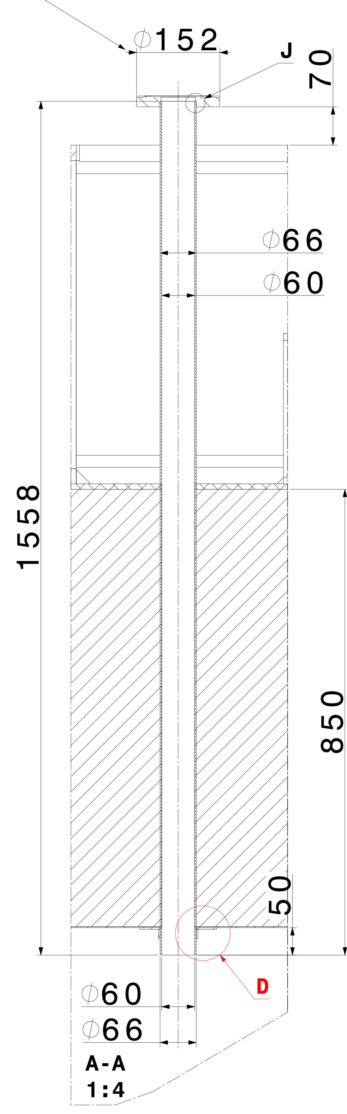
Flange CF-100
