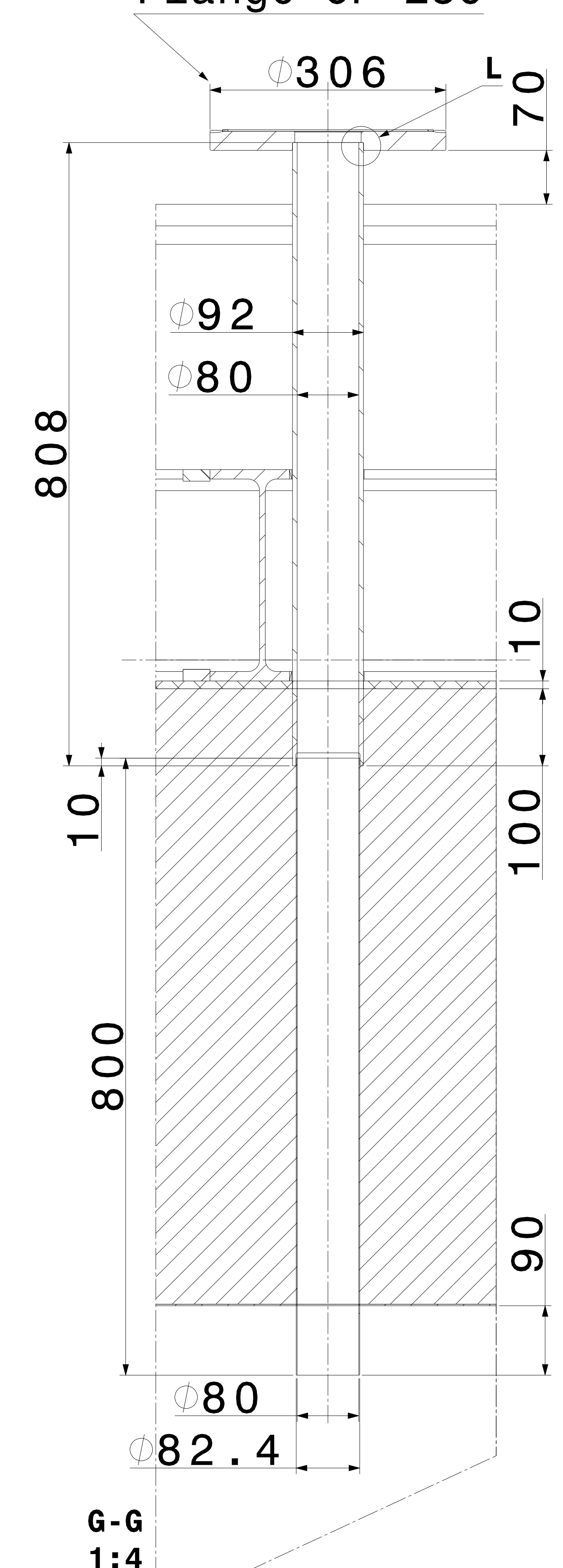
Flange CF-250
