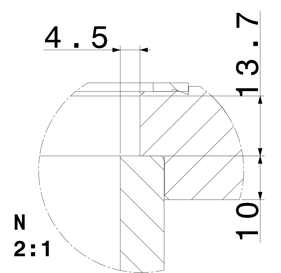
Flange CF-273
