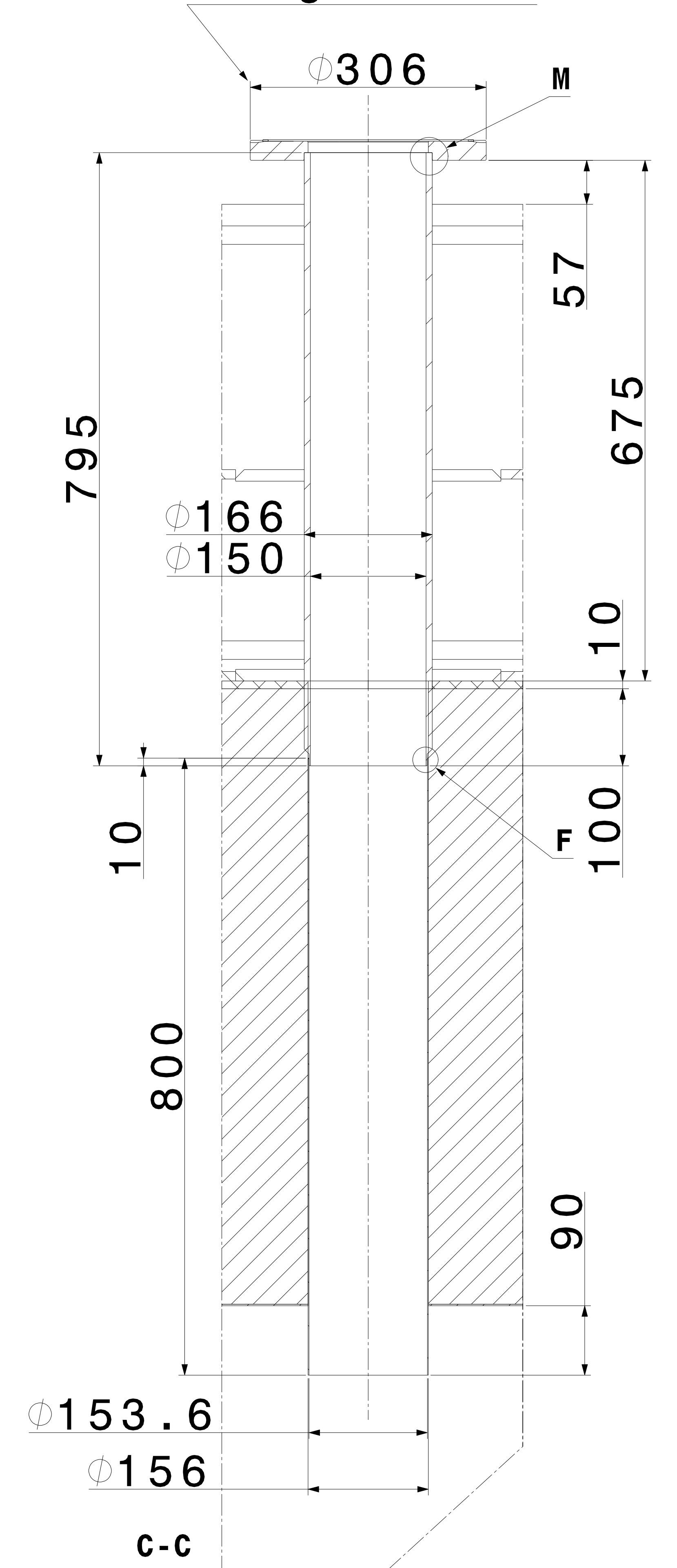
Flange CF-250
