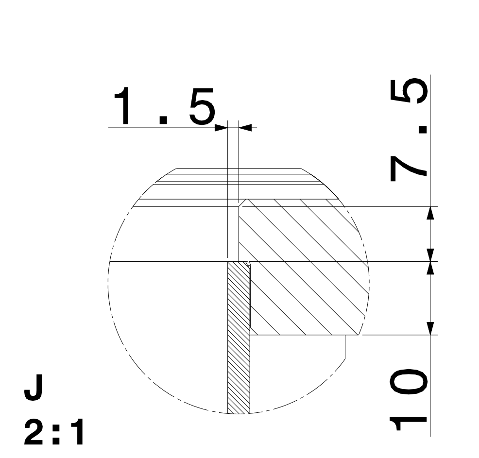
Flange CF-100
