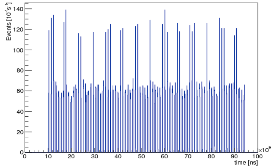
Pulsing of quads as seen in trackers
