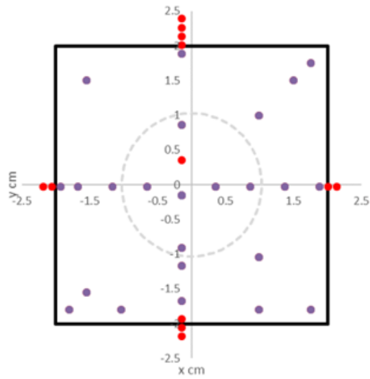
Figure 10: Results from a 4x4 tile made of SCSN81, with Tyvek wrapping.
