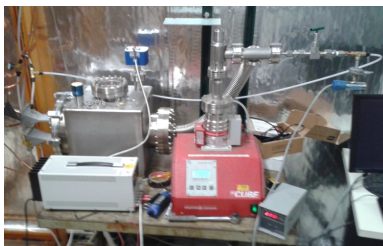
Figure 13: Setup at MTest in the gas room. the module is placed inside the vacuum tank and pumped down using the Pfeiffer turbo vacuum pump. The gas is supplied from MTest.
