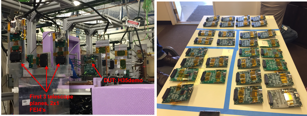
Figure 24: Left: The test beam setup used for the silicon CMOS studies includes 6 planes of pixel detectors and a cold box for the DUT. Right: An array of some of the H35demo samples laid out after testing.
