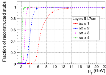
Figure 23: Stub efficiency v.s. emulated track momentum
