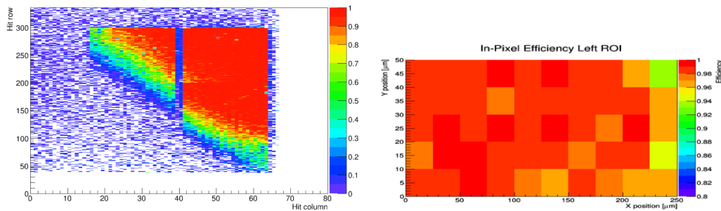
Figure 25: Left: An example of the tracking efficiency map with a gradient in efficiency due to a gradient in the glue thickness. Right: The efficiency of the fully digital CMOS matrix with an average of 98% tracking efficiency.
