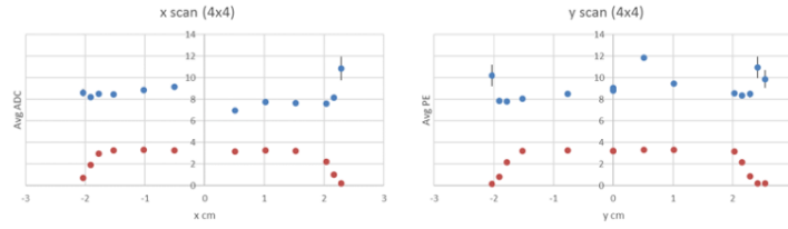
Figure 11: Light yield of different points in x and y scans.
