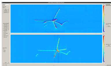
Figure 6: LArIAT Run II antiproton candidate event.
