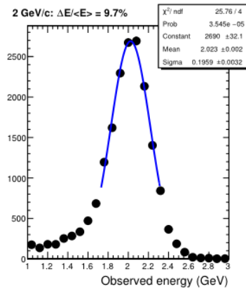
Figure 18: The EMCal energy response for 2 GeV/c electrons.
