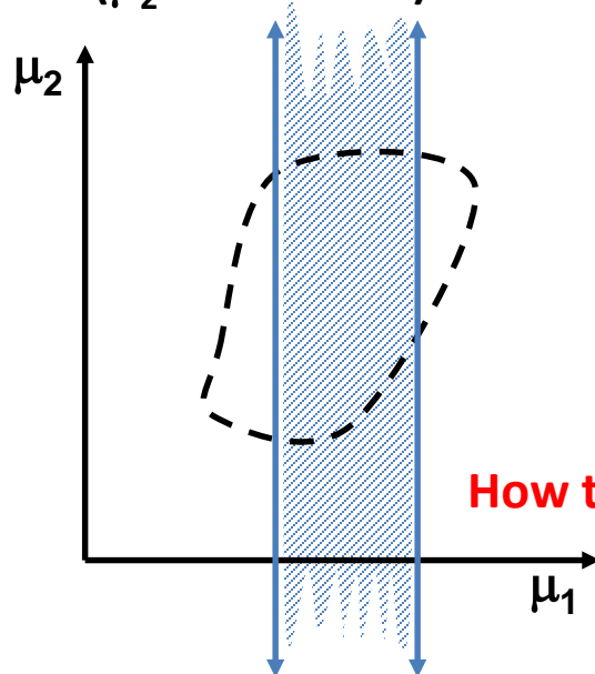
2D region to get 1D 68% C.L. interval for \mu_1 ( \mu_2 is nuisance)
