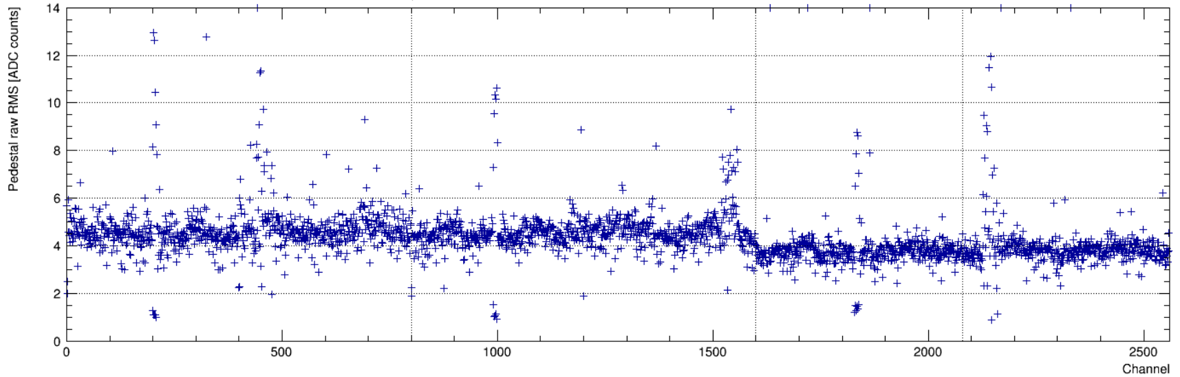
ADC pedestal raw RMS for run 4458 event 141 TPS set 0 (APA 3: US-RaS)
