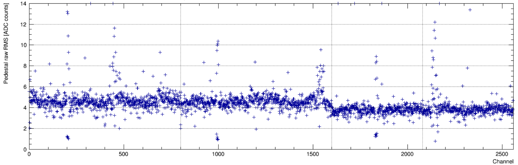
ADC pedestal raw RMS for run 4462 event 2 TPS set 0 (APA 3: US-RaS)
