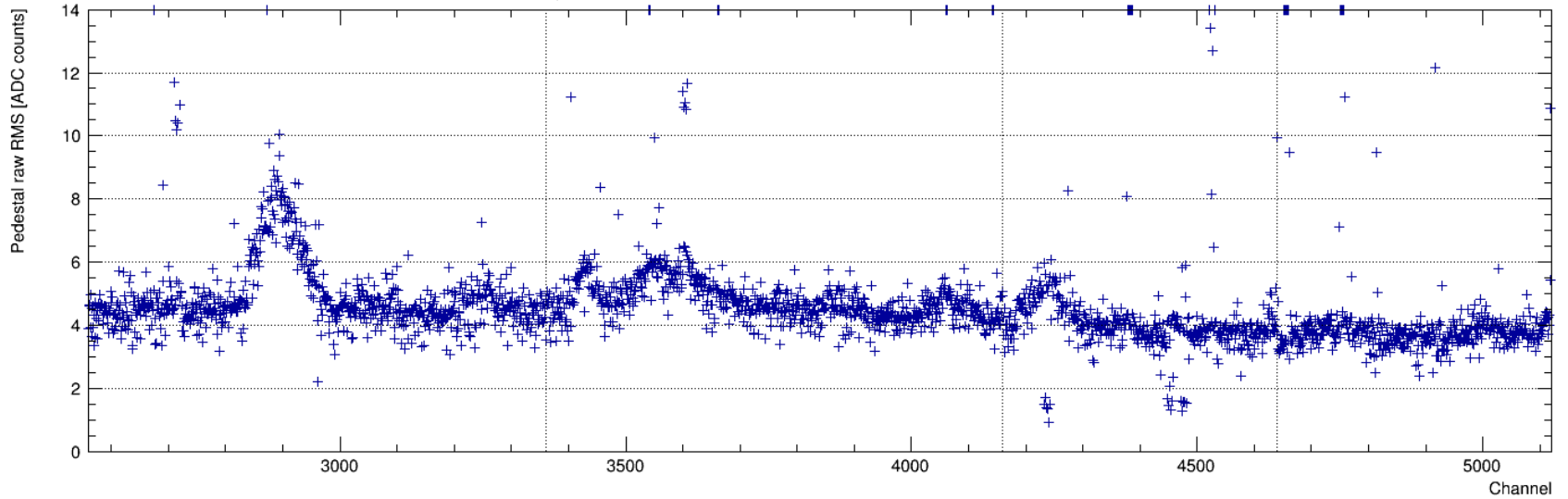
ADC pedestal raw RMS for run 4462 event 2 TPS set 1 (APA 5: US-DaS)
