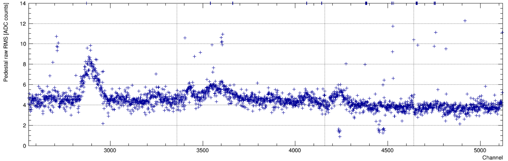
ADC pedestal raw RMS for run 4458 event 141 TPS set 1 (APA 5: US-DaS)
