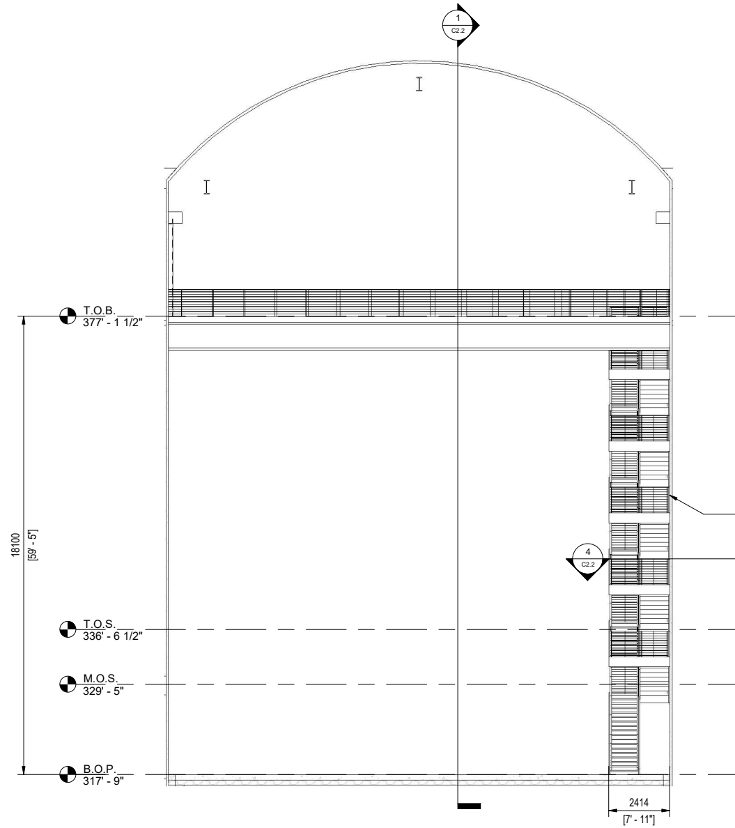
2 BRIDGE // STAIR SECTION 1 1:100
