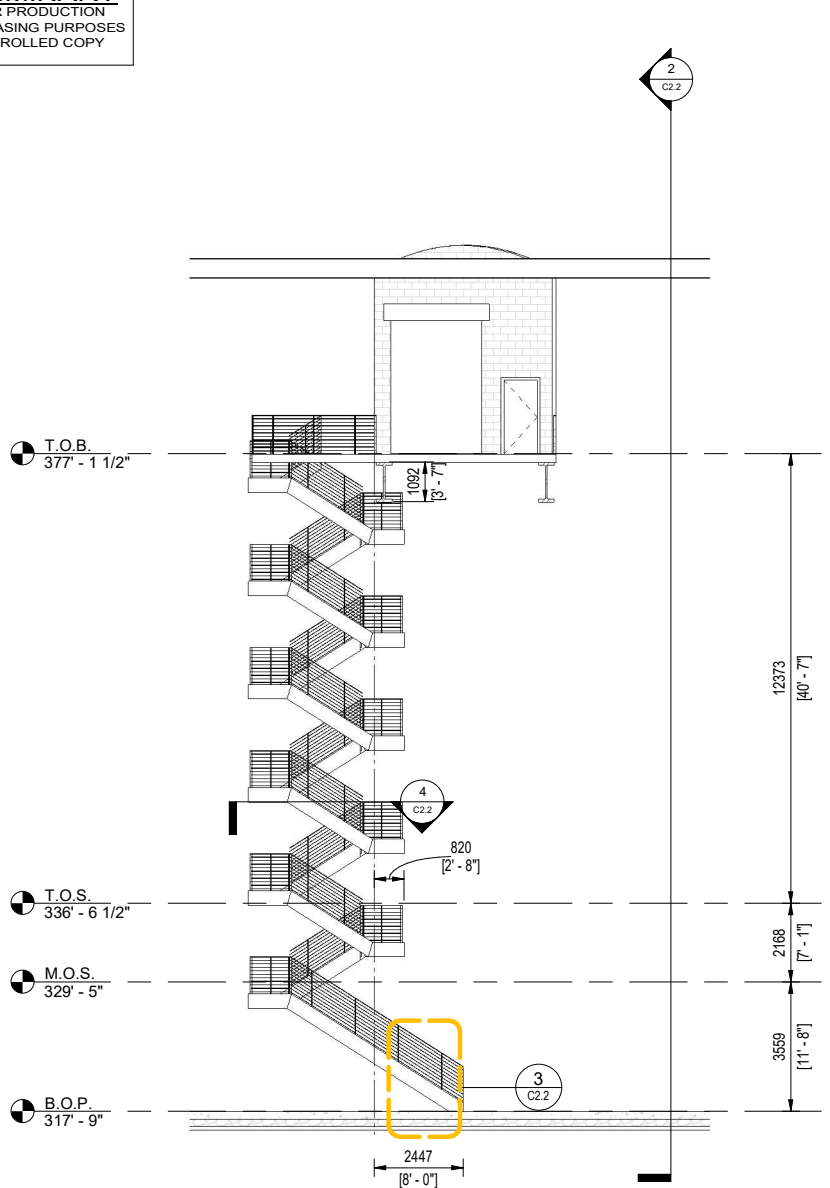
1 BRIDGE // STAIR SECTION 1:100
