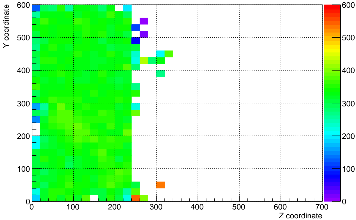
plane_0 (beam left) dQ/dx for YZ plane for time 15 hrs to 16 hrs
