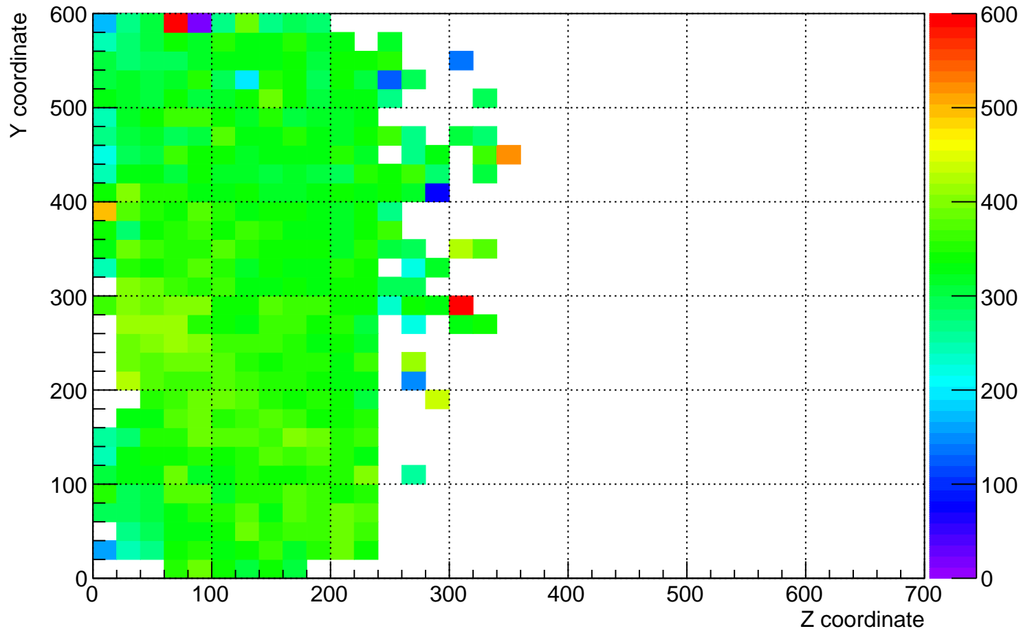
plane_0 (beam left) dQ/dx for YZ plane for time 2 hrs to 3 hrs
