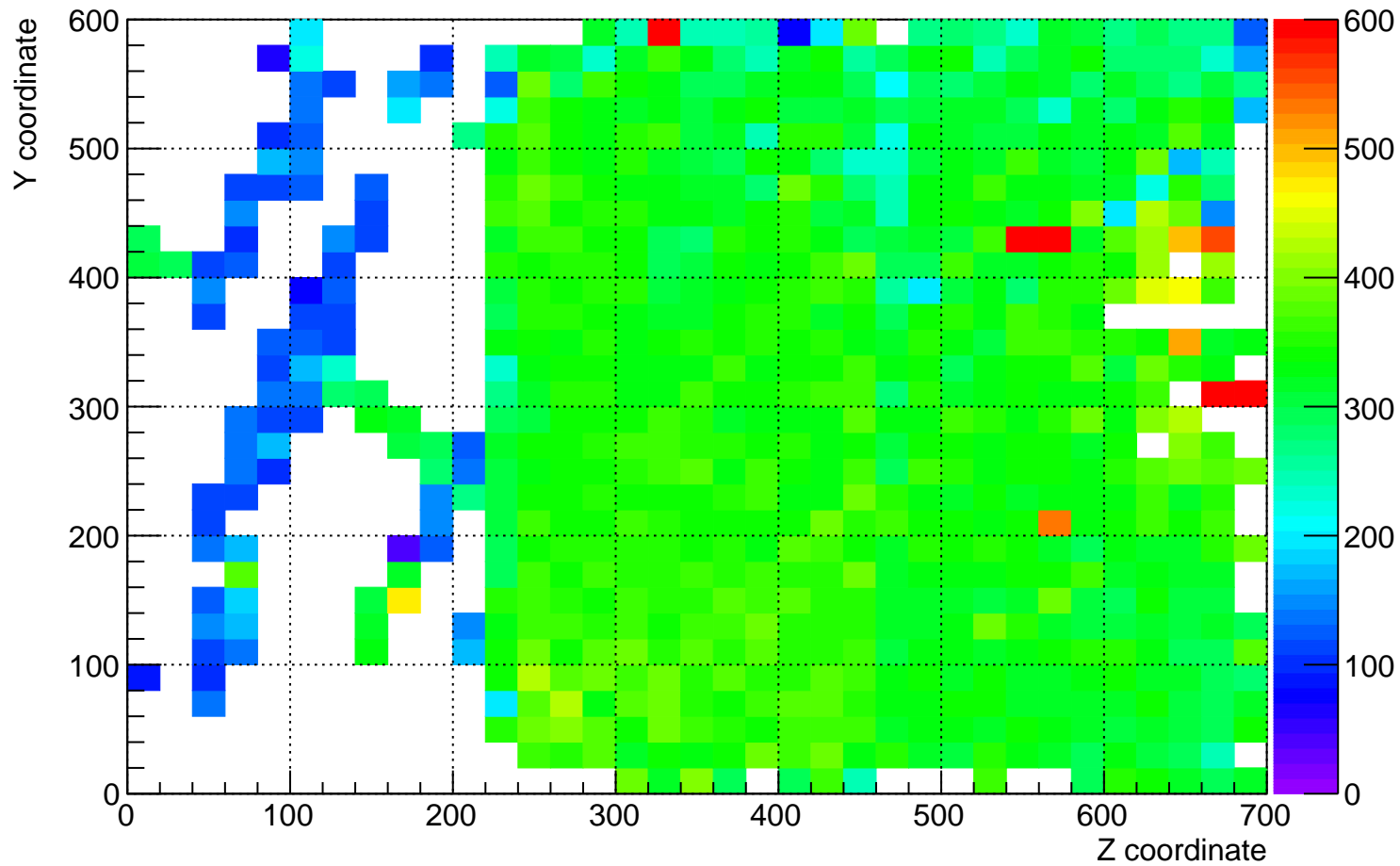
plane_0 (beam right) dQ/dx for YZ plane for time 2 hrs to 3 hrs
