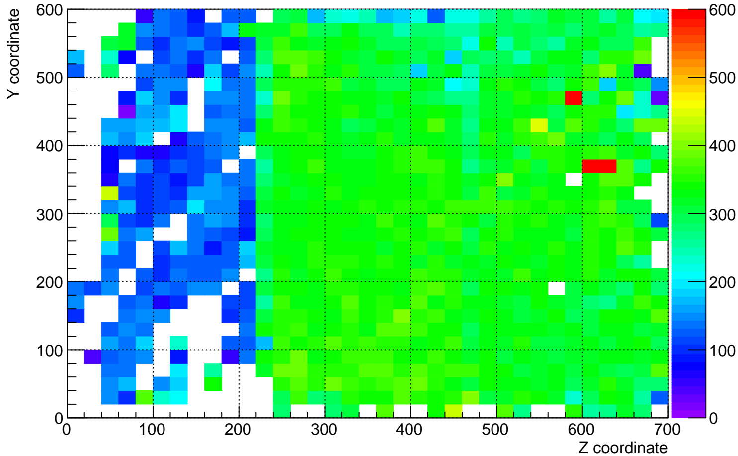
plane_0 (beam right) dQ/dx for YZ plane for time 6 hrs to 7 hrs
