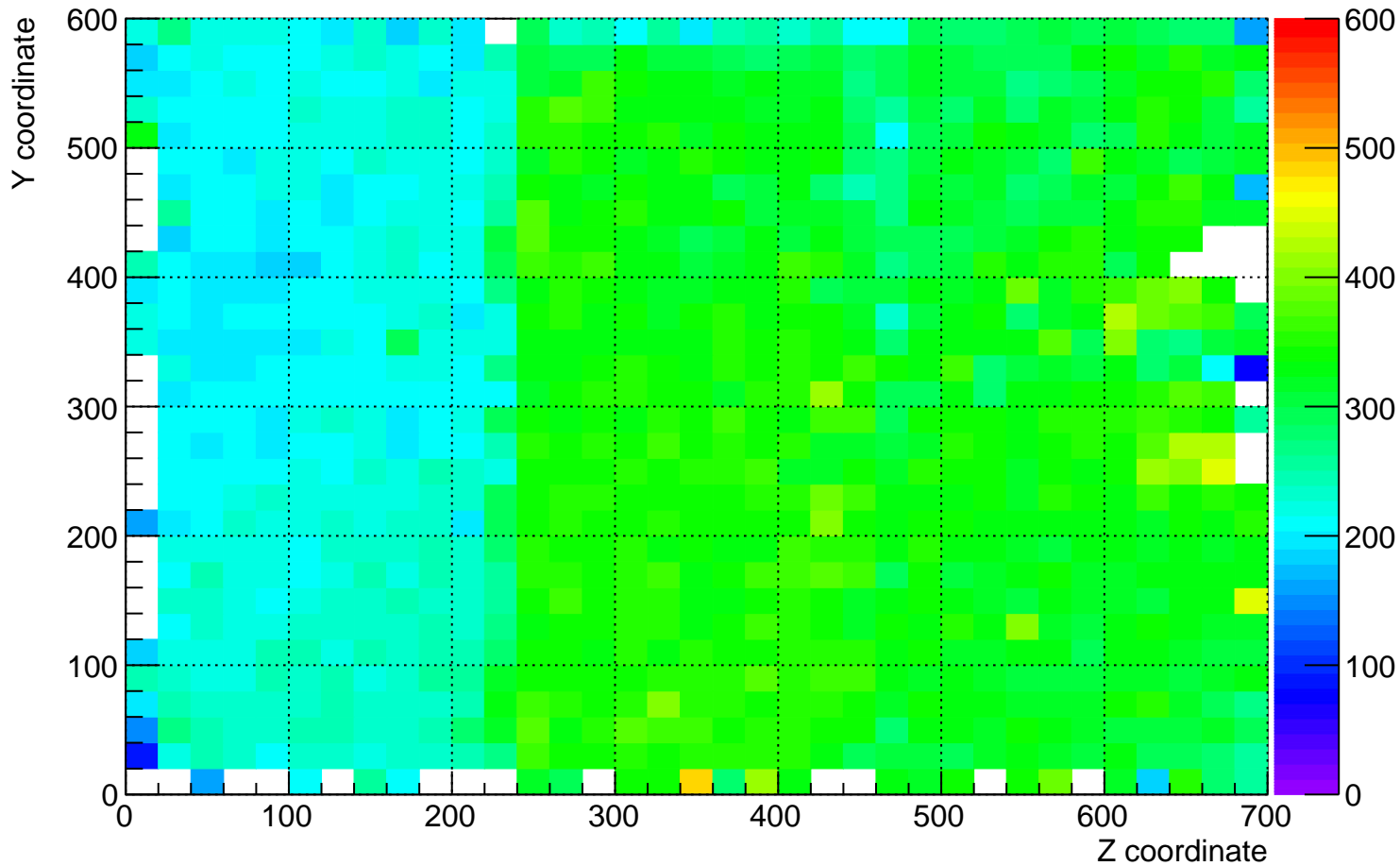
plane_0 (beam right) dQ/dx for YZ plane for time 16 hrs to 17 hrs
