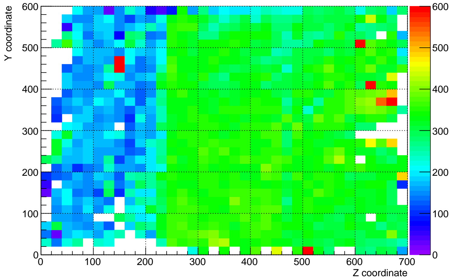
plane_0 (beam right) dQ/dx for YZ plane for time 9 hrs to 10 hrs
