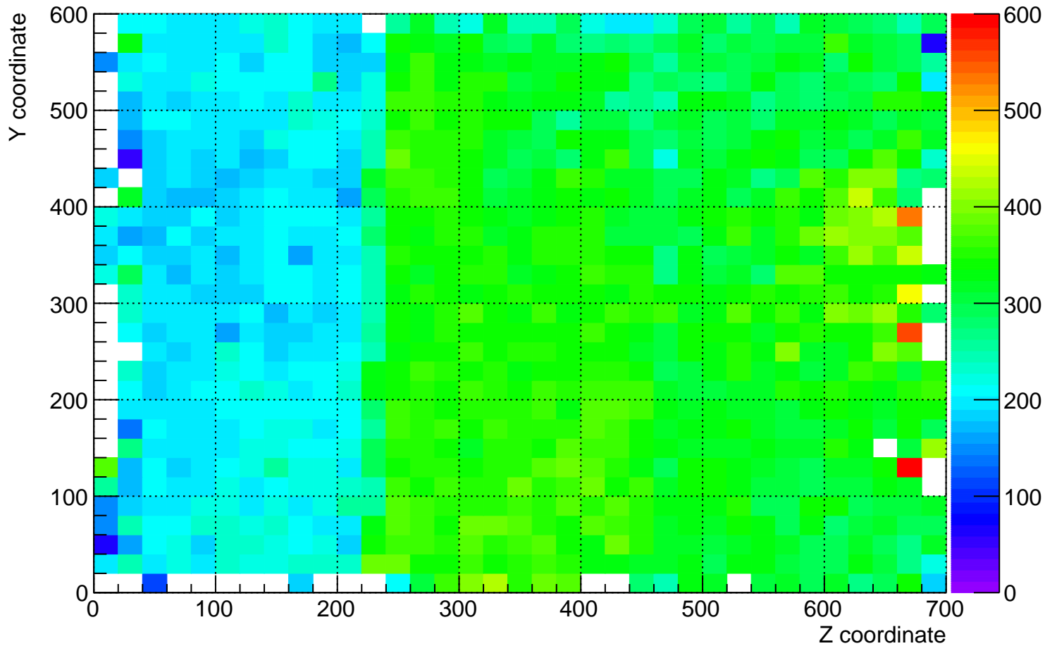
plane_0 (beam right) dQ/dx for YZ plane for time 13 hrs to 14 hrs
