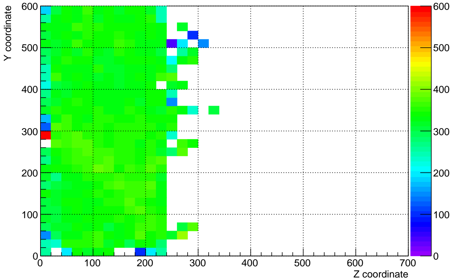
plane_0 (beam left) dQ/dx for YZ plane for time 16 hrs to 17 hrs
