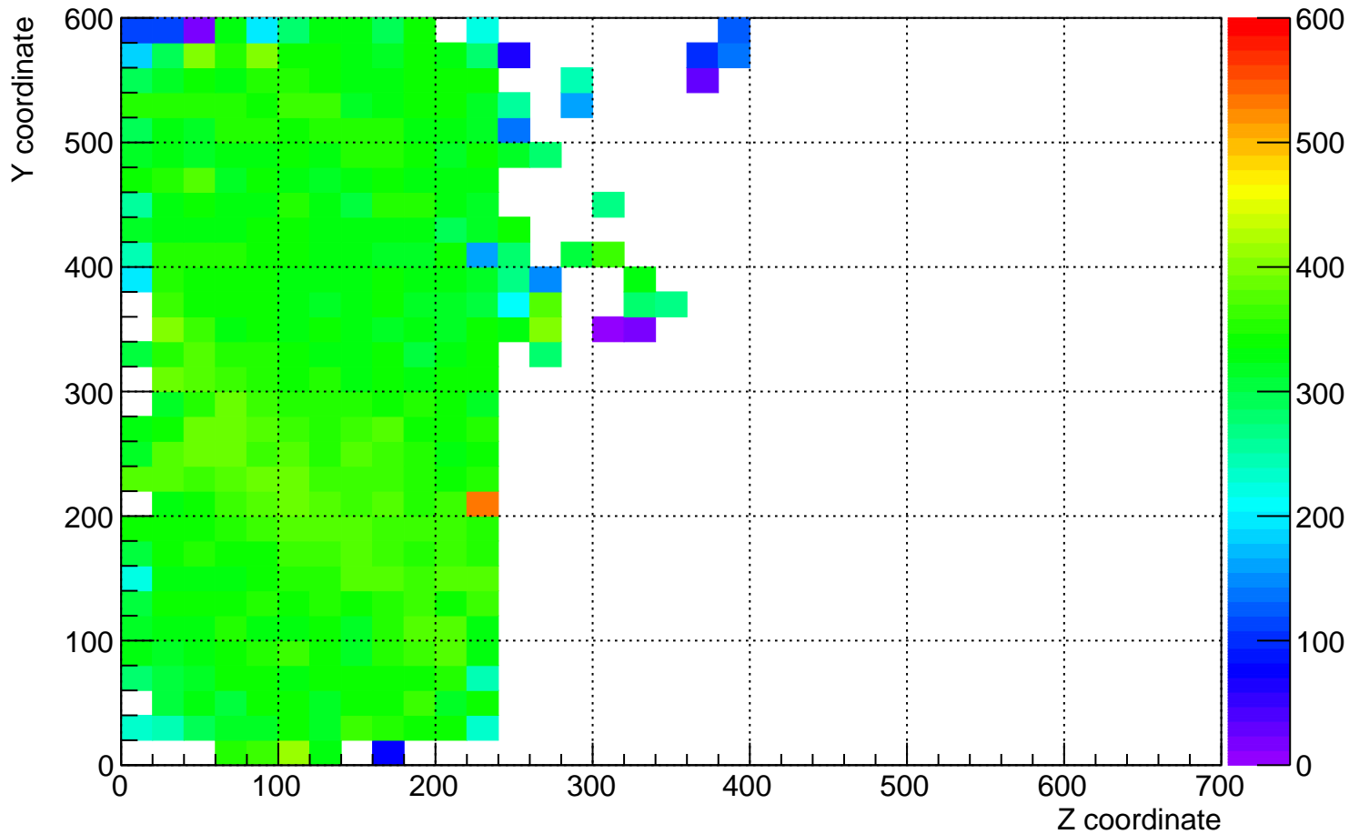
plane_0 (beam left) dQ/dx for YZ plane for time 9 hrs to 10 hrs
