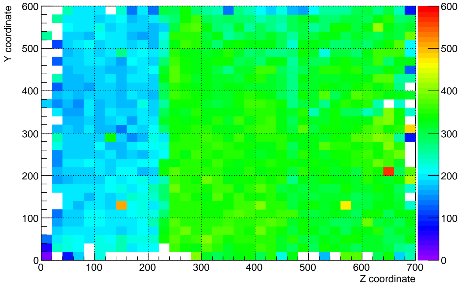
plane_0 (beam right) dQ/dx for YZ plane for time 12 hrs to 13 hrs
