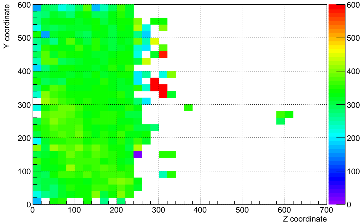
plane_0 (beam left) dQ/dx for YZ plane for time 0 hrs to 1 hrs
