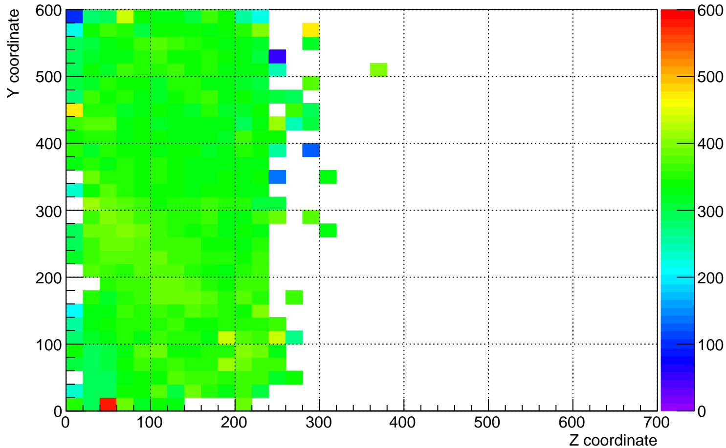
plane_0 (beam left) dQ/dx for YZ plane for time 7 hrs to 8 hrs
