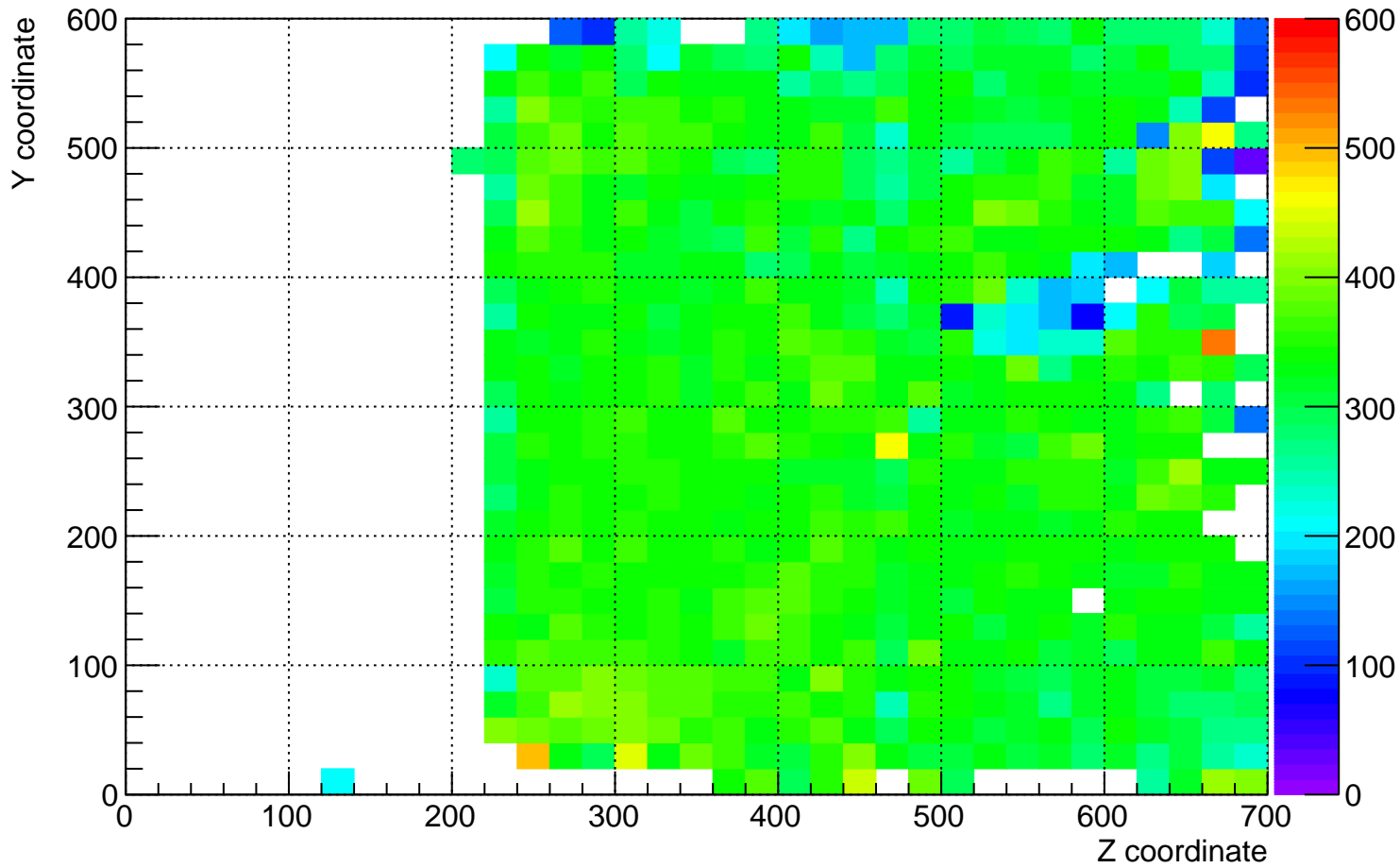
plane_0 (beam right) dQ/dx for YZ plane for time 1 hrs to 2 hrs
