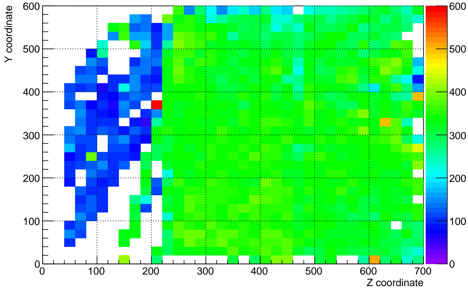
plane_0 (beam right) dQ/dx for YZ plane for time 3 hrs to 4 hrs
