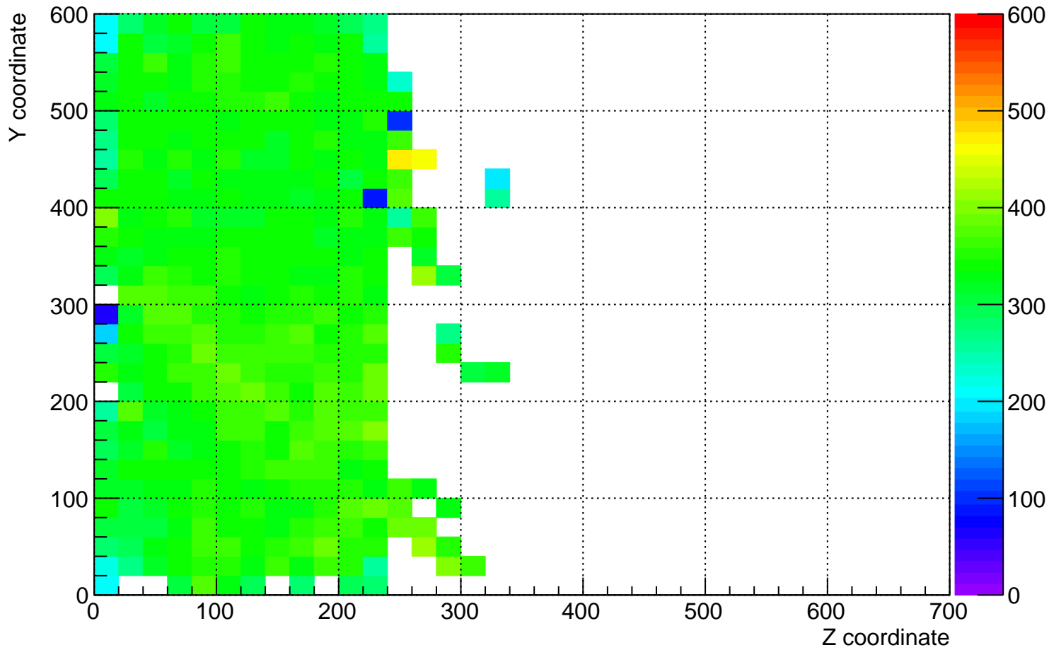
plane_0 (beam left) dQ/dx for YZ plane for time 13 hrs to 14 hrs
