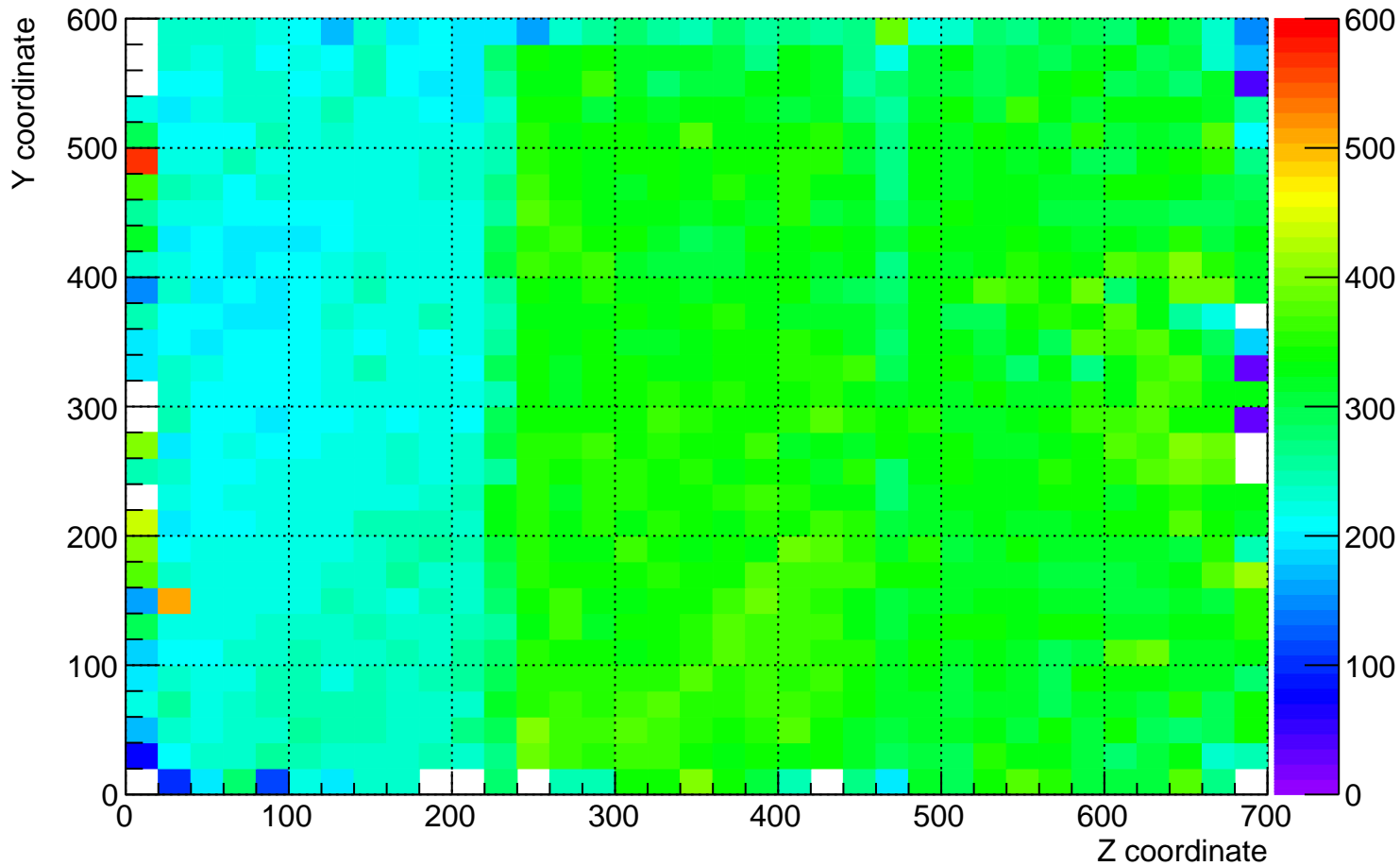
plane_0 (beam right) dQ/dx for YZ plane for time 17 hrs to 18 hrs
