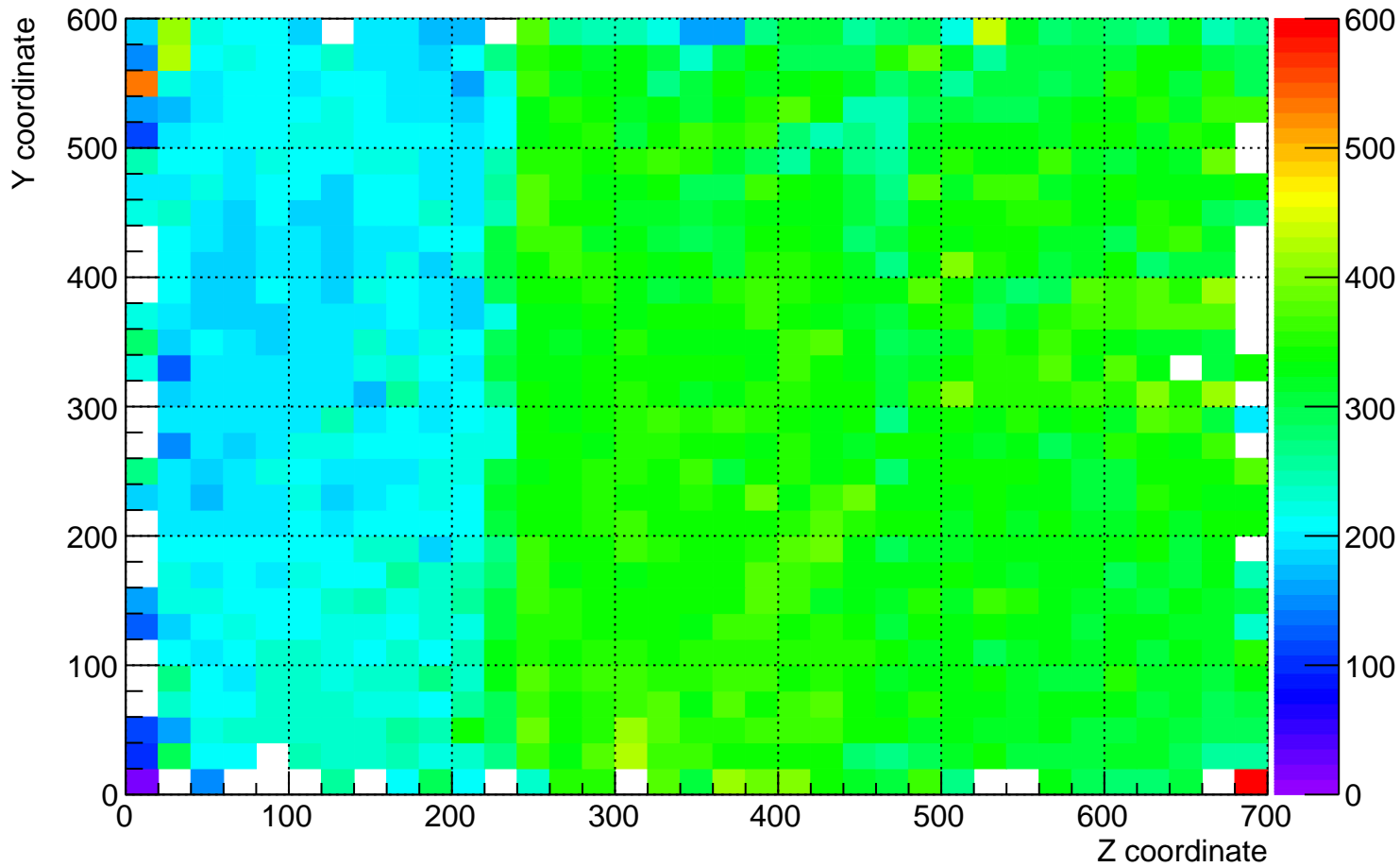
plane_0 (beam right) dQ/dx for YZ plane for time 14 hrs to 15 hrs
