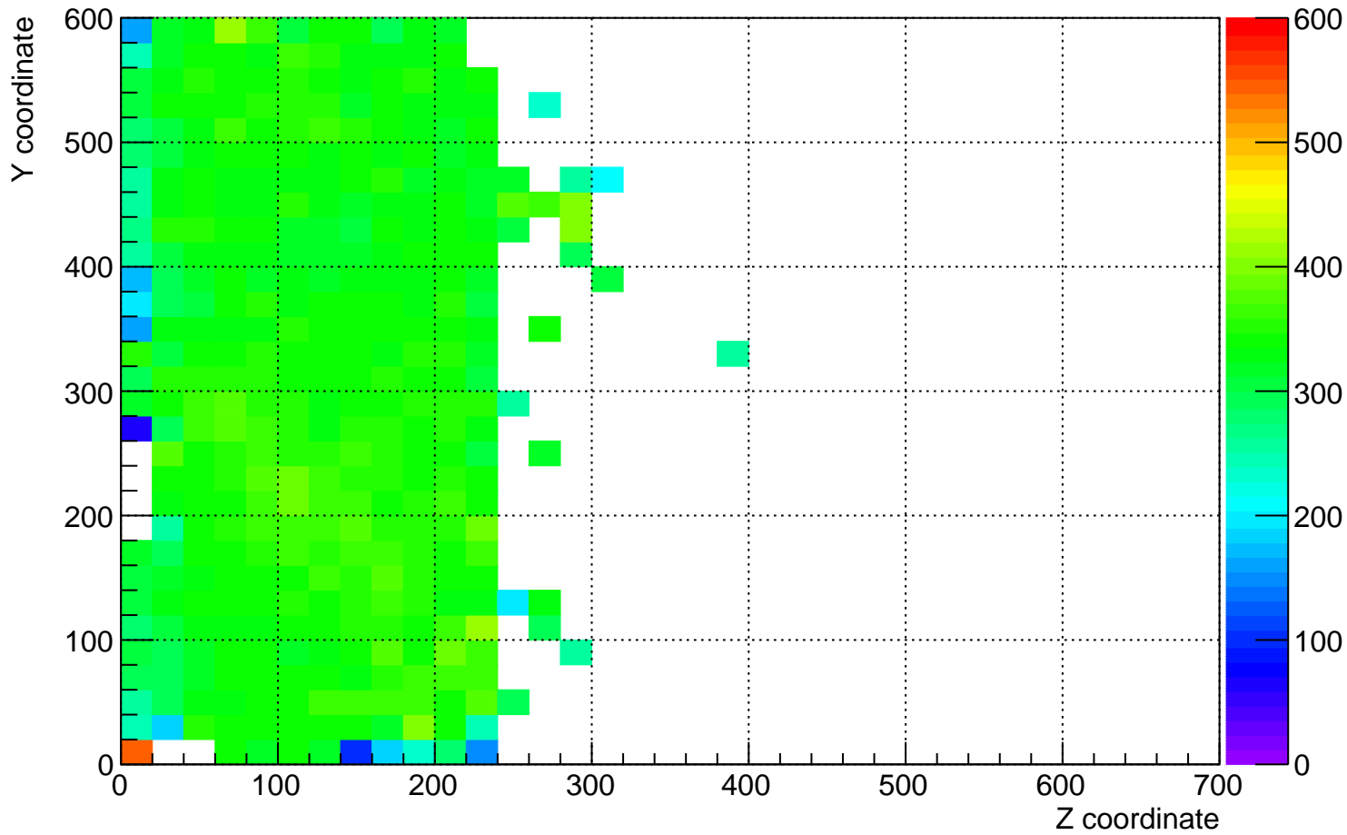
plane_0 (beam left) dQ/dx for YZ plane for time 14 hrs to 15 hrs
