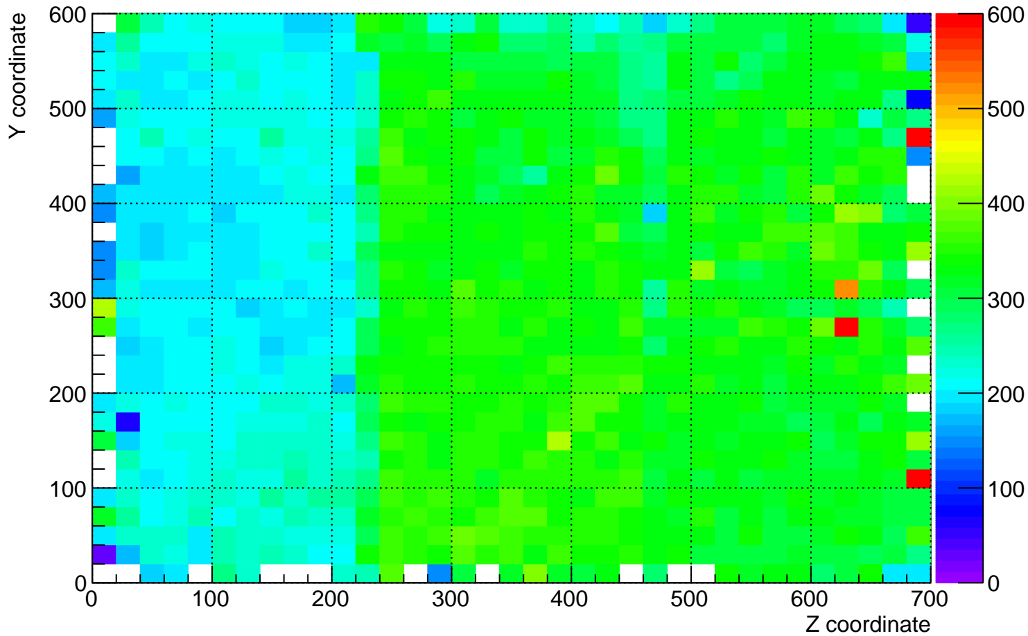
plane_0 (beam right) dQ/dx for YZ plane for time 15 hrs to 16 hrs
