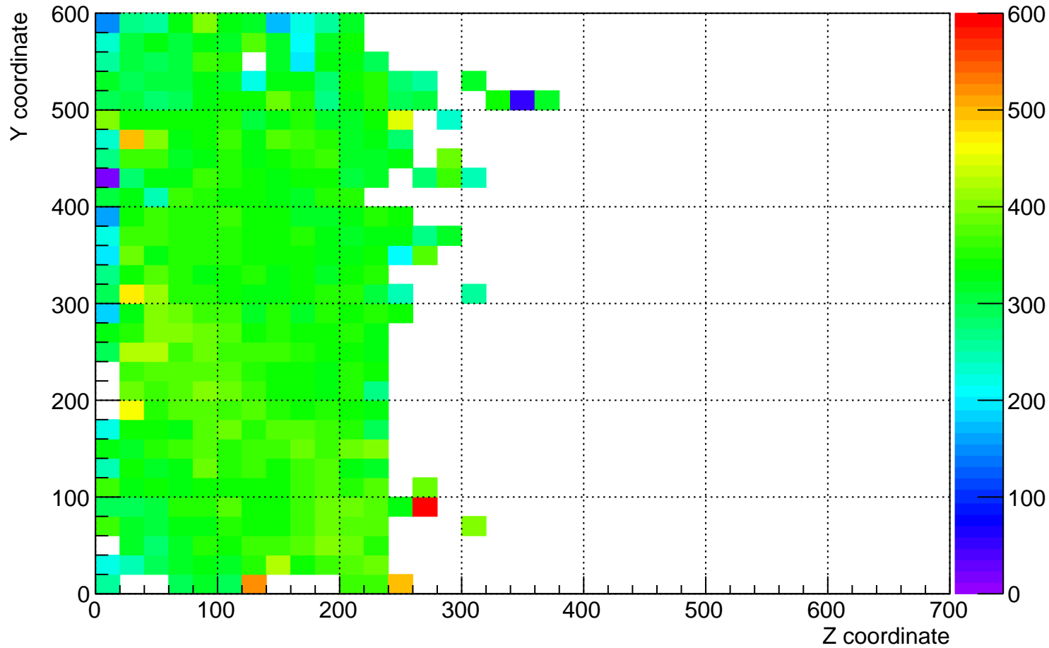
plane_0 (beam left) dQ/dx for YZ plane for time 1 hrs to 2 hrs
