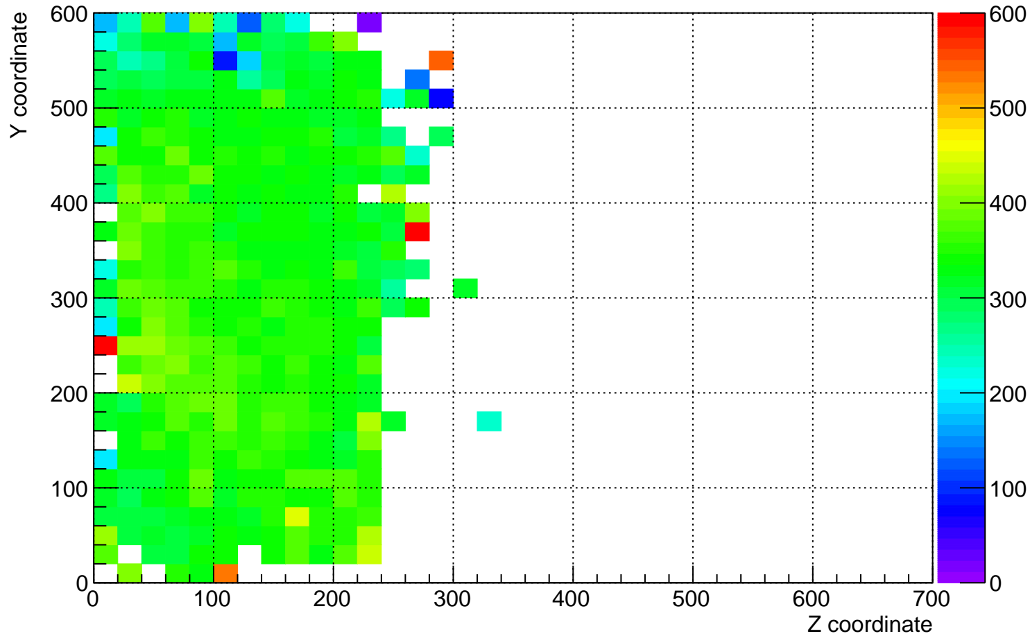
plane_0 (beam left) dQ/dx for YZ plane for time 4 hrs to 5 hrs
