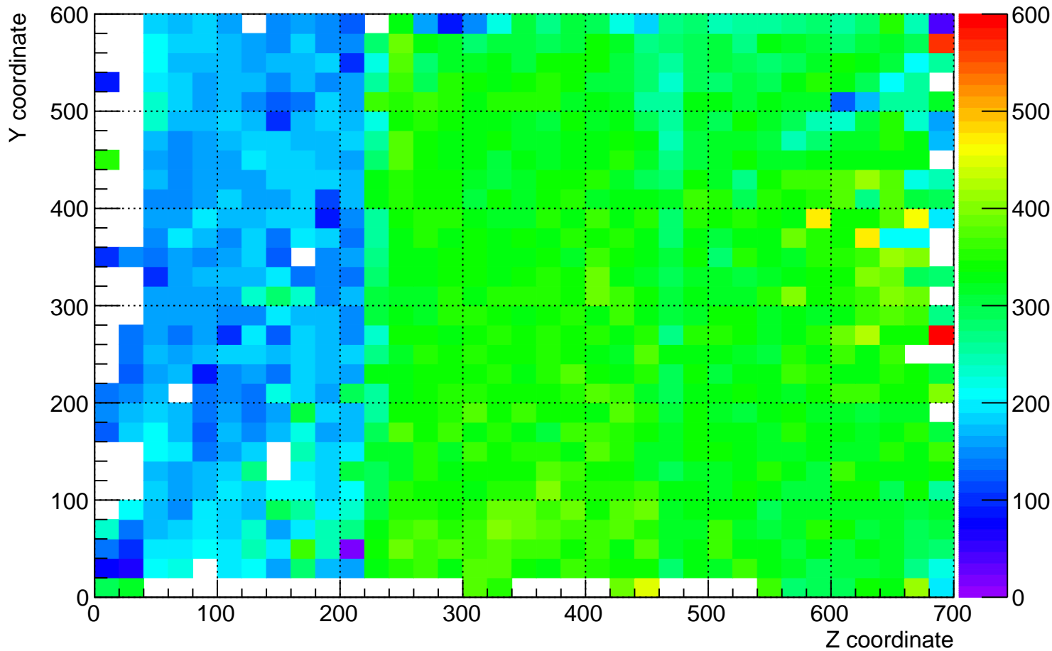
plane_0 (beam right) dQ/dx for YZ plane for time 10 hrs to 11 hrs
