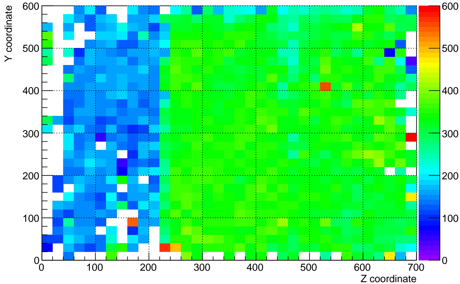
plane_0 (beam right) dQ/dx for YZ plane for time 8 hrs to 9 hrs
