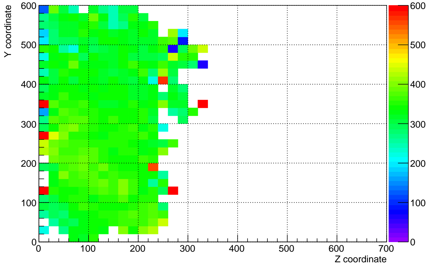
plane_0 (beam left) dQ/dx for YZ plane for time 3 hrs to 4 hrs
