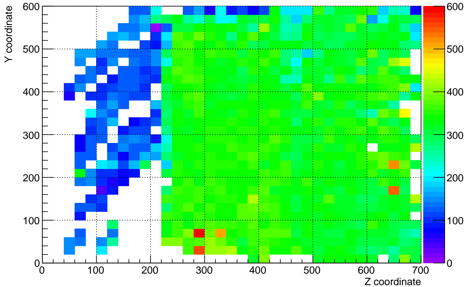
plane_0 (beam right) dQ/dx for YZ plane for time 4 hrs to 5 hrs
