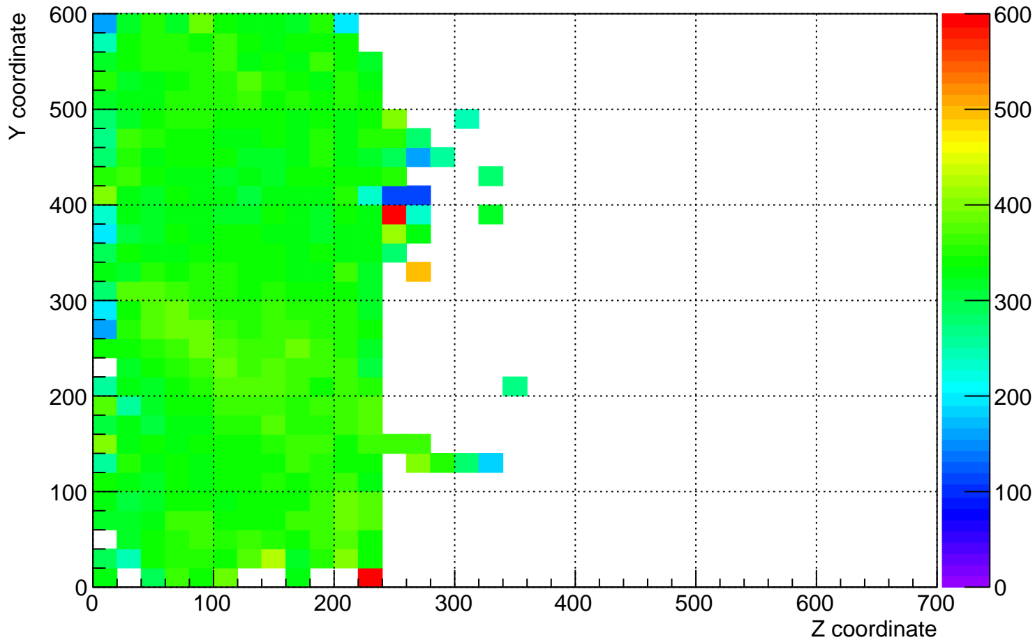
plane_0 (beam left) dQ/dx for YZ plane for time 12 hrs to 13 hrs
