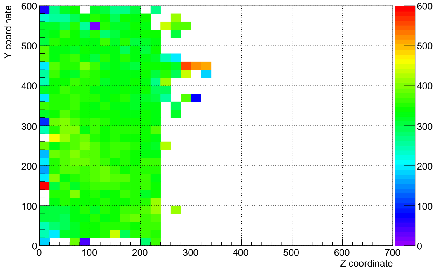
plane_0 (beam left) dQ/dx for YZ plane for time 5 hrs to 6 hrs
