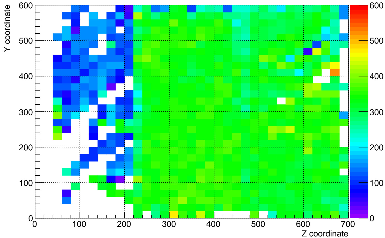
plane_0 (beam right) dQ/dx for YZ plane for time 5 hrs to 6 hrs
