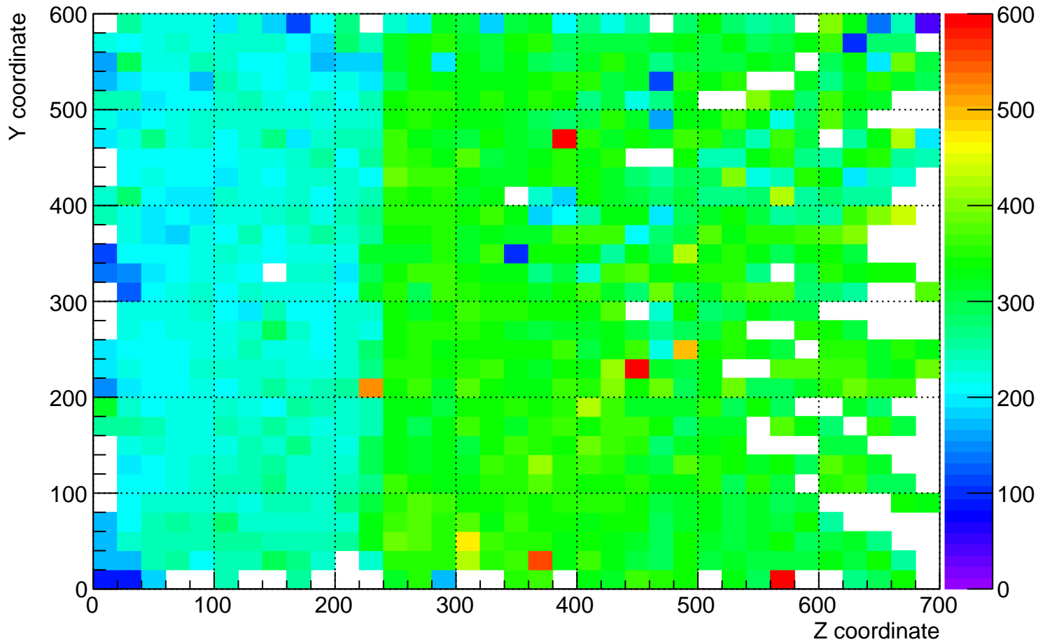
plane_0 (beam right) dQ/dx for YZ plane for time 18 hrs to 19 hrs
