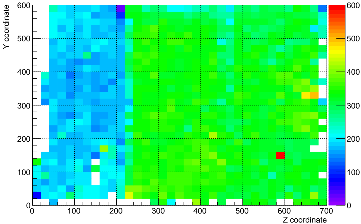
plane_0 (beam right) dQ/dx for YZ plane for time 11 hrs to 12 hrs
