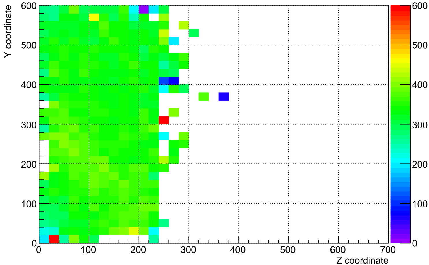
plane_0 (beam left) dQ/dx for YZ plane for time 6 hrs to 7 hrs
