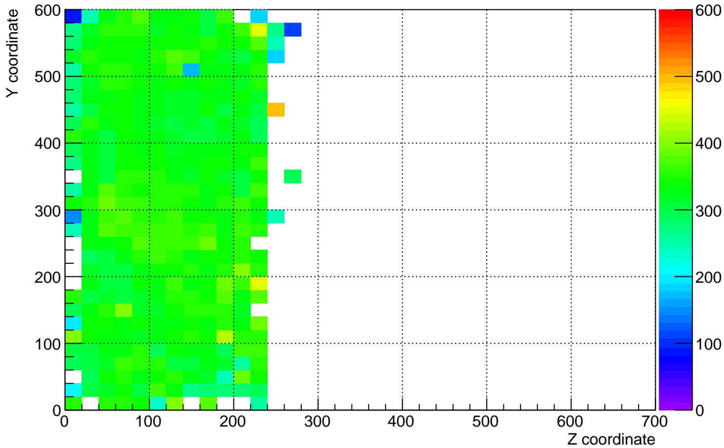
plane_0 (beam left) dQ/dx for YZ plane for time 18 hrs to 19 hrs
