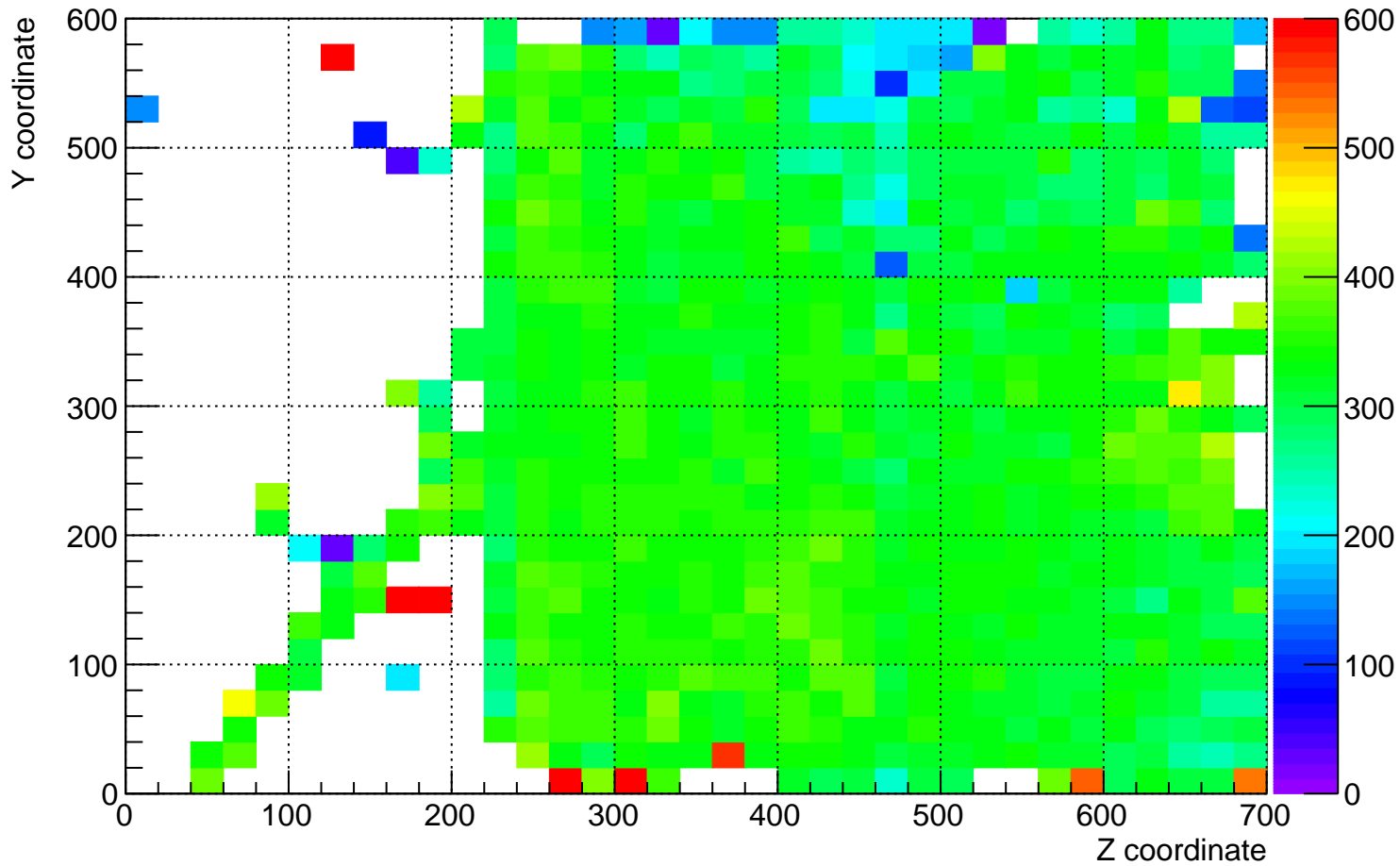
plane_0 (beam right) dQ/dx for YZ plane for time 0 hrs to 1 hrs
