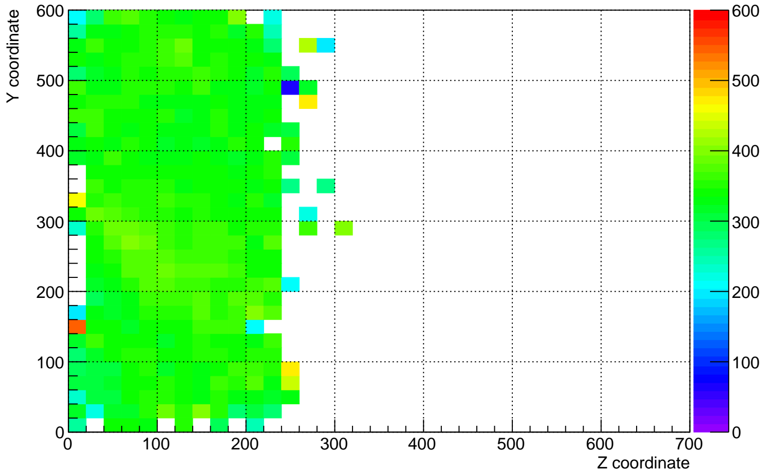
plane_0 (beam left) dQ/dx for YZ plane for time 10 hrs to 11 hrs
