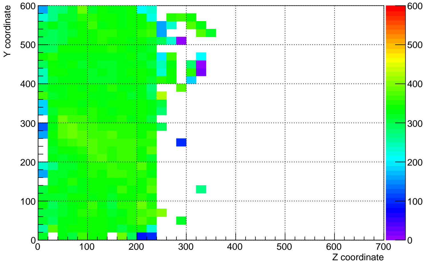
plane_0 (beam left) dQ/dx for YZ plane for time 17 hrs to 18 hrs
