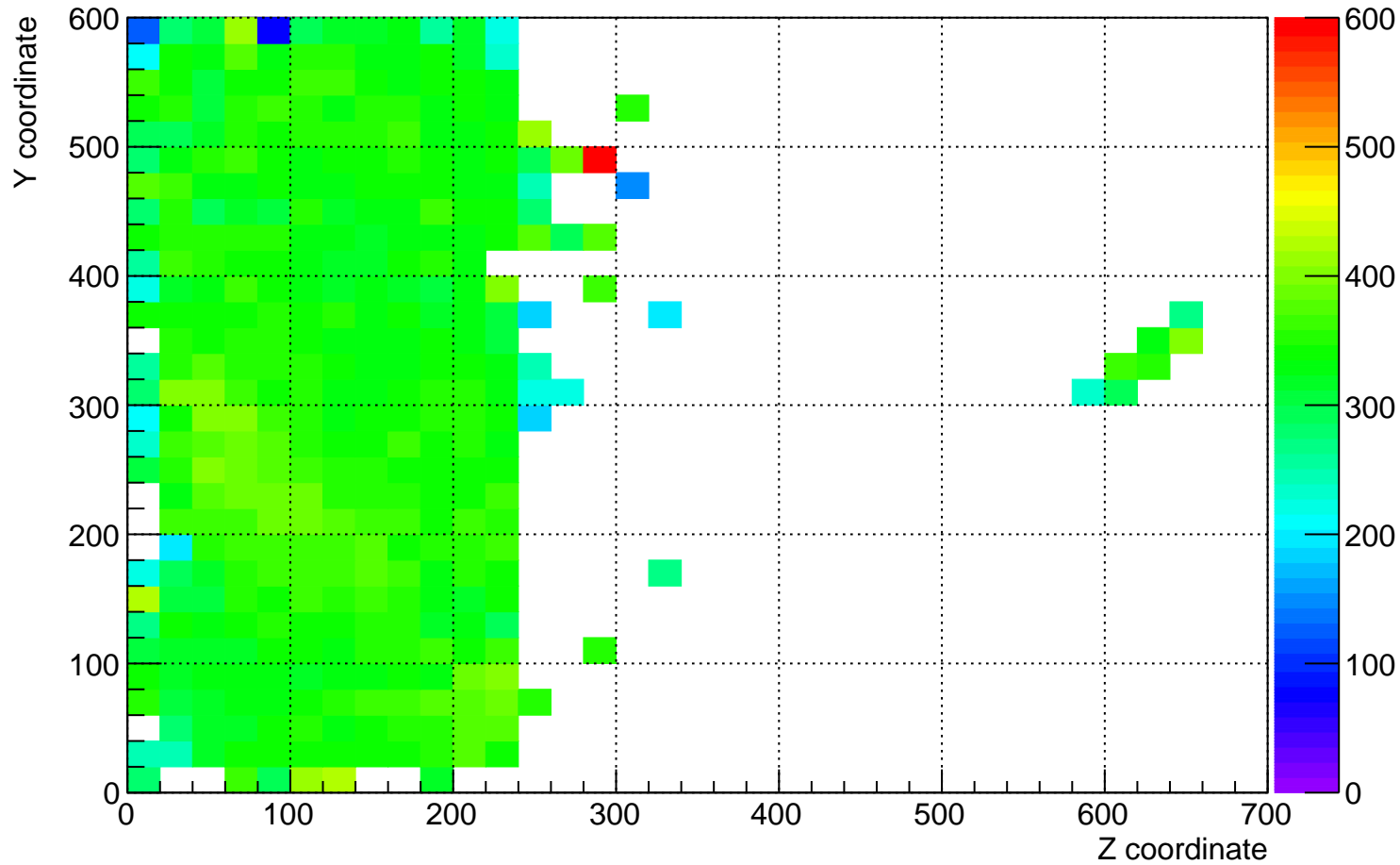
plane_0 (beam left) dQ/dx for YZ plane for time 8 hrs to 9 hrs
