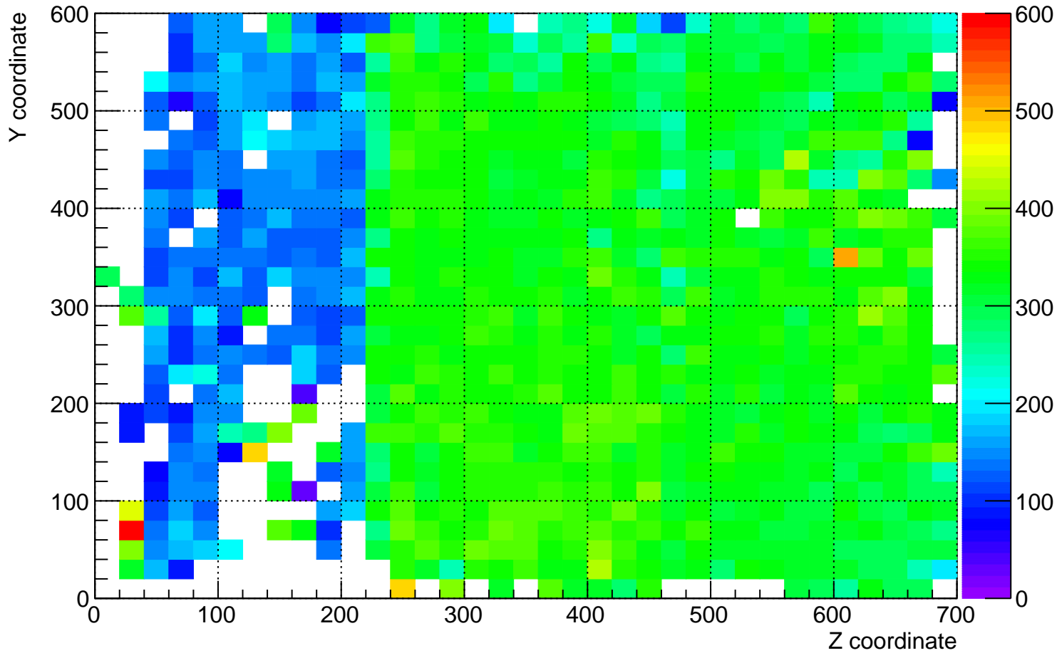
plane_0 (beam right) dQ/dx for YZ plane for time 7 hrs to 8 hrs
