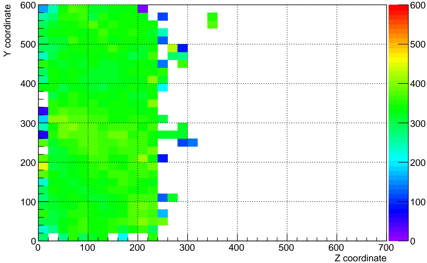
plane_0 (beam left) dQ/dx for YZ plane for time 11 hrs to 12 hrs
