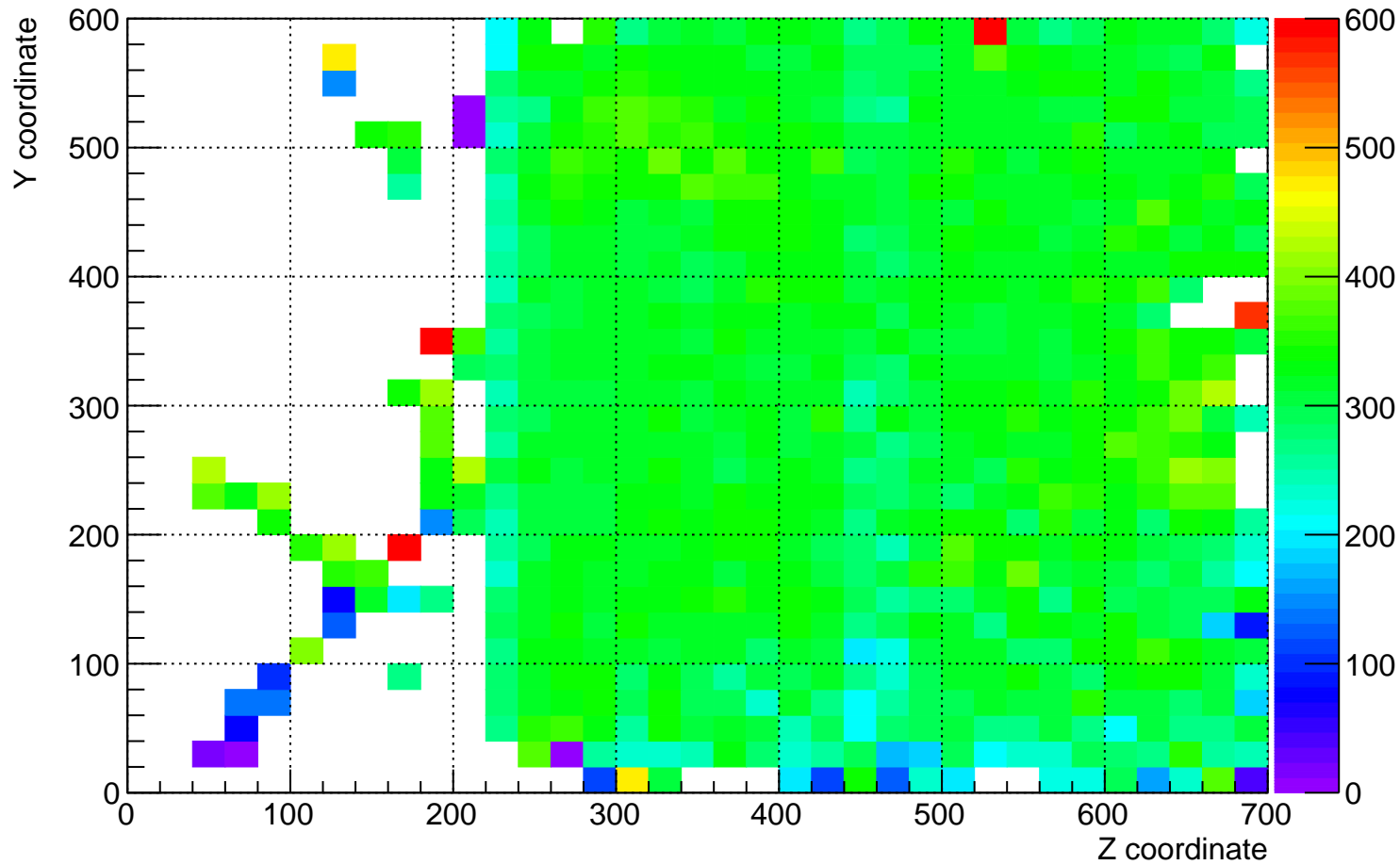
plane_1 (beam right) dQ/dx for YZ plane for time 0 hrs to 1 hrs
