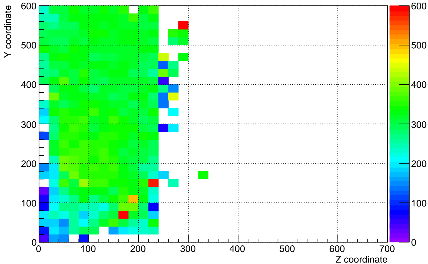
plane_1 (beam left) dQ/dx for YZ plane for time 4 hrs to 5 hrs
