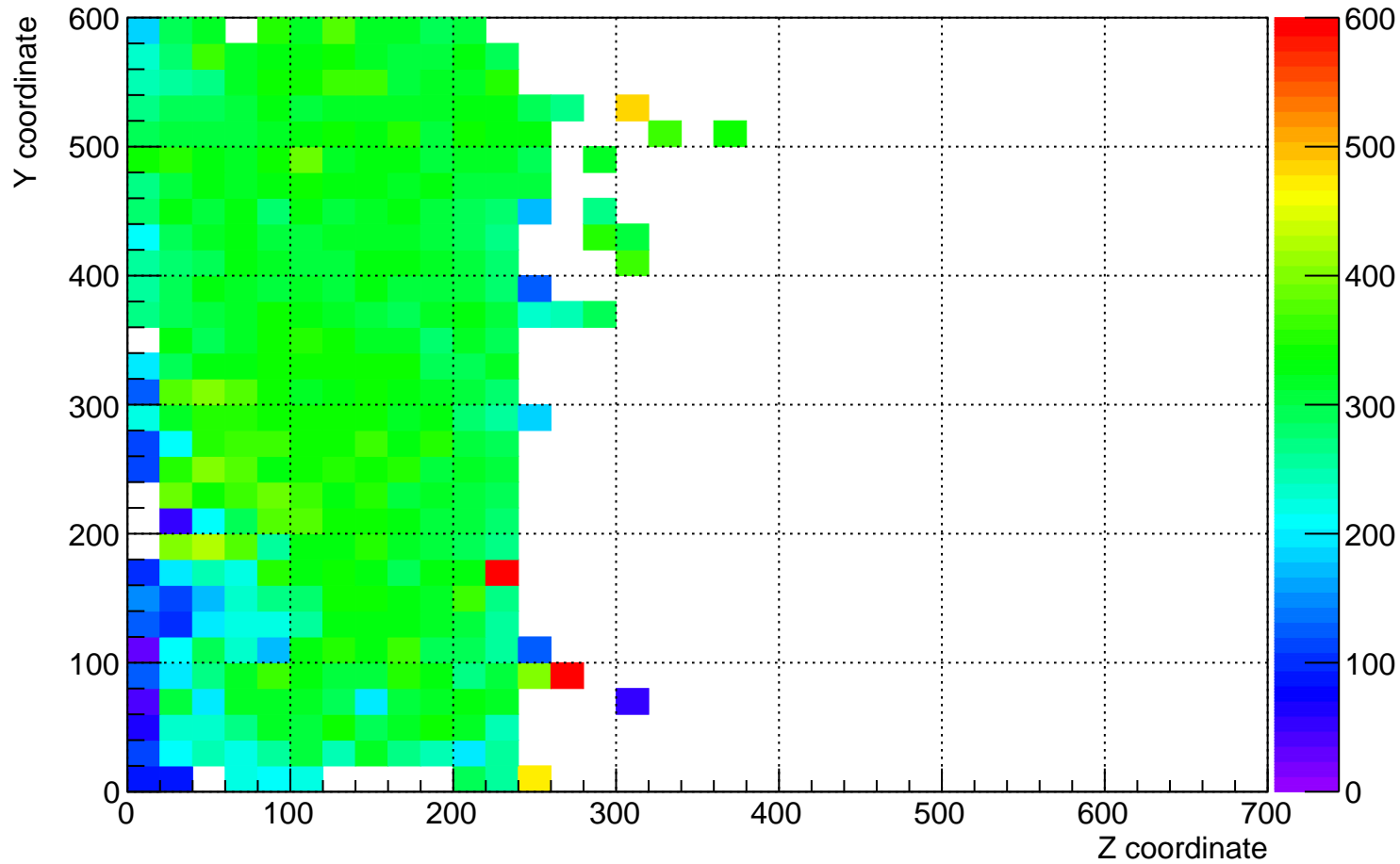
plane_1 (beam left) dQ/dx for YZ plane for time 1 hrs to 2 hrs
