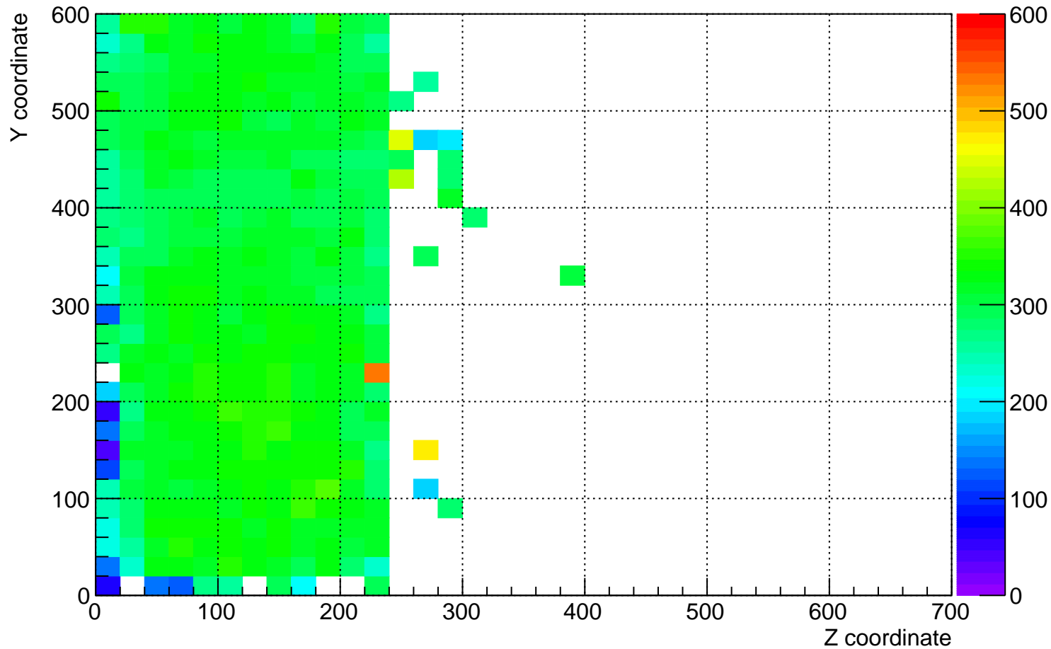
plane_1 (beam left) dQ/dx for YZ plane for time 14 hrs to 15 hrs
