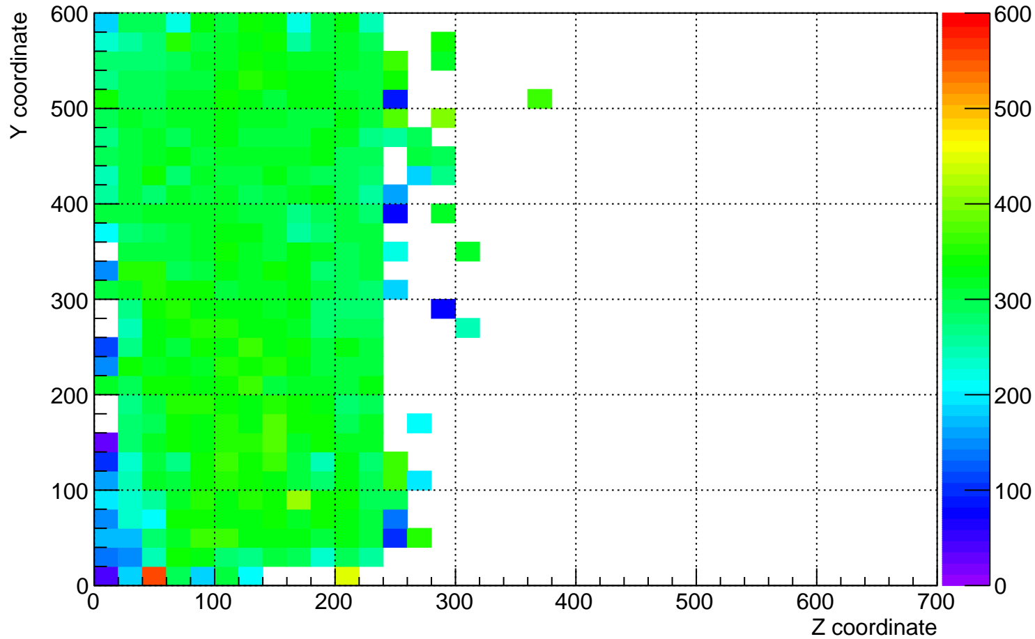
plane_1 (beam left) dQ/dx for YZ plane for time 7 hrs to 8 hrs
