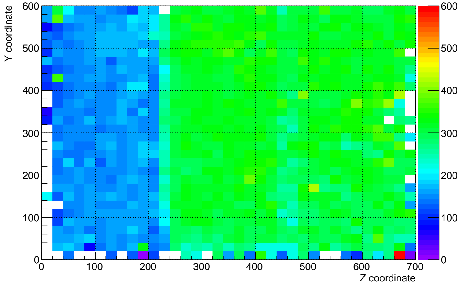
plane_1 (beam right) dQ/dx for YZ plane for time 14 hrs to 15 hrs
