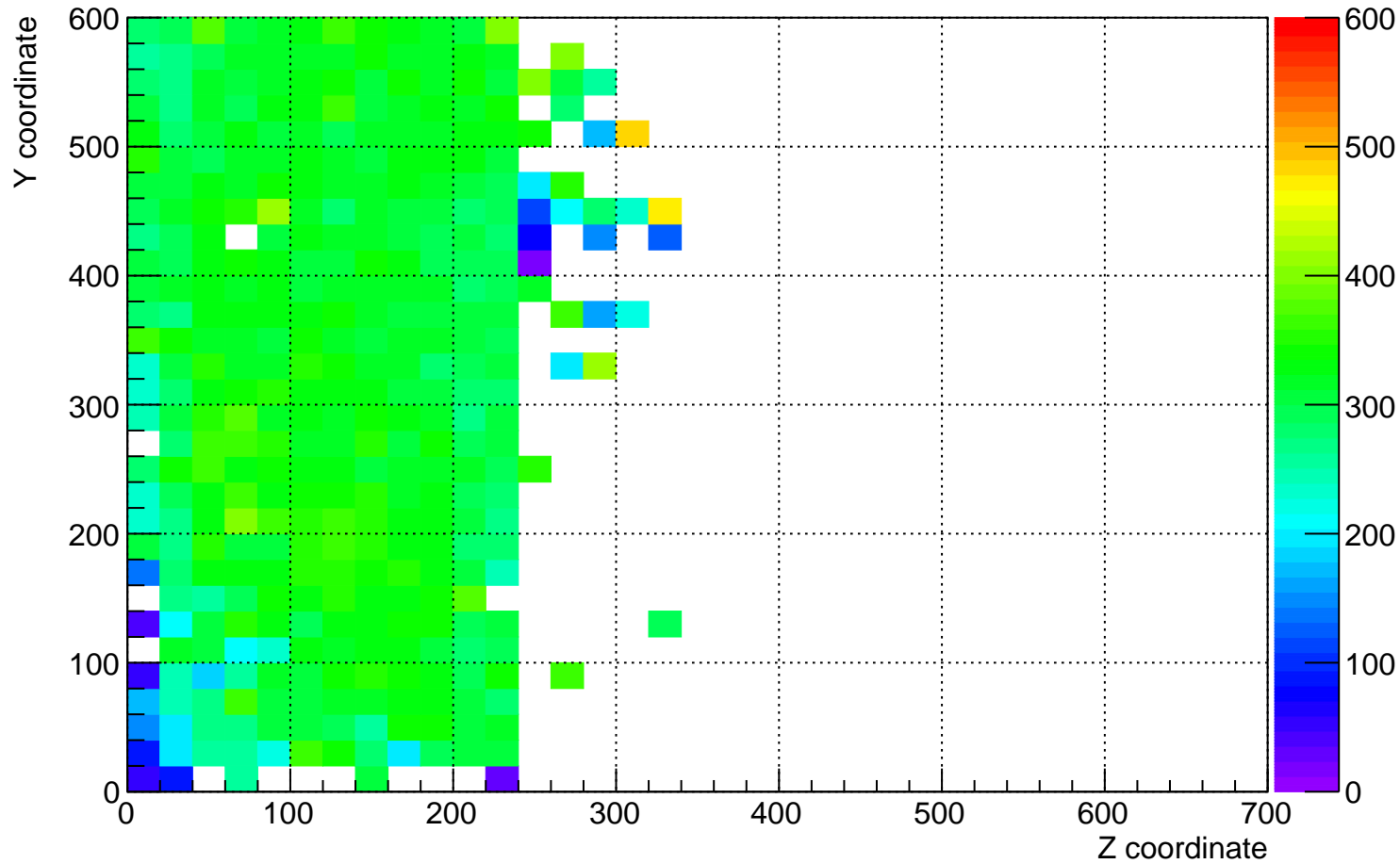
plane_1 (beam left) dQ/dx for YZ plane for time 5 hrs to 6 hrs
