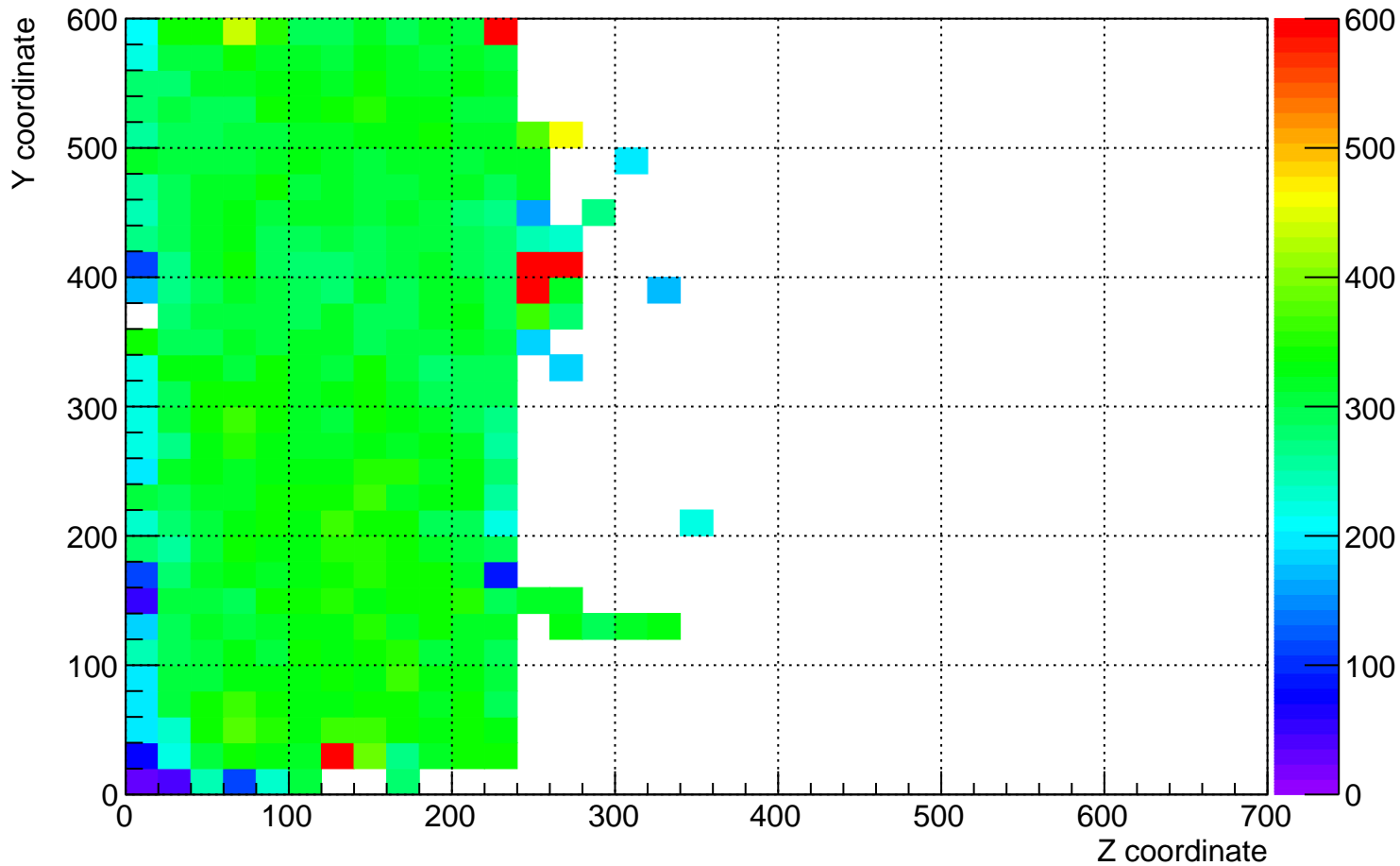
plane_1 (beam left) dQ/dx for YZ plane for time 12 hrs to 13 hrs
