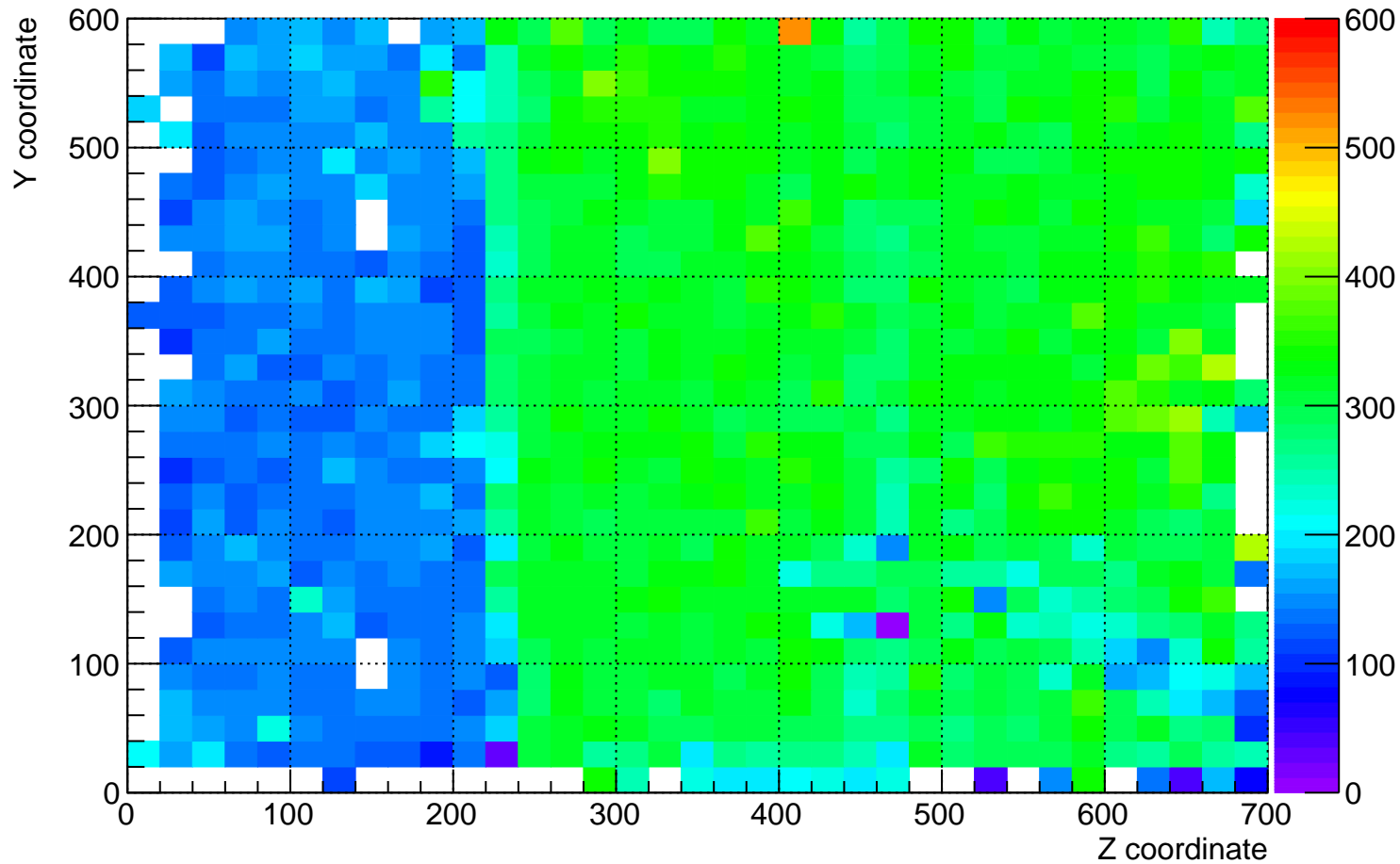
plane_1 (beam right) dQ/dx for YZ plane for time 12 hrs to 13 hrs
