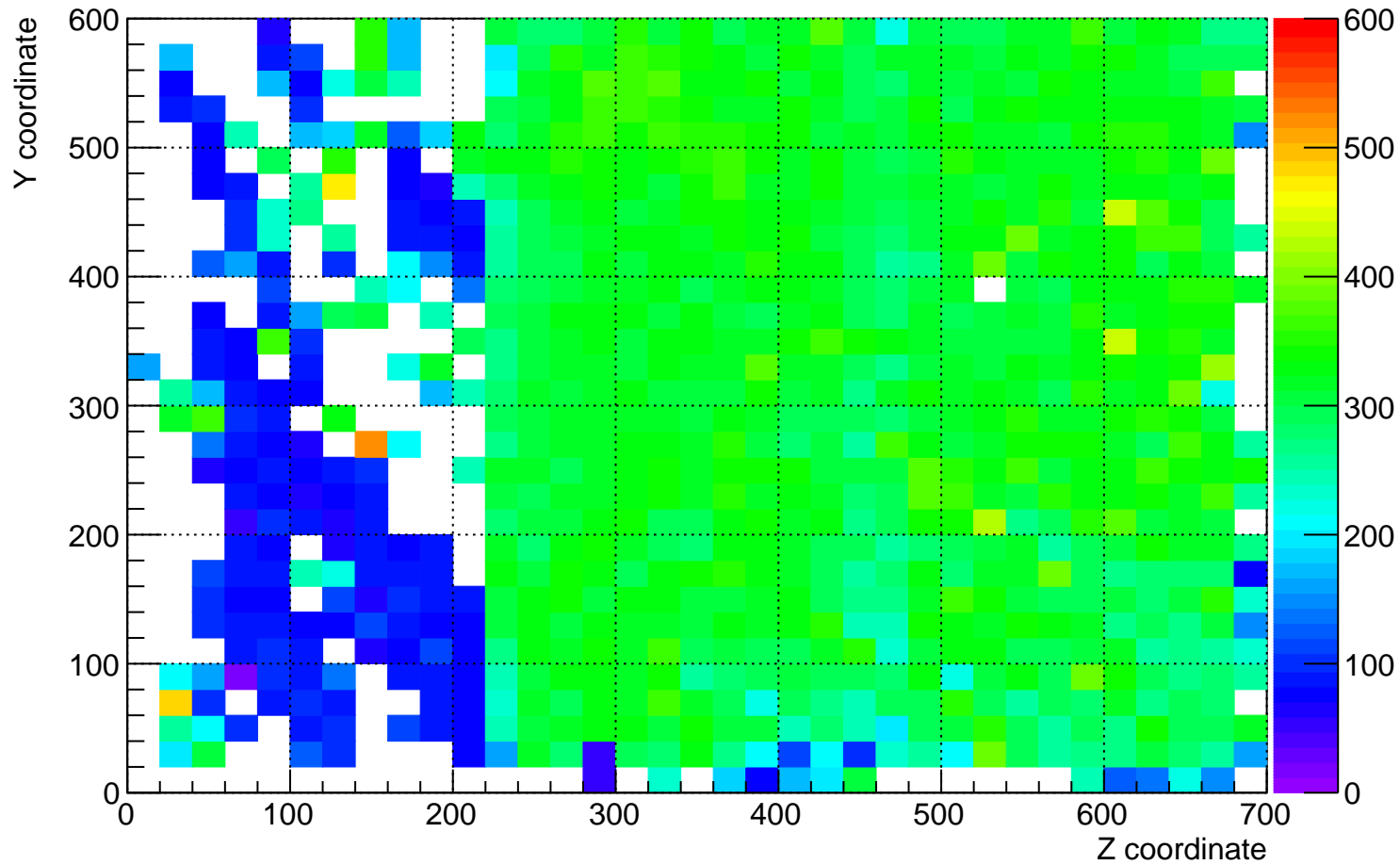
plane_1 (beam right) dQ/dx for YZ plane for time 7 hrs to 8 hrs
