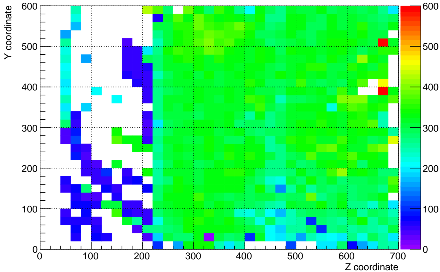
plane_1 (beam right) dQ/dx for YZ plane for time 5 hrs to 6 hrs
