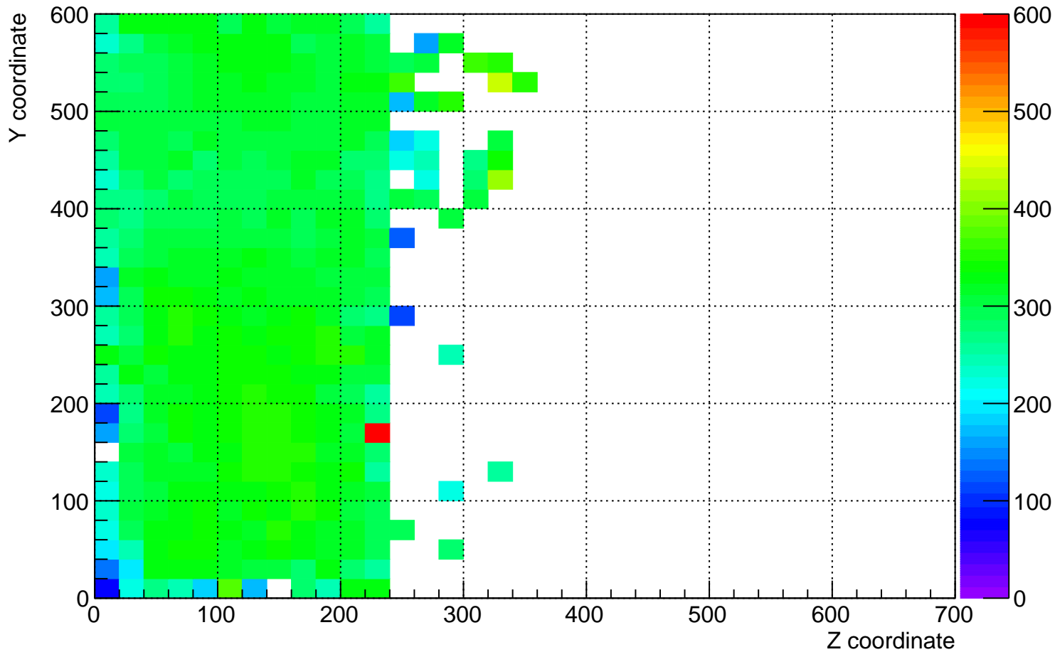
plane_1 (beam left) dQ/dx for YZ plane for time 17 hrs to 18 hrs
