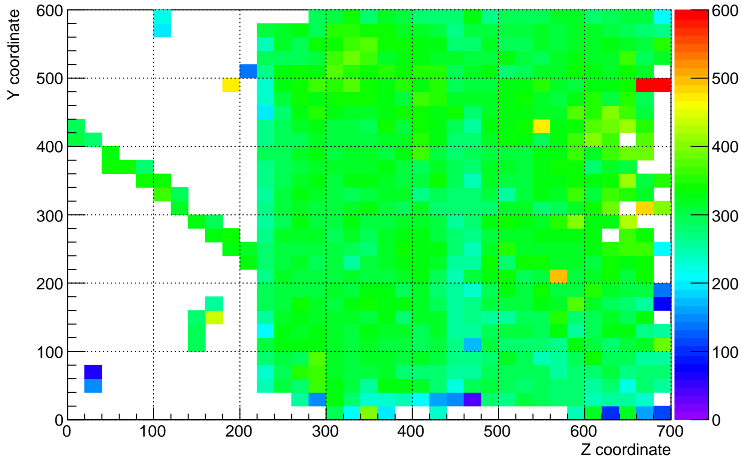
plane_1 (beam right) dQ/dx for YZ plane for time 2 hrs to 3 hrs
