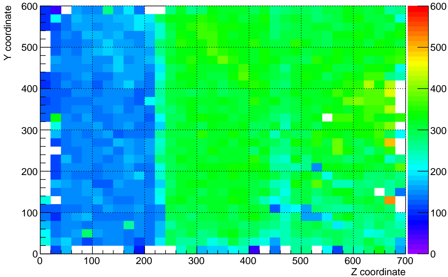
plane_1 (beam right) dQ/dx for YZ plane for time 13 hrs to 14 hrs
