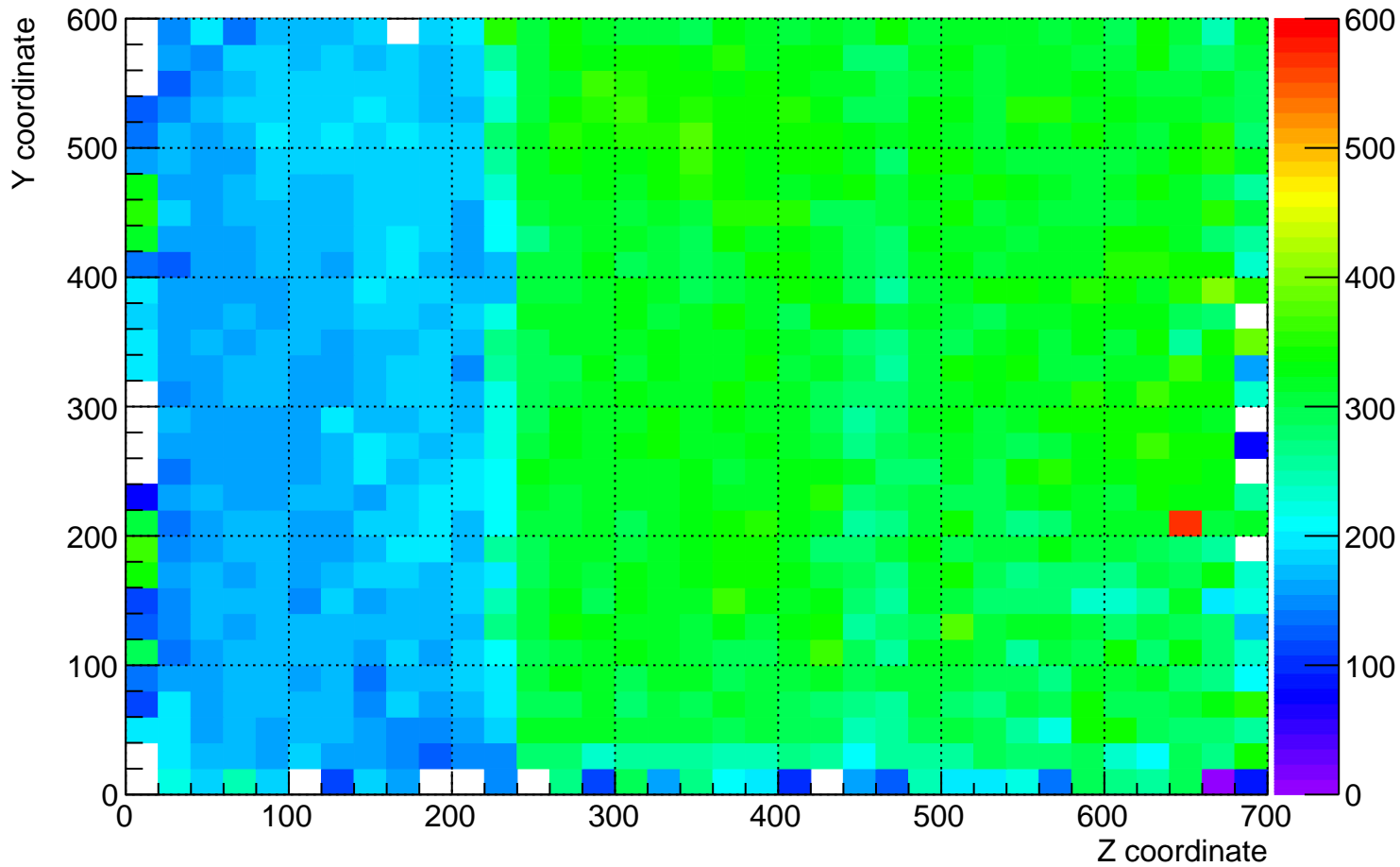
plane_1 (beam right) dQ/dx for YZ plane for time 17 hrs to 18 hrs
