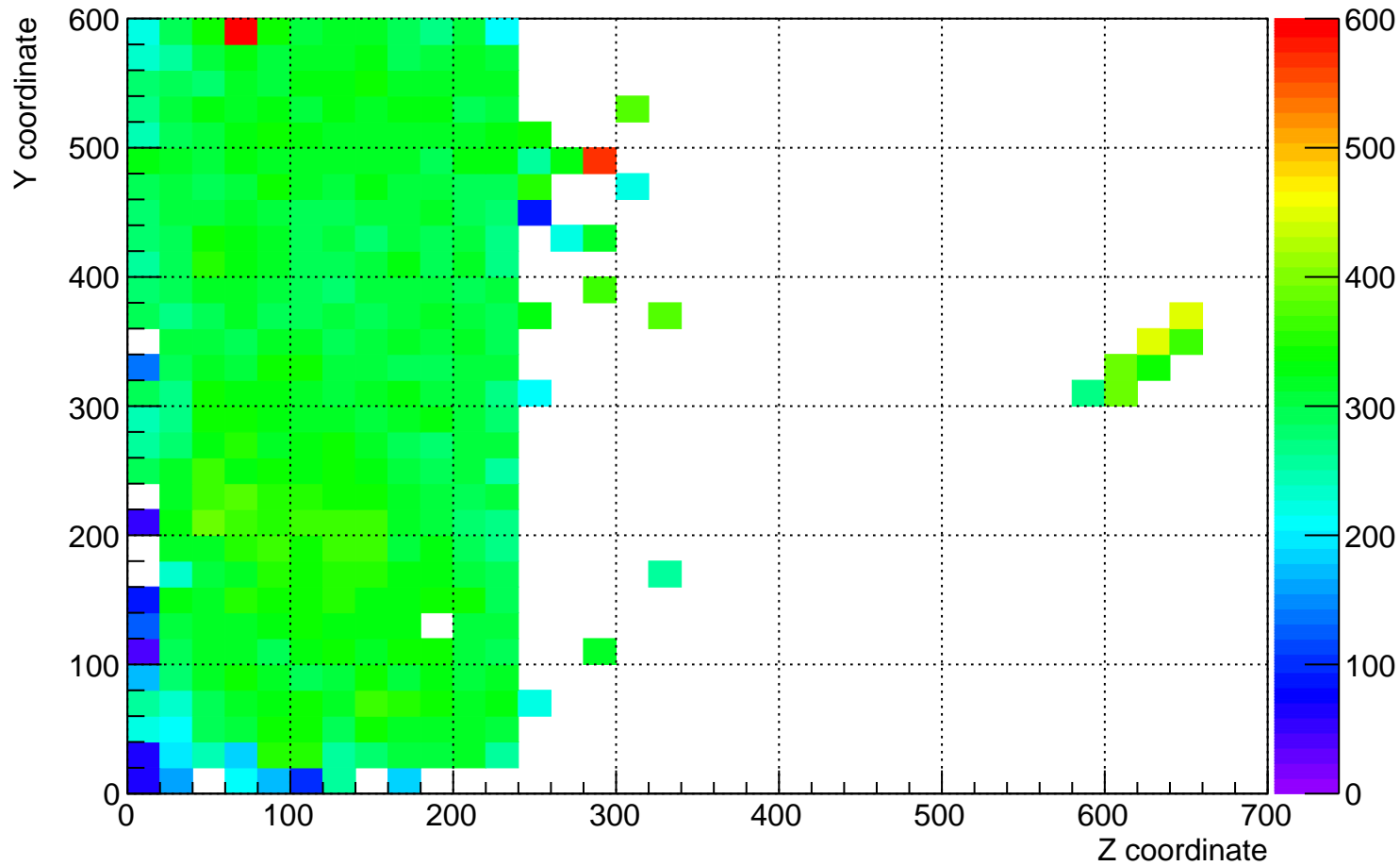
plane_1 (beam left) dQ/dx for YZ plane for time 8 hrs to 9 hrs
