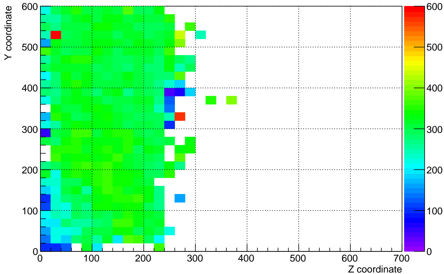
plane_1 (beam left) dQ/dx for YZ plane for time 6 hrs to 7 hrs
