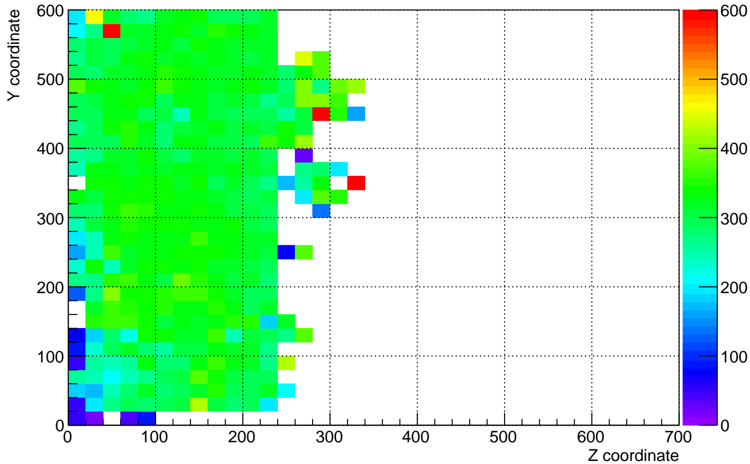
plane_1 (beam left) dQ/dx for YZ plane for time 3 hrs to 4 hrs
