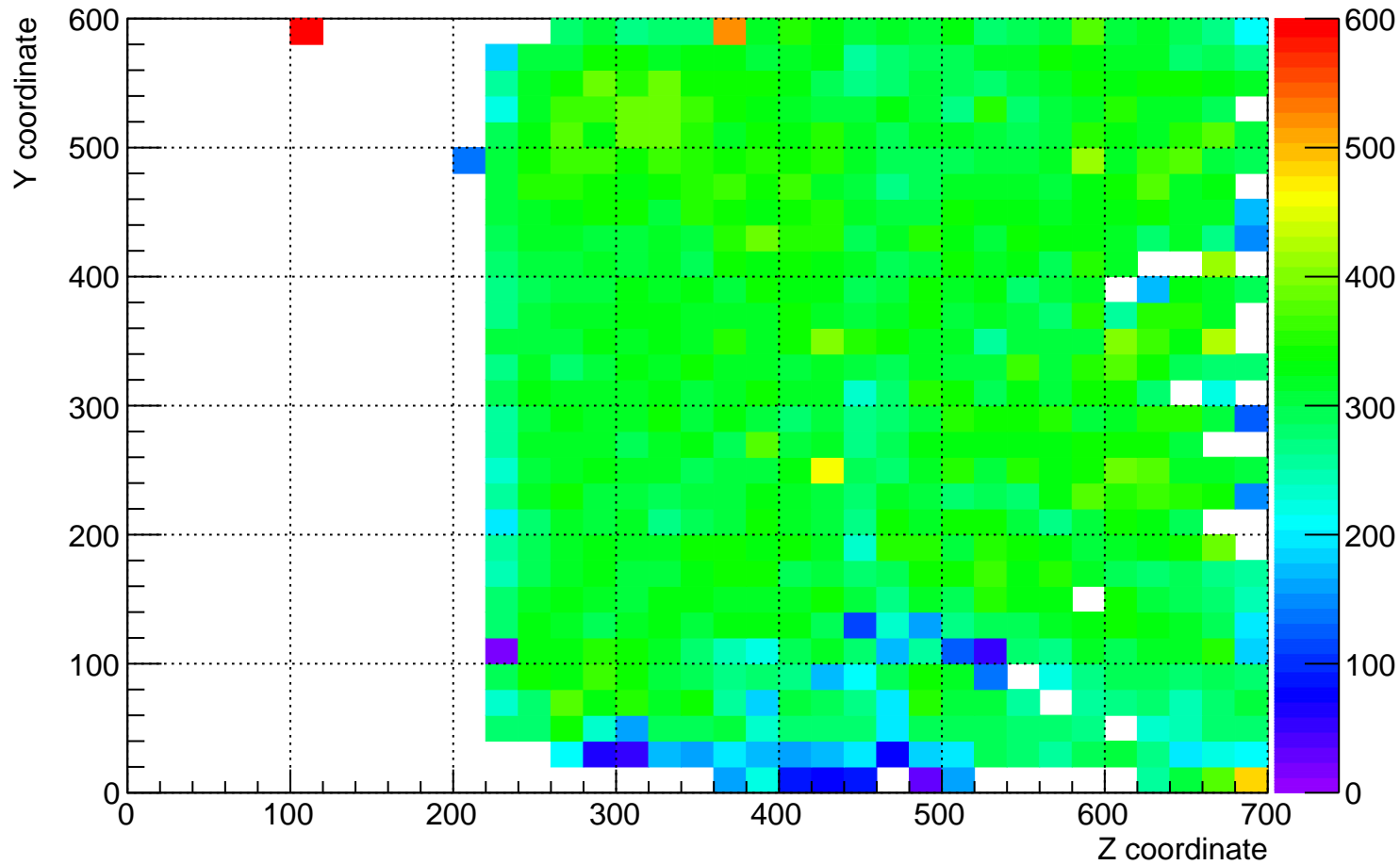
plane_1 (beam right) dQ/dx for YZ plane for time 1 hrs to 2 hrs
