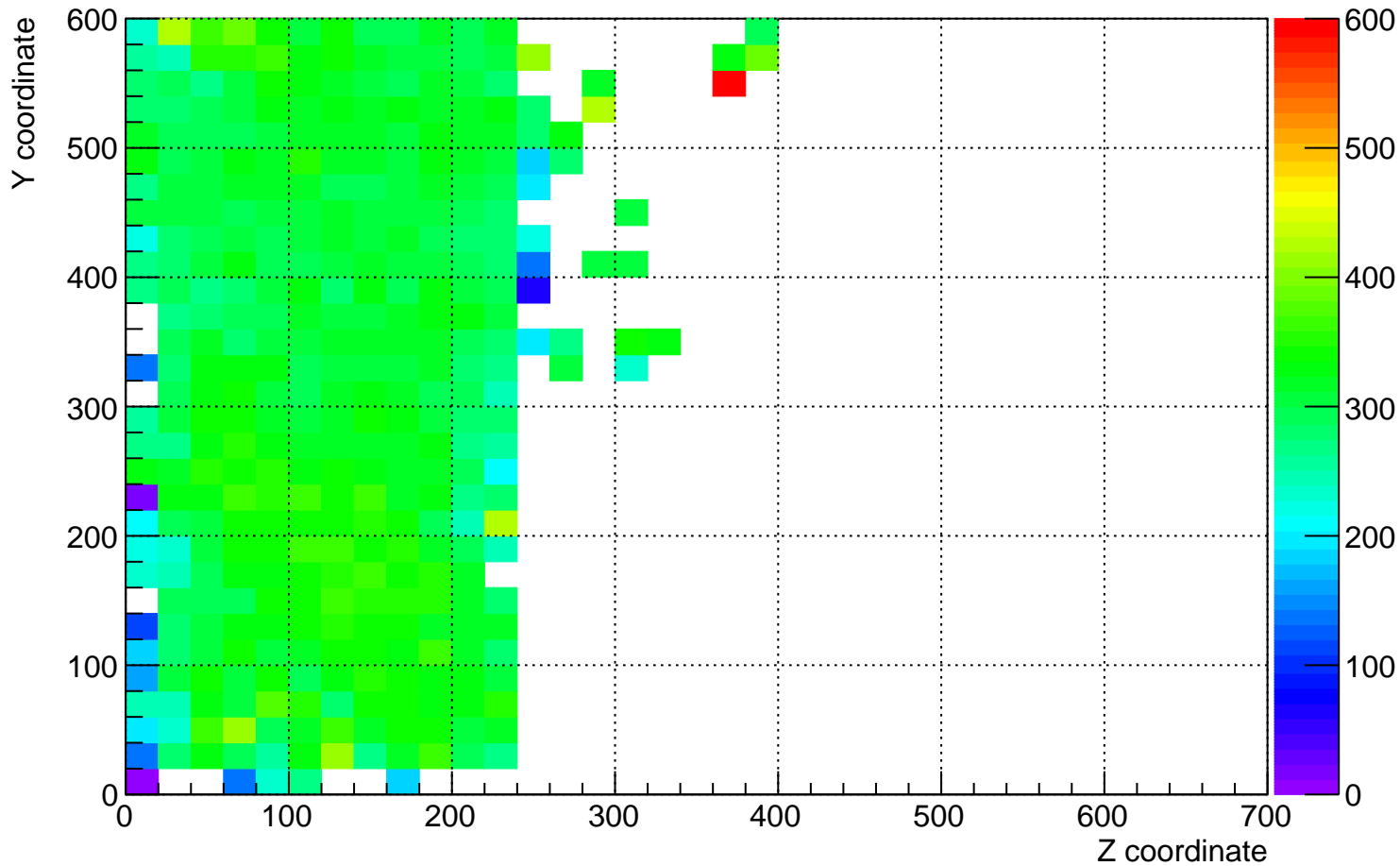
plane_1 (beam left) dQ/dx for YZ plane for time 9 hrs to 10 hrs
