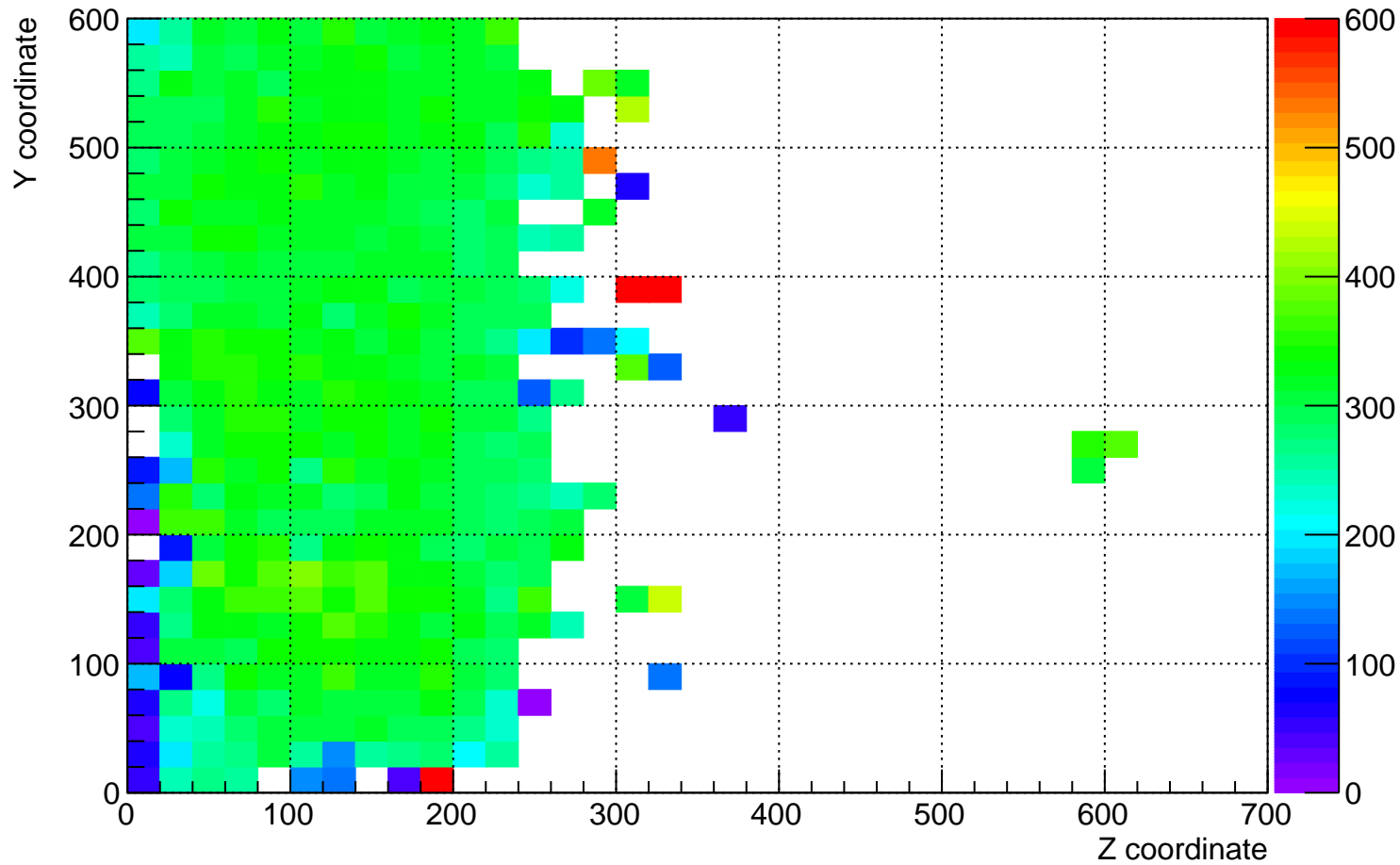
plane_1 (beam left) dQ/dx for YZ plane for time 0 hrs to 1 hrs
