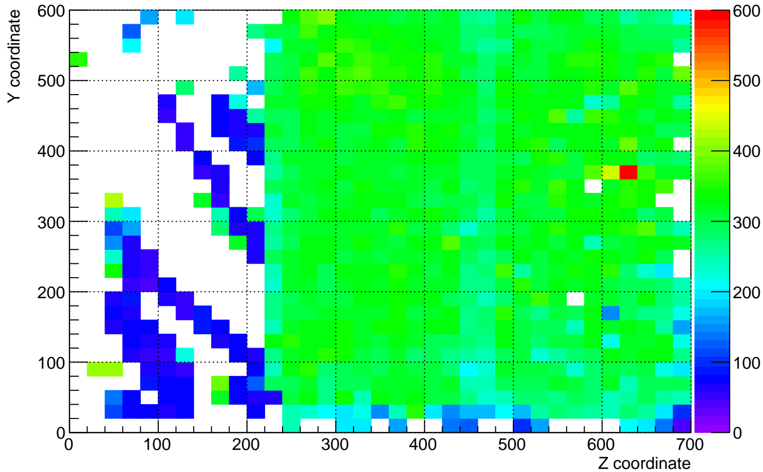
plane_1 (beam right) dQ/dx for YZ plane for time 6 hrs to 7 hrs
