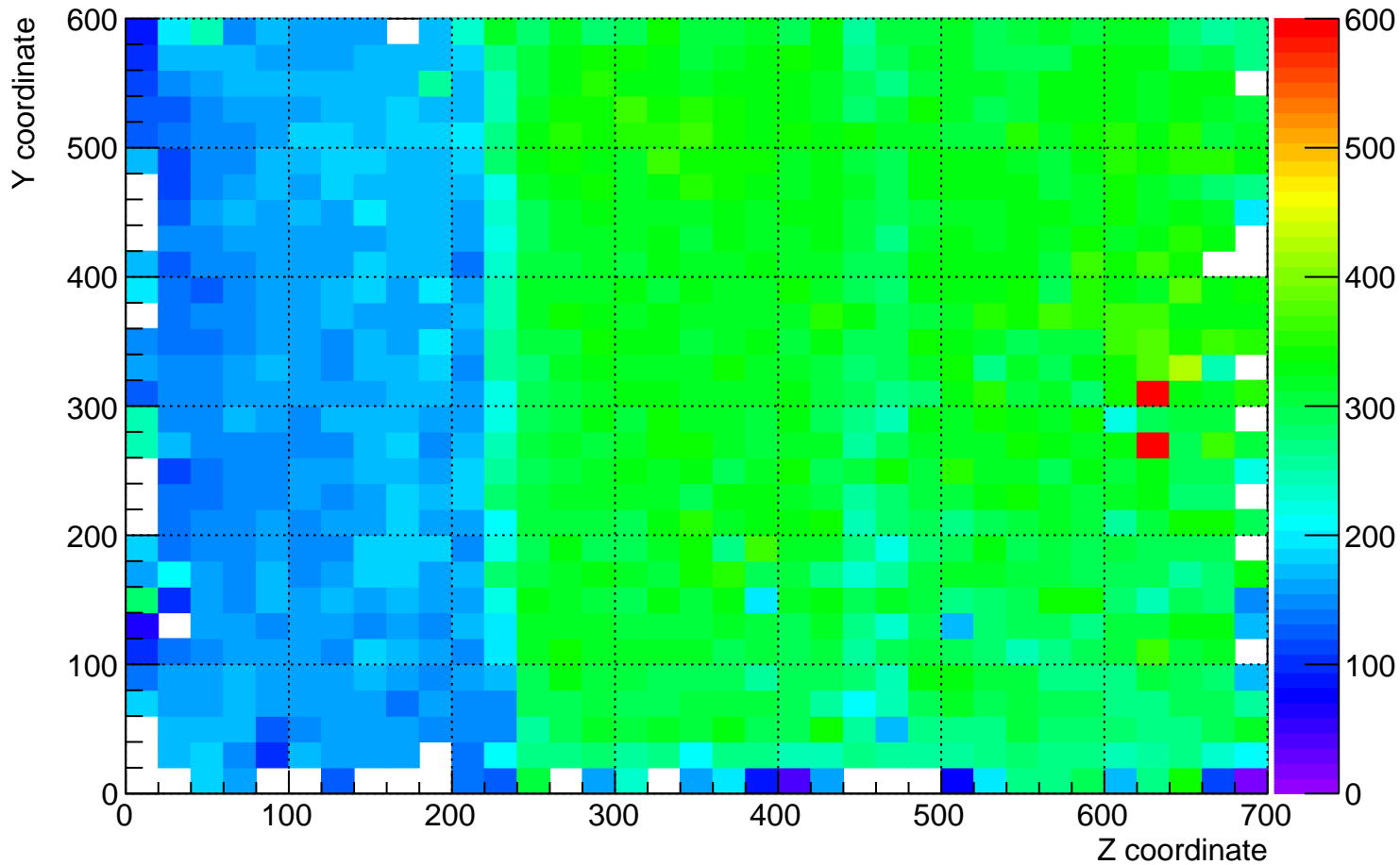
plane_1 (beam right) dQ/dx for YZ plane for time 15 hrs to 16 hrs
