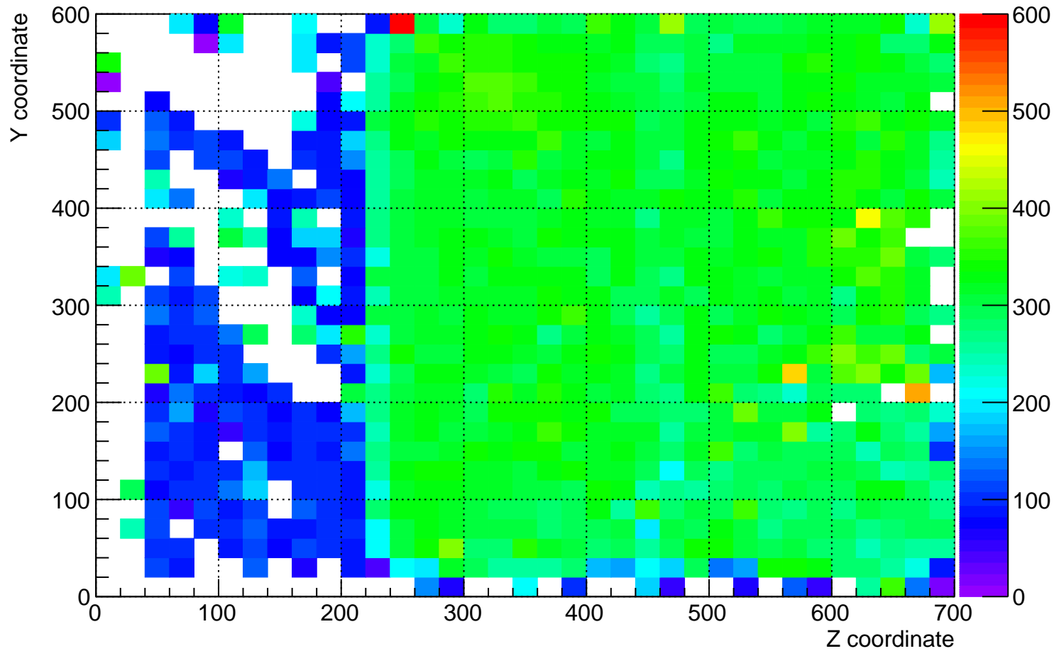
plane_1 (beam right) dQ/dx for YZ plane for time 8 hrs to 9 hrs
