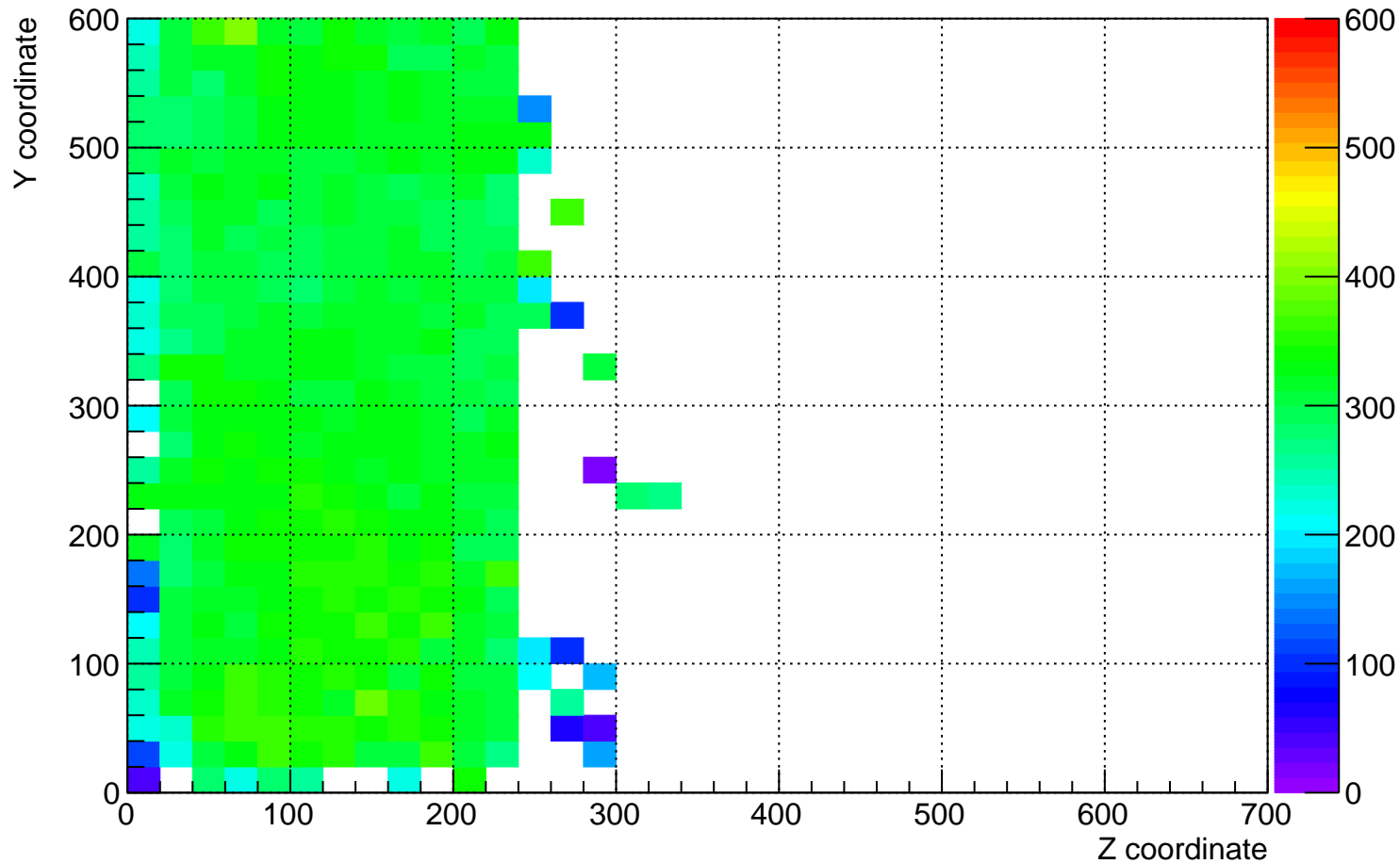
plane_1 (beam left) dQ/dx for YZ plane for time 13 hrs to 14 hrs
