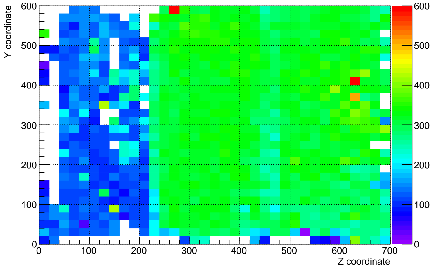
plane_1 (beam right) dQ/dx for YZ plane for time 10 hrs to 11 hrs
