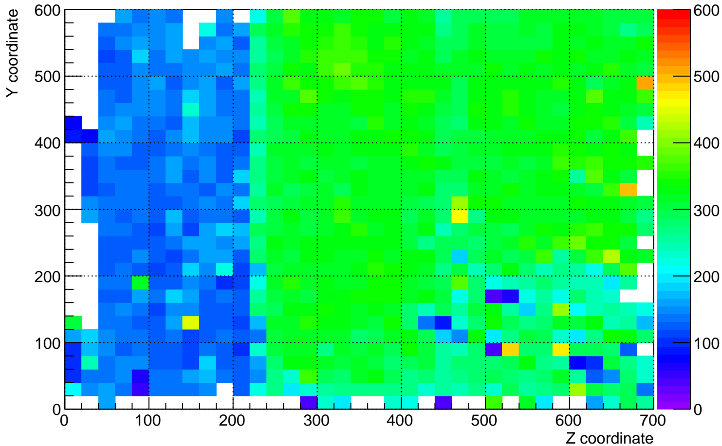
plane_1 (beam right) dQ/dx for YZ plane for time 11 hrs to 12 hrs
