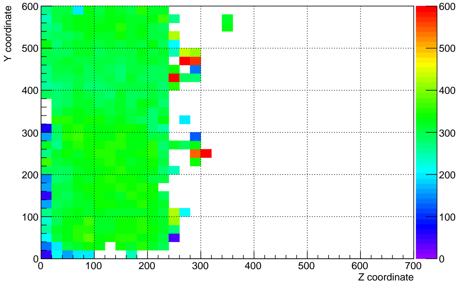
plane_1 (beam left) dQ/dx for YZ plane for time 11 hrs to 12 hrs
