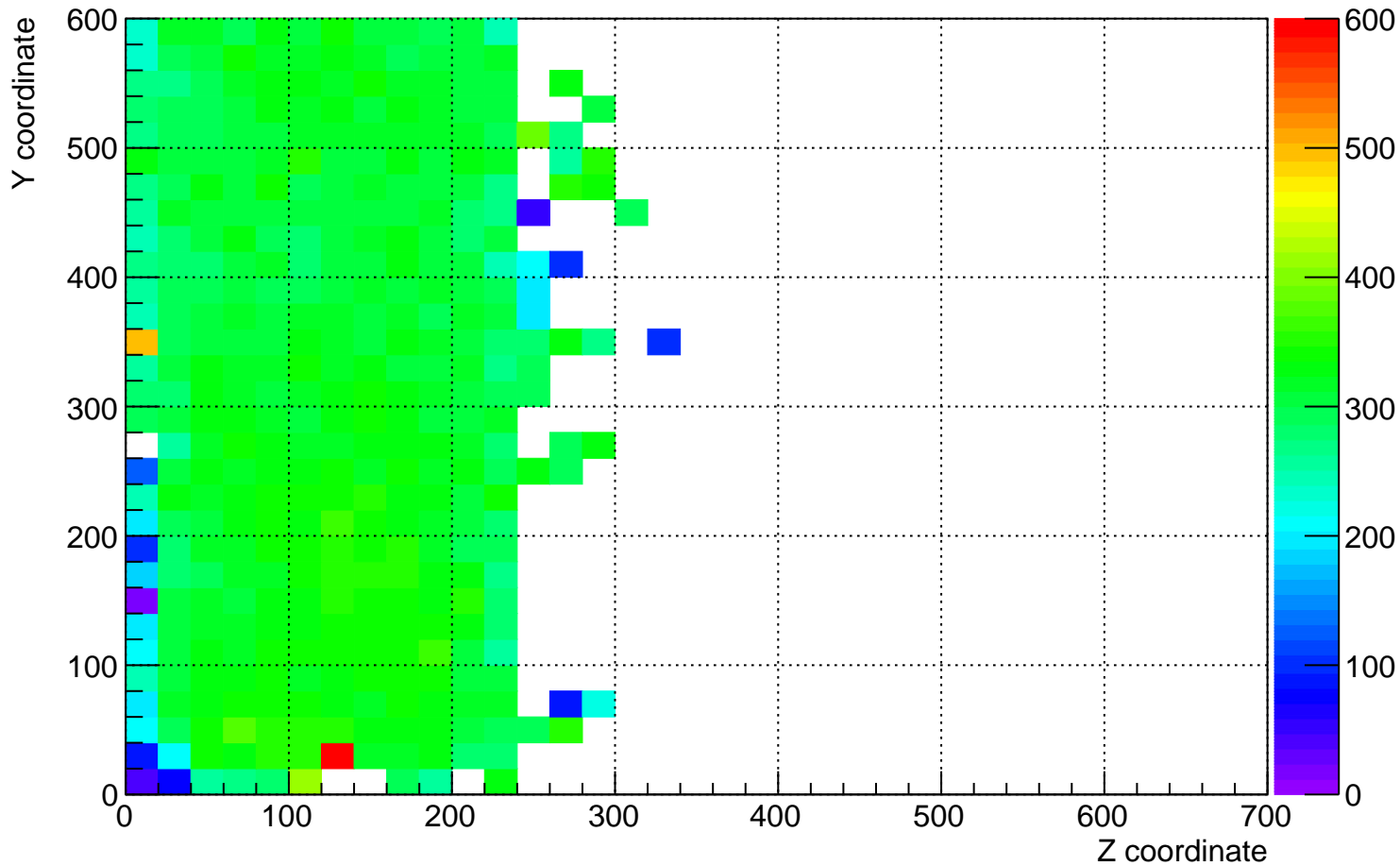
plane_1 (beam left) dQ/dx for YZ plane for time 16 hrs to 17 hrs
