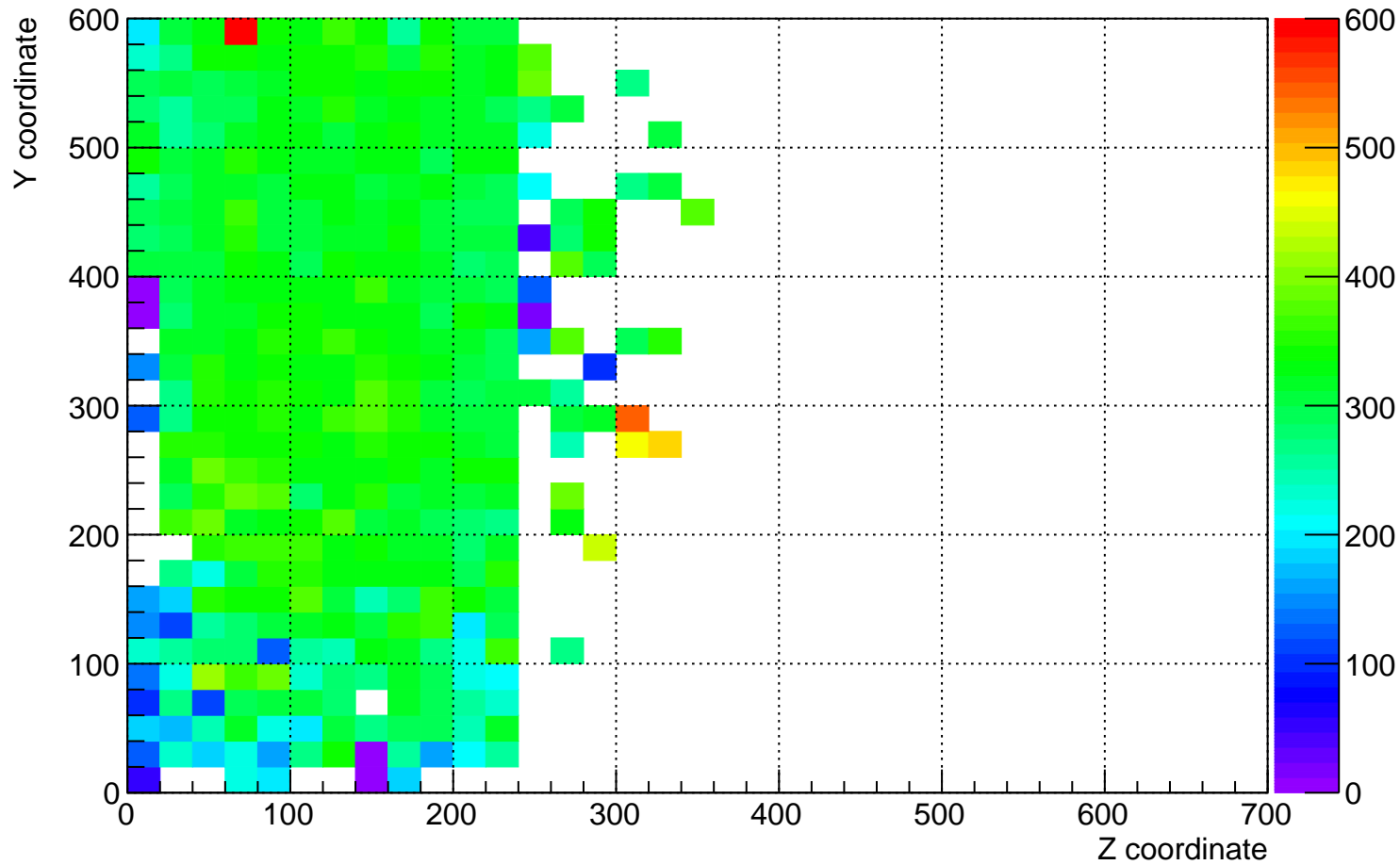
plane_1 (beam left) dQ/dx for YZ plane for time 2 hrs to 3 hrs
