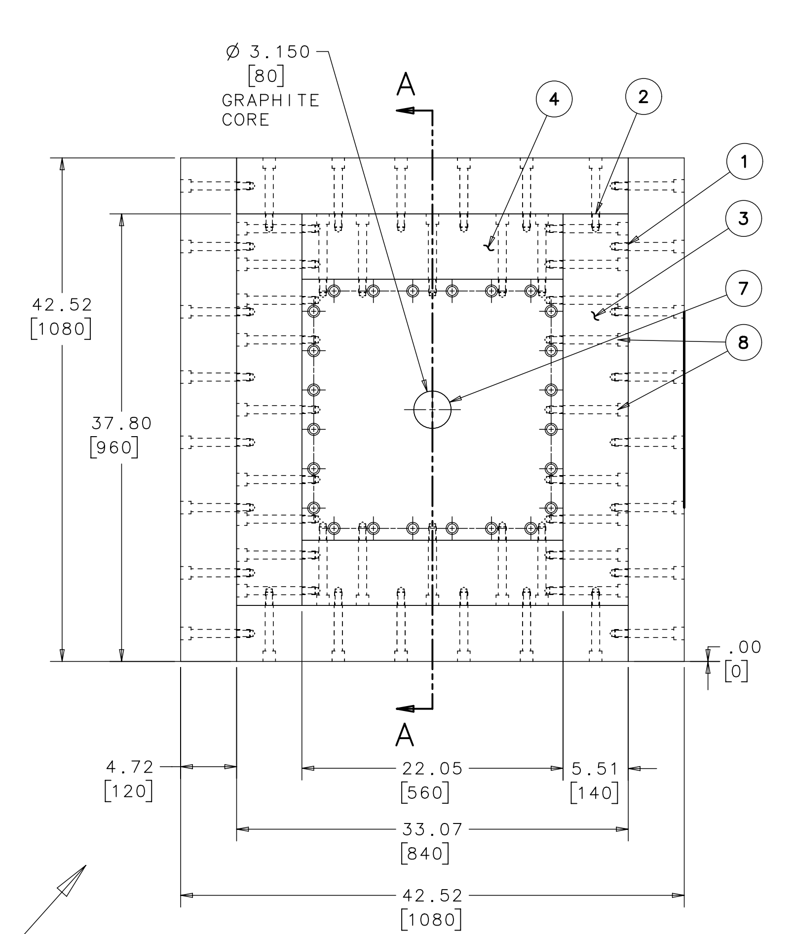
DETAIL SCALE: 1:8 WITHOUT COOLING TUBES
