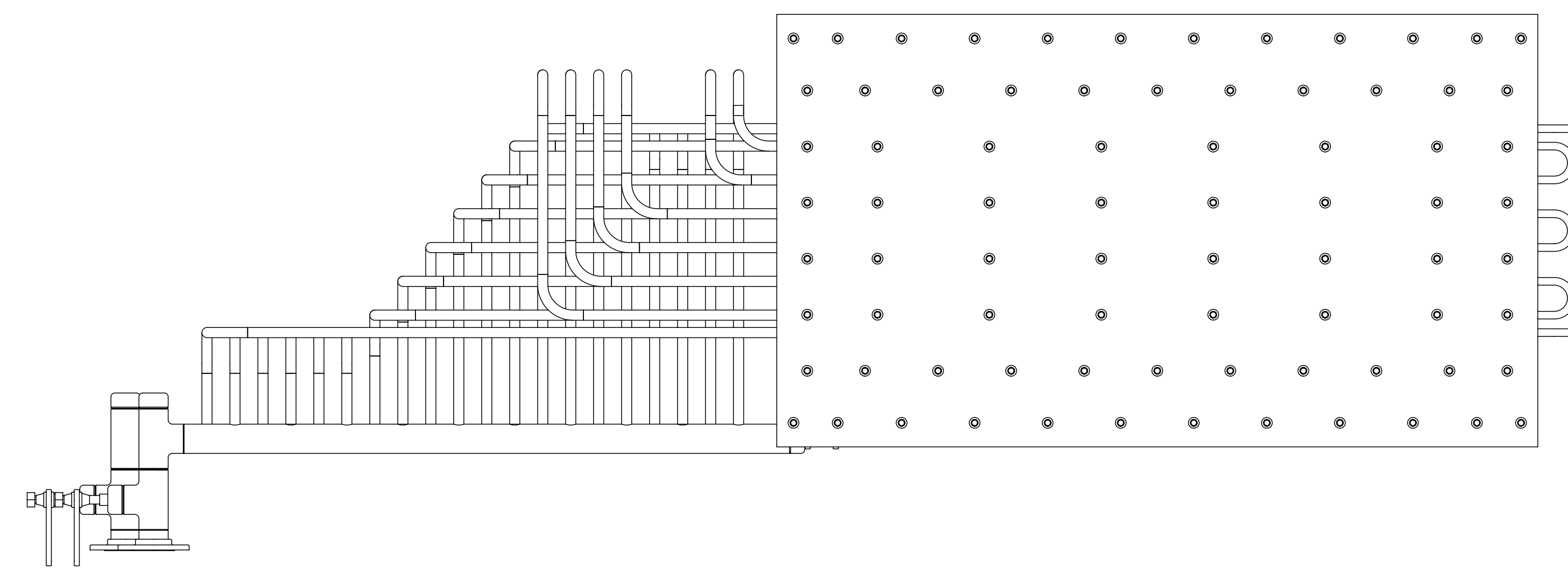
DETAIL SCALE: 1:8 WITHOUT COOLING TUBES
