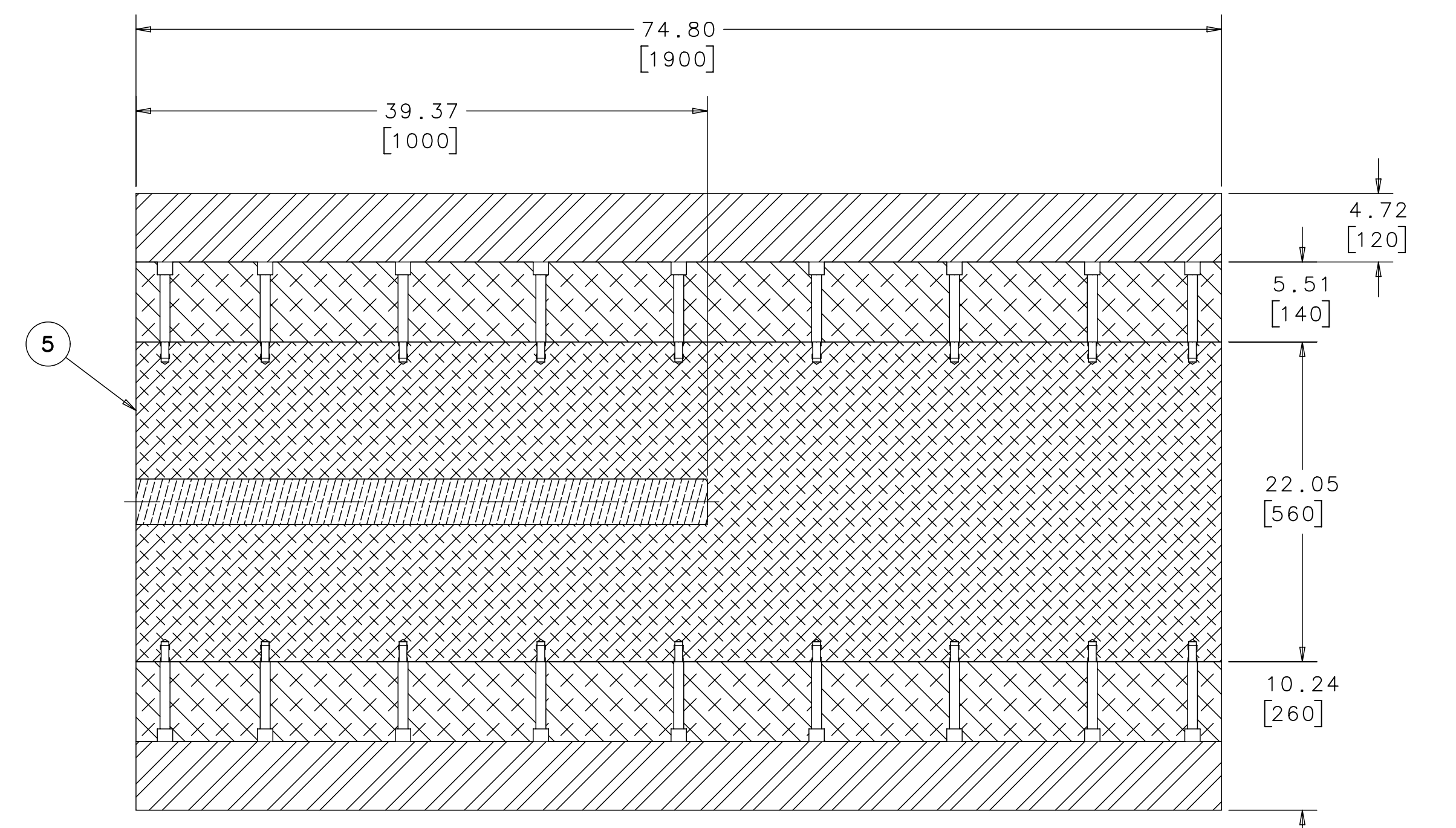
SECTION A-A SCALE 1:8
