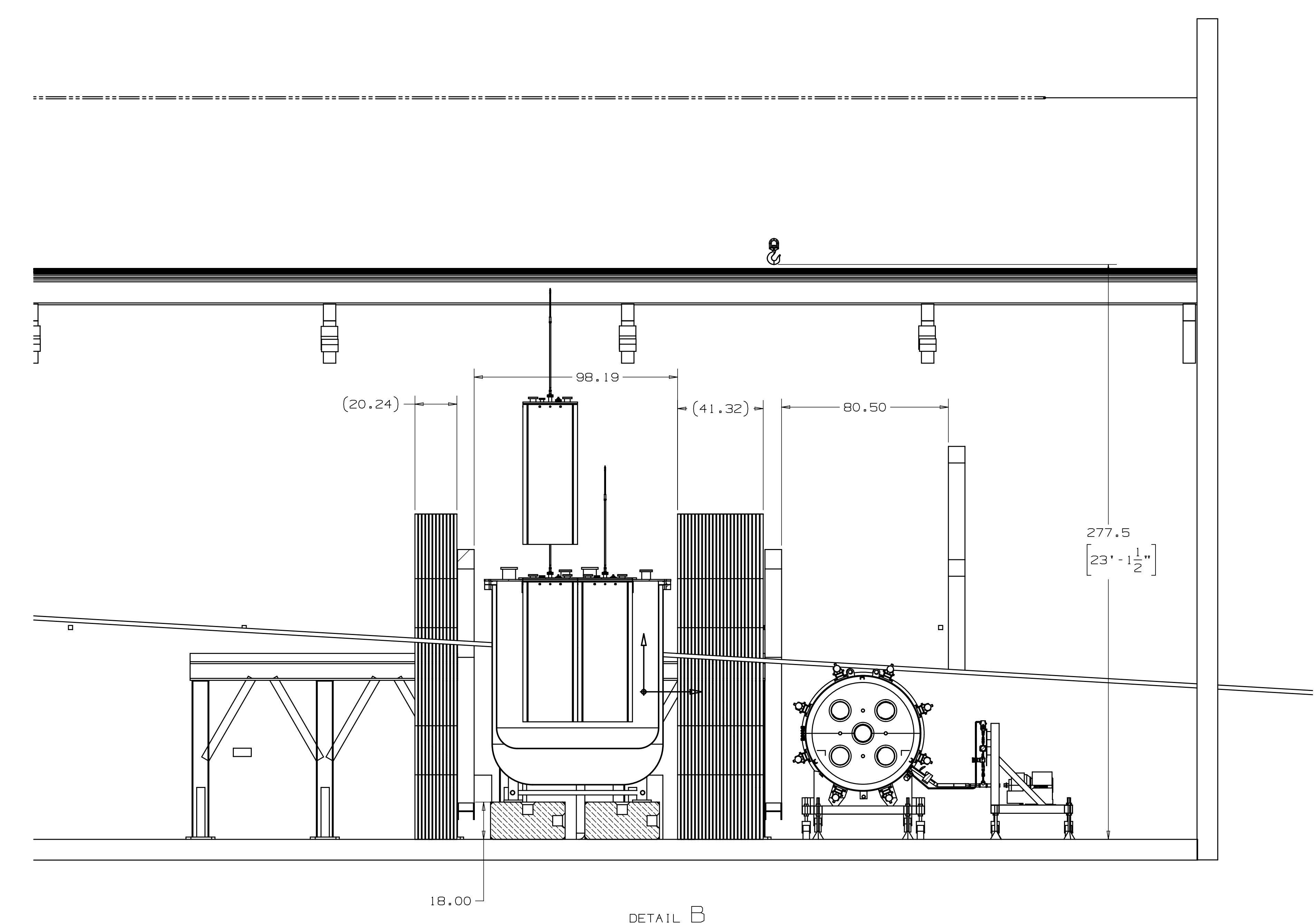
DETAIL B SCALE 1:32
