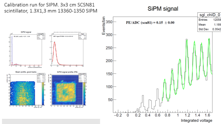
Figure 43: Results from calibration run. The lower left scatter plots show beam profile, leftmost, and scintillator tile light yield in photoelectrons. This tile had artificially low light yield to add in calibration of photoelectrons. (Tile SCSN81tvk) The right-hand plot shows photoelectron fitting. The first 10 photoelectron peaks are clearly visible. PE gain is calculated using this fitting.
