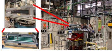
Figure 35: MVTX Telescope Setup at FTBF. A 4-stave telescope assembly was used at Fermilab to verify the detector tracking performance with the latest near final readout electronics and high-speed data cables, and production sensor staves.
