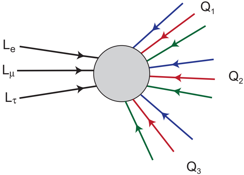
FIG. 5: A B + L violating process due to non-perturbative SM effects.
