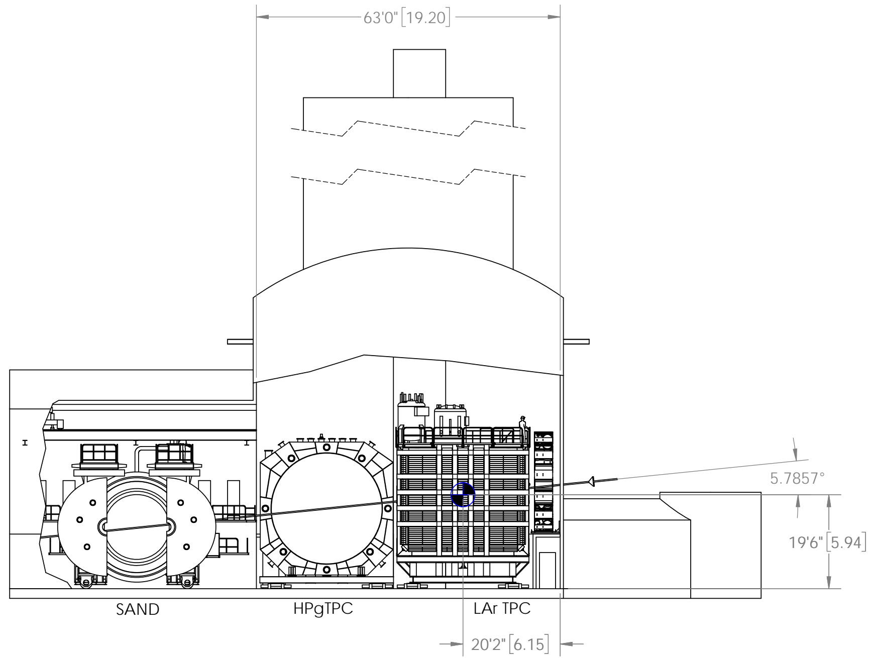
BEAM SWEET SPOT FOR FLOOR DEPTH CALC'S
