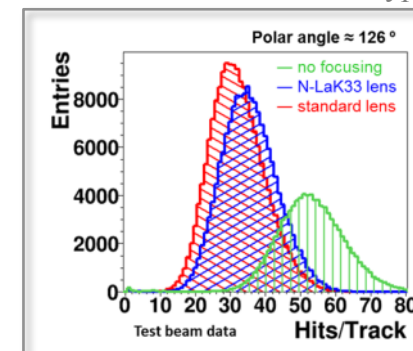
PANDA Barrel DIRC Prototype
