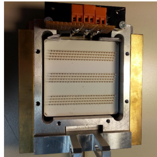
Rear view (anode pin array) in holder
