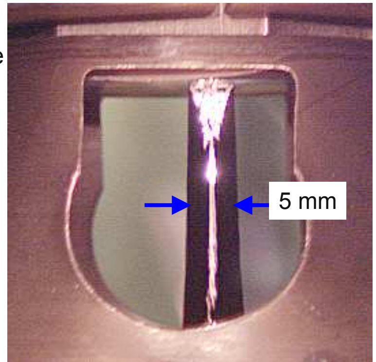
5 x 10 mm liquid Li jet flowing at 10 m/s in vacuum.
