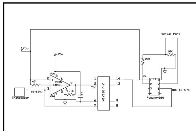
Fig.5. ADC circuit
