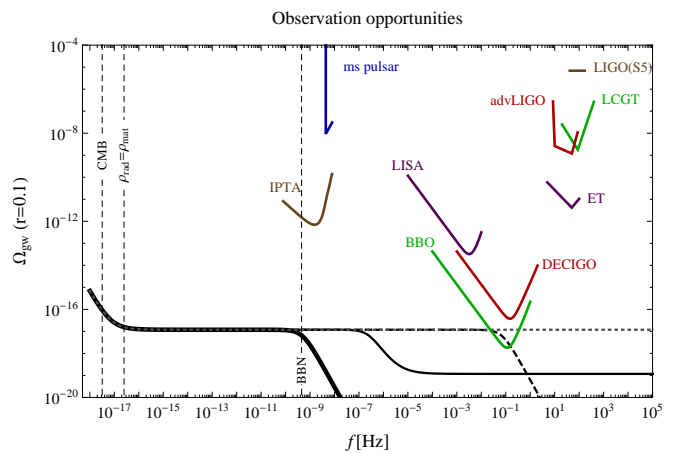
Figure 2: Observation opportunities for the spectra of Fig. 1. In addition to the spectra of Fig. 1, sensitivity curves of existing [17] and future [18] gravitational wave observatories are plotted.
