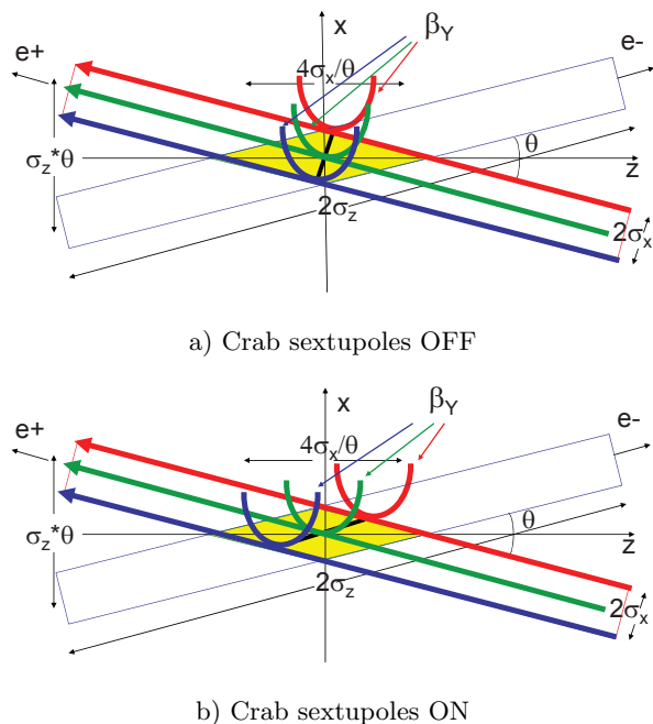
FIG. 11. Crab waist collision scheme [318].
