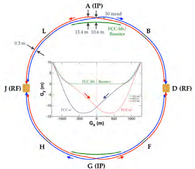
FIG. 28. Layout of the FCC-ee double ring collider with two long RF straights and two interactions points, sharing a tunnel with the full-energy top-up booster [325, 327].
