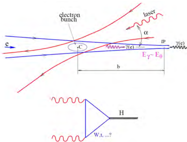
FIG. 40. (top) Scheme of \gamma\gamma , \gamma e collider; (bottom) Higgs production diagram in \gamma\gamma collisions (from Ref.[553]).
