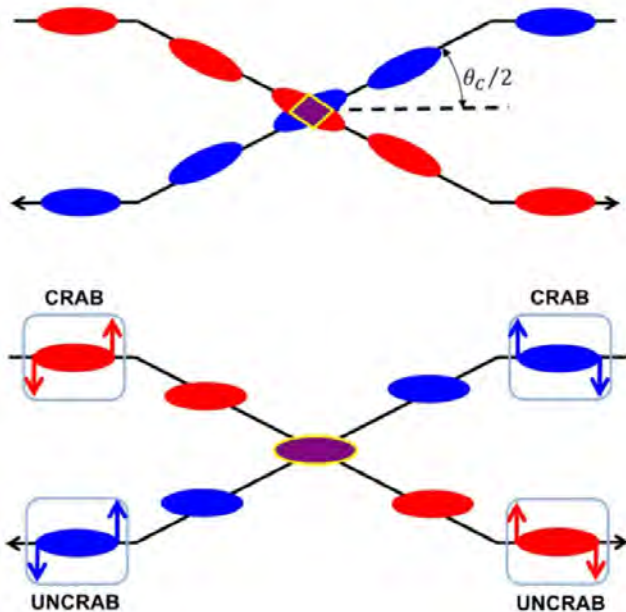
FIG. 9. Top: beam collision scheme with crossing angle suffers from geometric luminosity reduction. Bottom: crab-crossing scheme that results in full bunch overlapping and thus maximum luminosity. Deflecting RF cavities generate a null kick to the center of the bunch while its head and tail receive opposite transverse kicks (from [270]).
