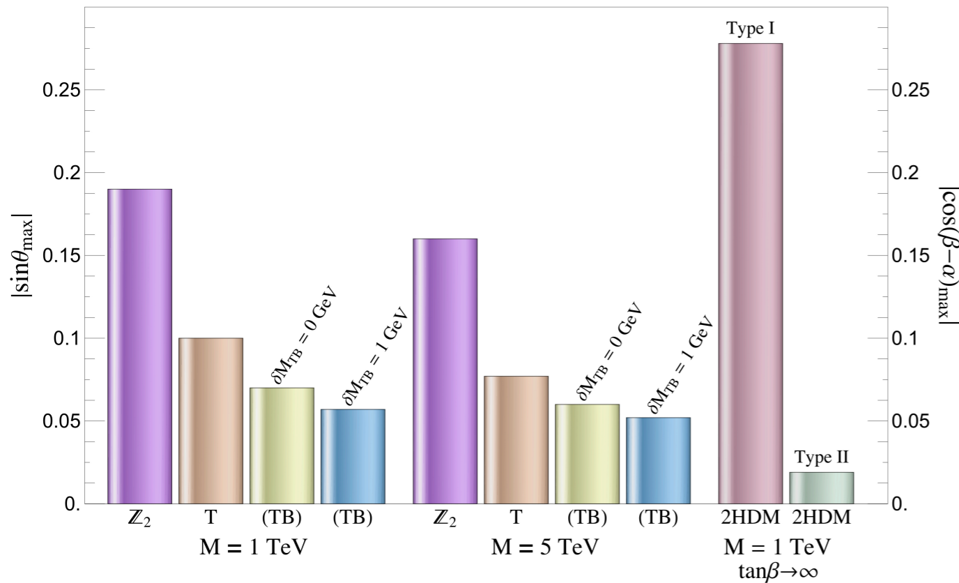
Limits from SMEFT Global Fits
