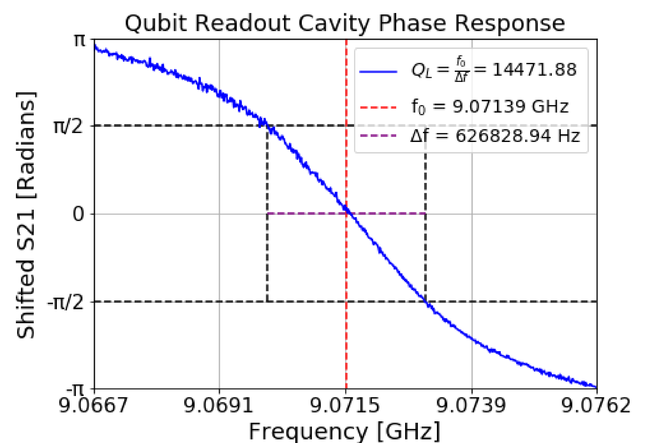
Qubit/Cavity system readout frequency and Q-factor.
