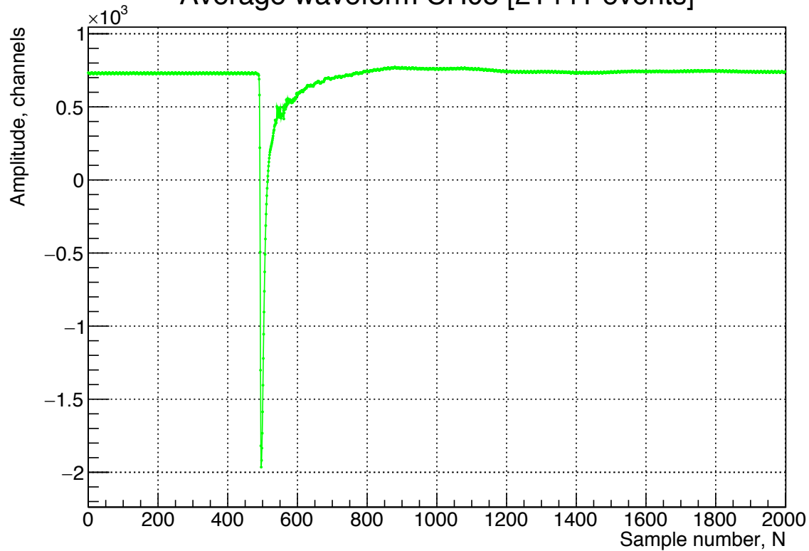
Average waveform CH05 [21441 events]
