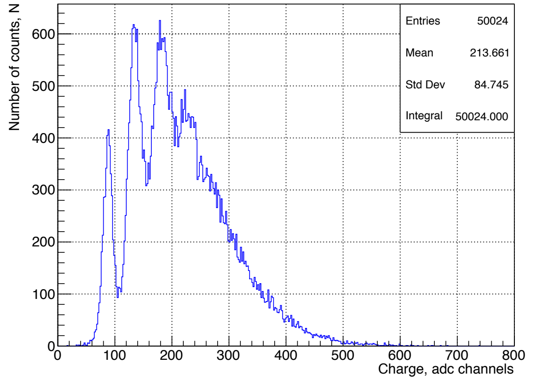
Spectrum [a7b54bd CH07]
