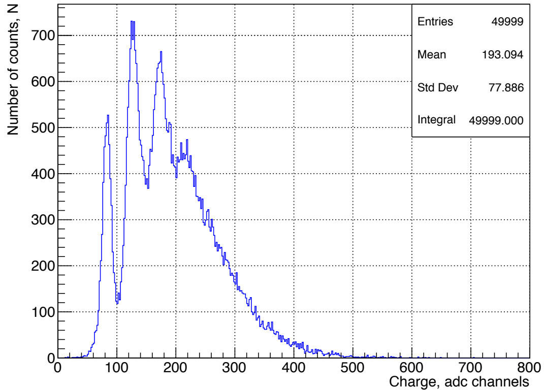
Spectrum [a7b54bd CH02]
