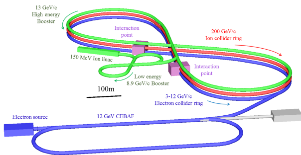
FIG. 18. Layout of the Jefferson Lab Electron-Ion Collider (JLEIC) (from [407]).
