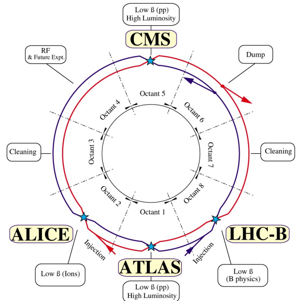
FIG. 14. Layout of the LHC double ring, with its eight long straight sections hosting two general and two special-purpose experimental detectors and/or devoted to specific accelerator functions, such as betatron collimation (cleaning), momentum collimation, beam extraction, RF systems and diagnostics, and injection. (Image credit: CERN).
