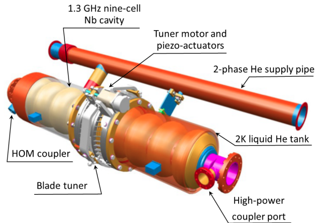
FIG. 5. The baseline superconducting cavity package (dressed cavity) of the International Linear Collider; the titanium helium tank is shown as transparent for a view of the 1 m long 9-cell niobium RF cavity inside (adapted from [75]).
