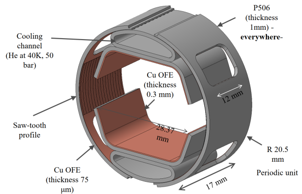
FIG. 31. A periodic unit of the FCC-hh vacuum beamscreen, which will be mounted inside the magnet cold bore (1.9 K) [486]. This beamscreen will be operated at an elevated temperature of about 50 K for efficient removal of the heat from synchrotron radiation.
