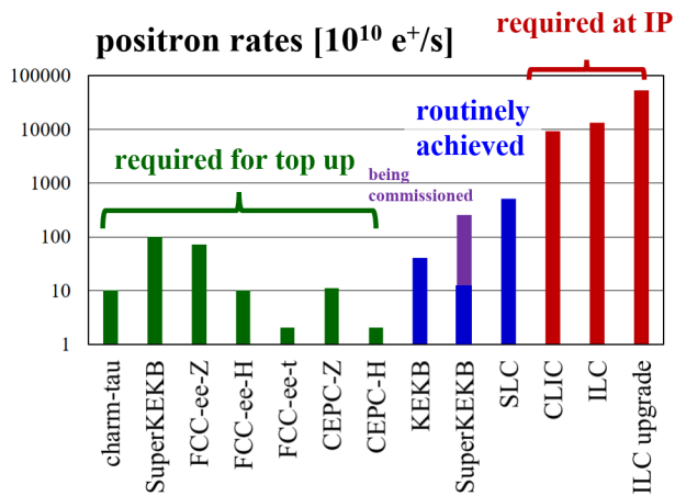
FIG. 26. Positron production rates achieved at the SLC, KEKB and SuperKEKB compared with the need for top-up injection at future circular and linear e^+e^- colliders (also in Ref. [456]).
