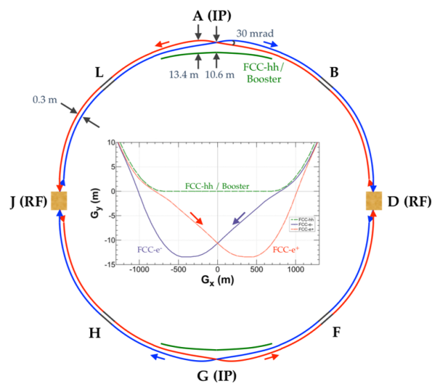
FIG. 28. Layout of the FCC-ee double ring collider with two long RF straights and two interaction points, sharing a tunnel with the full-energy top-up booster [325, 327].
