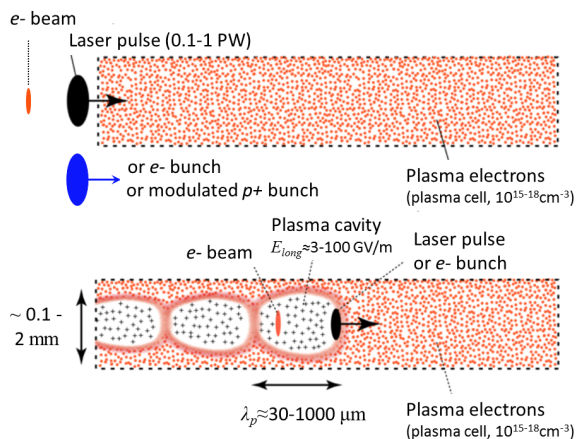
FIG. 37. Concept of the plasma wakefield acceleration driven either by a short laser pulse (LWFA), or by a short electron bunch or by long(er) modulated proton bunch (PWA), adapted from [518].
