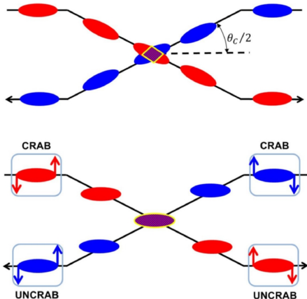
FIG. 9. Top: beam collision scheme with crossing angle suffers from geometric luminosity reduction. Bottom: crab-crossing scheme that results in full bunch overlapping and thus maximum luminosity. Deflecting RF cavities generate a null kick to the center of the bunch while its head and tail receive opposite transverse kicks (from [270]).
