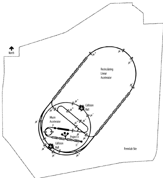
FIG. 34. Schematic of a 4 TeV Muon Collider on the 6×7 km FNAL site (from Ch.12.2 Ref. [36]).
