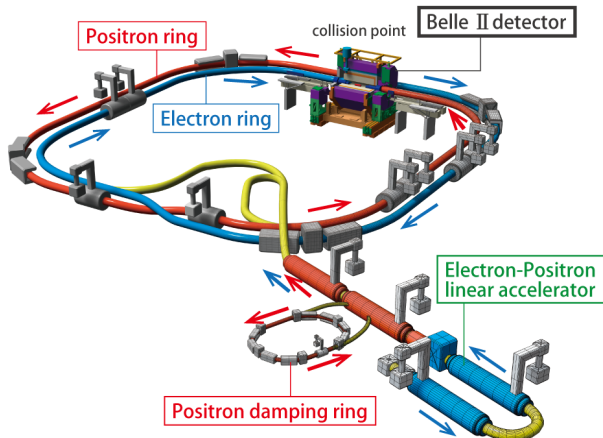
FIG. 12. Schematic of SuperKEKB (Courtesy: KEK).
