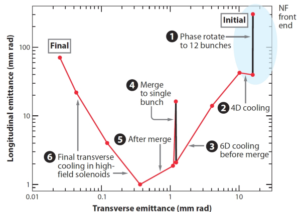
FIG. 36. Simulated six-dimensional (6D) cooling path [499] corresponding to one particular candidate muon collider cooling channel. The first part of the scheme (blue ellipse) is identical to the present baseline neutrino factory front end (from Ref.[495]).
