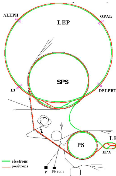
FIG. 8. Schematic view of the LEP injector chain of accelerators and the LEP storage ring [240] with the four experiments ALEPH, DELPHI, L3, and OPAL. The first part of the chain of injectors, the LEP pre-injector (LPI), consisted of two LEP injector linacs (LIL) and an electron/positron storage ring (EPA). Eight positron bunches, followed by eight electron bunches, were ejected from EPA to the Proton Synchrotron (PS), and then accelerated plus extracted to the Super Proton Synchrotron (SPS) for further acceleration. Positrons and electrons were injected into LEP from the SPS, initially at a beam energy of 20 GeV, and later (since 1995) at 22 GeV, to boost the bunch current, which was limited at injection by the TMCI. In its last year of operation (2000), the LEP reached a maximum e^+e^- collision energy of 209 GeV.
