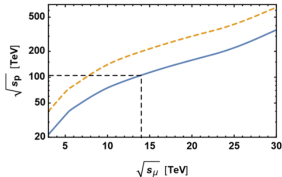
FIG. 33. Energy reach of muon-muon collisions: the energy at which the proton collider cross-section equals that of a muon collider (from Ref. [489]). The dashed line assumes comparable Feynman amplitudes for muon and proton production processes.
