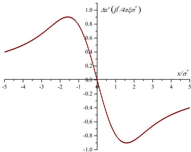
FIG. 6. Angular kick due to beam-beam force.
