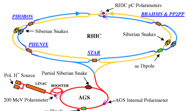
FIG. 13. Layout of the RHIC collider with its injector complex [335]. The two RHIC rings cross in six points. The two principal experiments still running are PHENIX and STAR. The smaller experiments PHOBOS, BRAHMS and PP2PP have been completed. The LINAC is the injector for polarized protons into the Booster/AGS/RHIC chain. A jet target used for precision beam polarization measurements. A tandem injector for ions has been replaced by an Electron Beam Ion Source (EBIS) starting with the 2012 run.
