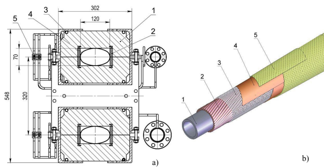
FIG. 16. Superferric 1.8 T magnets of the NICA collider: a) (left) cross-section of the magnet, based on a cold, window-frame iron yoke and a hollow superconductor winding: 1 — lamination, 2 — SC cable, 3 — yoke cooling tube, 4 — beam pipe, 5 — current carrying bus bars. The magnets are placed in a 4.5 K cryostat (not shown); b) (right) 10.4 kA SC cable: 1 — 3 mm diameter cooling tube, 2 — Nb-Ti SC wire, 3 — Ni-Cr wire, 4 and 5 — insulation tapes (adapted from [387]).
