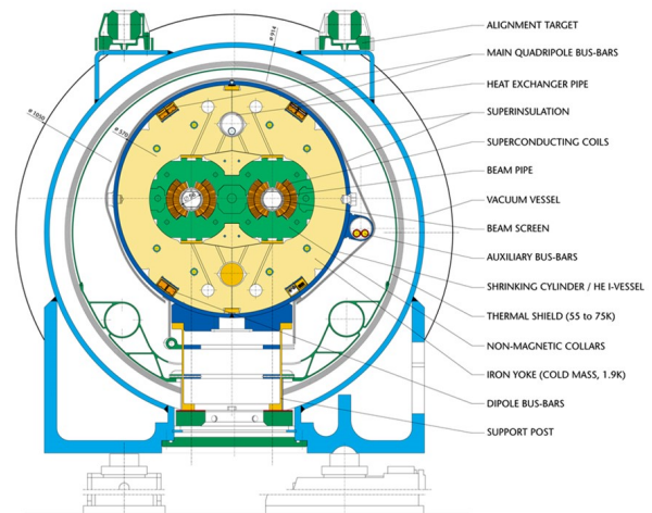
FIG. 4. Cross section of the 14.3 m long superconducting magnet of the Large Hadron Collider [70]. The design field of 8.33 T is vertical and opposite in the two 56 mm diameter bores for the two counter-rotating beams, with a horizontal beam-to-beam separation of 194 mm. The LHC comprises 1232 main dipoles, each weighing about 35 tons.
