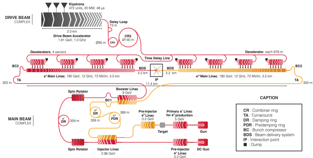
FIG. 24. CLIC accelerator complex layout at \sqrt{s}=380 GeV [446].
