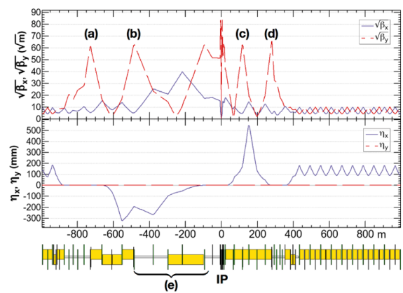
FIG. 27. Asymmetric final-focus optics of FCC-ee, featuring four sextupoles (a–d) for local vertical chromaticity correction combined with a virtual crab waist (see text for details) [325, 327].
