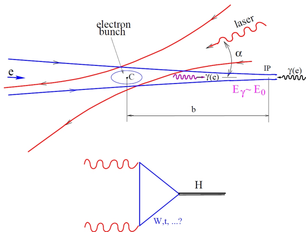
FIG. 40. (top) Scheme of \gamma\gamma , \gamma e collider; (bottom) Higgs production diagram in \gamma\gamma collisions (from Ref.[553]).
