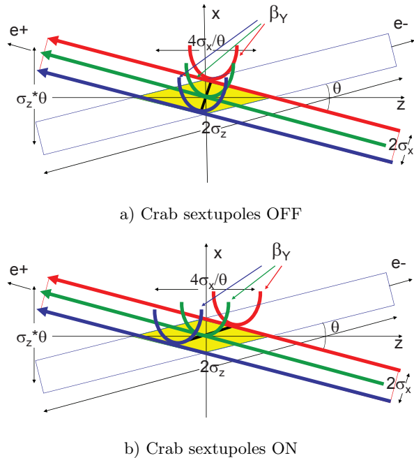
FIG. 11. Crab waist collision scheme [318].
