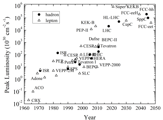
FIG. 3. Luminosities of particle colliders (triangles are lepton colliders and full circles are hadron colliders, adapted from [35]).
