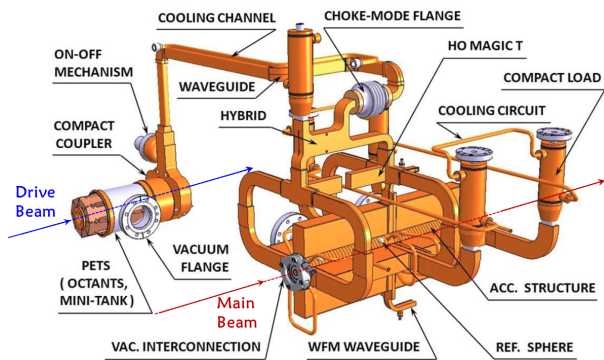
FIG. 23. 3D model of the CLIC two-beam RF module (adapted from [444]).
