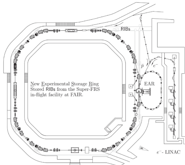
FIG. 17. Conceptual layout of the planned electron(antiproton)-ion collider hosting the ELISE experiment. The intersection region A - B is situated in a bypass section to the New Experimental Storage Ring (NESR) and hosts a dedicated spectrometer (from [397]).
