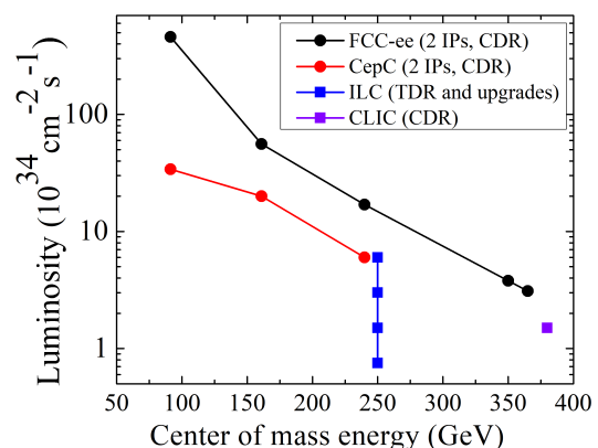
FIG. 22. Luminosity of the proposed Higgs and electroweak factories vs center of mass energy \sqrt{s} = 2E_b .
