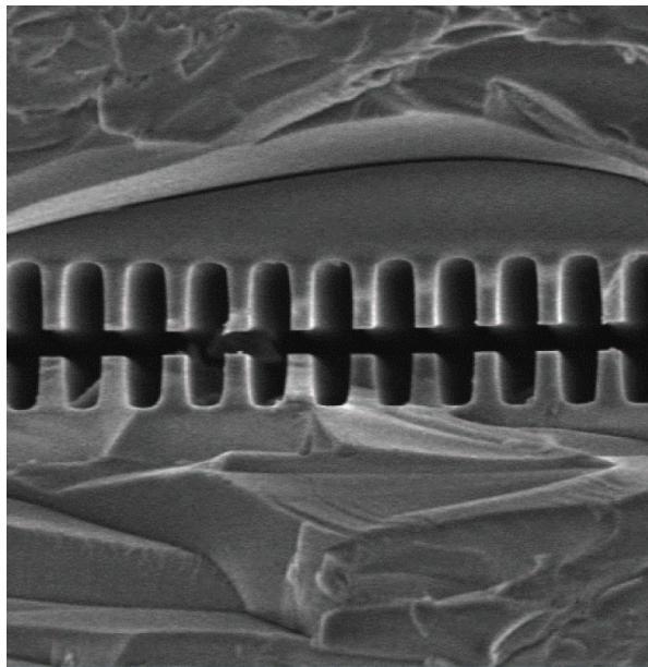
FIG. 41. Scanning electron microscope image of the longitudinal cross-section of a dielectric laser acceleration structure with 400 nm gap [569].
