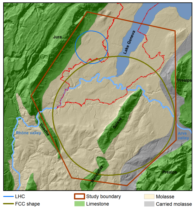
FIG. 29. Study boundary (red polygon), showing the main topographical and geological structures, LHC (blue line) and FCC tunnel trace (brown line) [325, 468].
