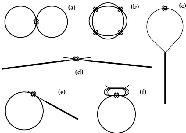
FIG. 1. Schematics of particle collider types.
