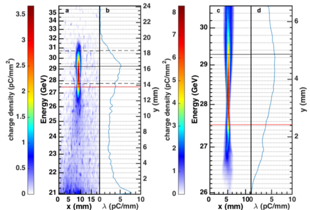
FIG. 38. A 0.1 nC electron bunch gained a maximum energy of 9 GeV in a 1.3 m-long electron plasma wakefield accelerator driven by a 20.35 GeV e^- beam at the FACET facility at SLAC: (a)-(d) show the energetically dispersed transverse charge density profile spectra and the horizontally integrated spectral charge density profiles as observed on the wide-field of view Cherenkov screen and on the order of magnitude more sensitive Lanex screen, respectively (from Ref. [526]).
