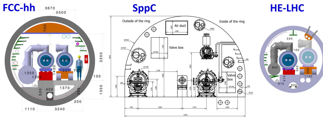
FIG. 32. Tunnel cross sections for FCC-hh, SppC, and HE-LHC, approximately to scale (from Ref. [488]).
