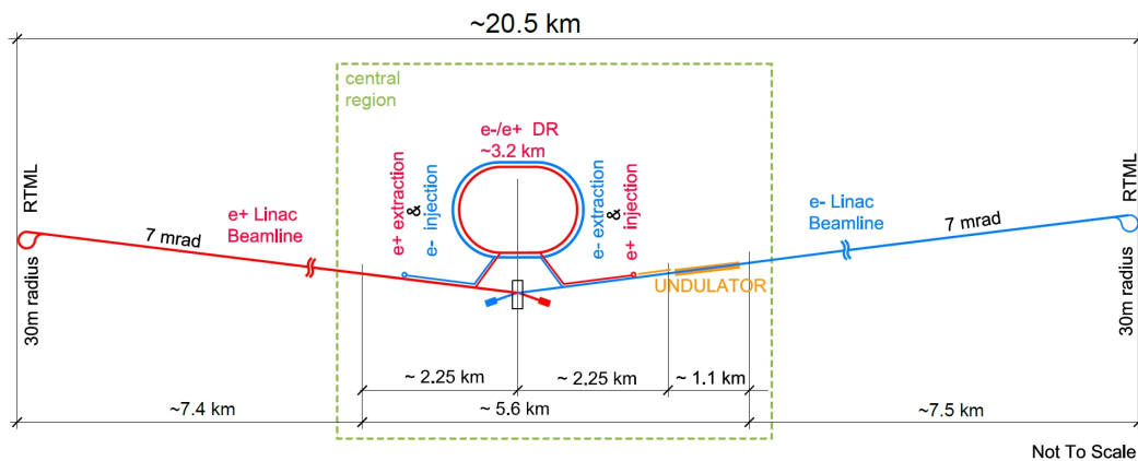
FIG. 21. Schematic layout of the ILC in the 250 GeV staged configuration (from [422]).
