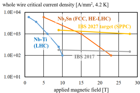
FIG. 30. Field limits for LHC-type Nb-Ti conductor, Nb 3 Sn conductor as used for HL-LHC, FCC-hh and HE-LHC, and iron-based superconductor (present and 10-year forecast) for SppC (after P.J. Lee [479], and private communication J. Gao).
