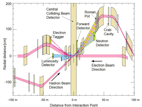
FIG. 20. Layout of the eRHIC interaction region. The length scales for the horizontal and vertical axis are very different. Beams cross with a crossing angle of 25 mrad. The IR design integrates focusing magnets for both beams, luminosity and neutron detectors, electron taggers, spectrometer magnets, near-beam detectors (Roman pots for hadrons), crab cavities, and spin rotators for both beams (from [409]).
