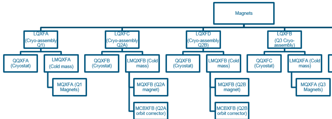
Figure 1: CERN Naming Conventions for HL-LHC Inner Triplets
