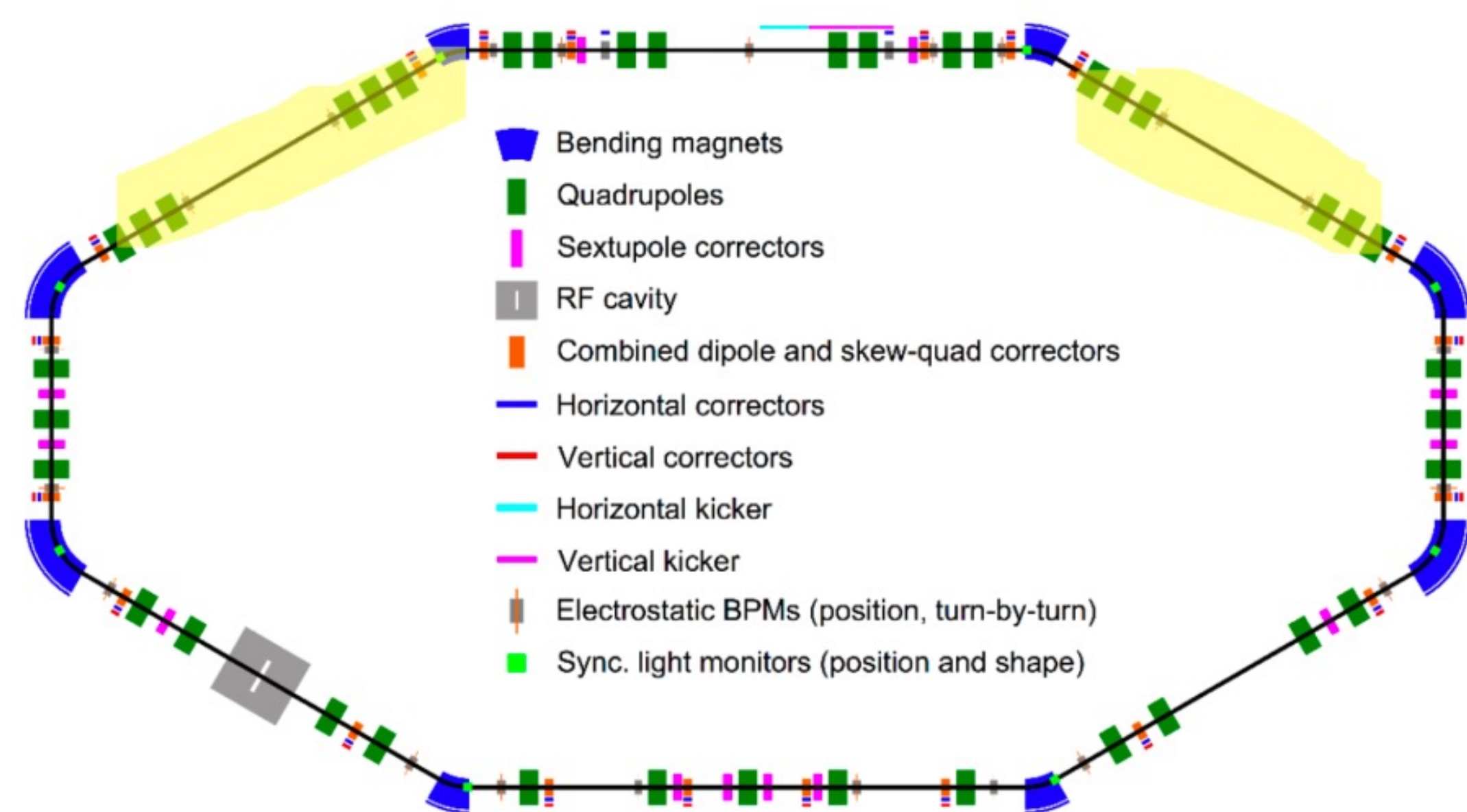
IOTA Schematic
