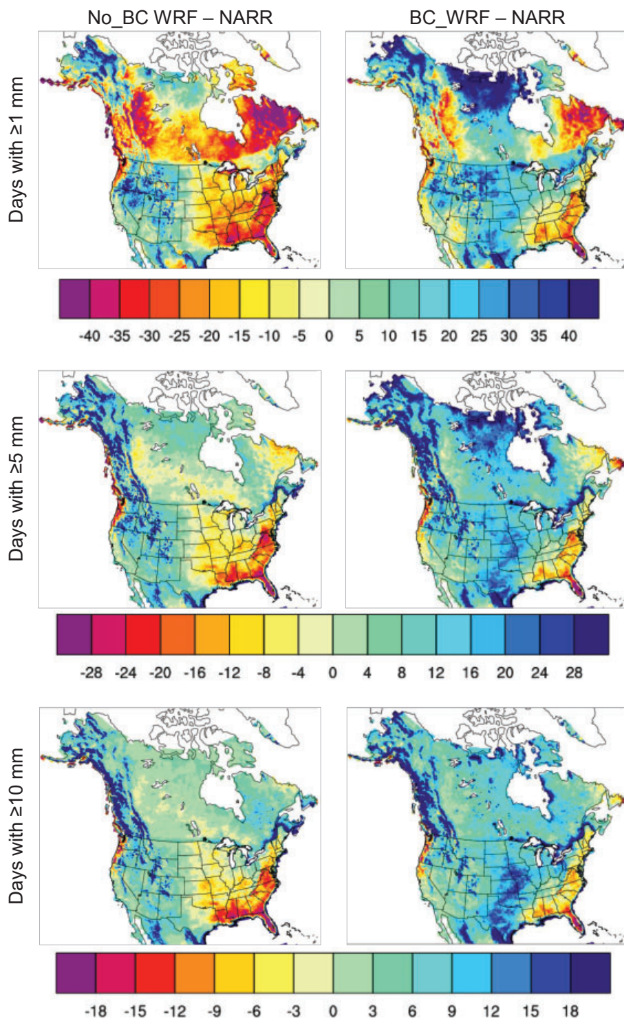
Figure 6. The differences in number of days per year with precipitation amount greater than 1, 5, and 10 mm for No_BC WRF and BC_WRF simulation versus NARR using the 10 year historical simulation (1995–2004).
