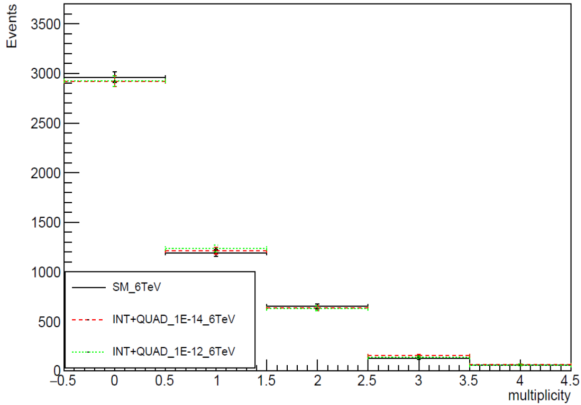
Electron
