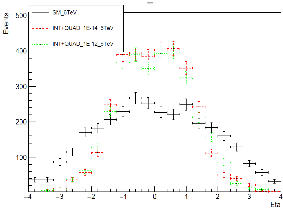
Electron
