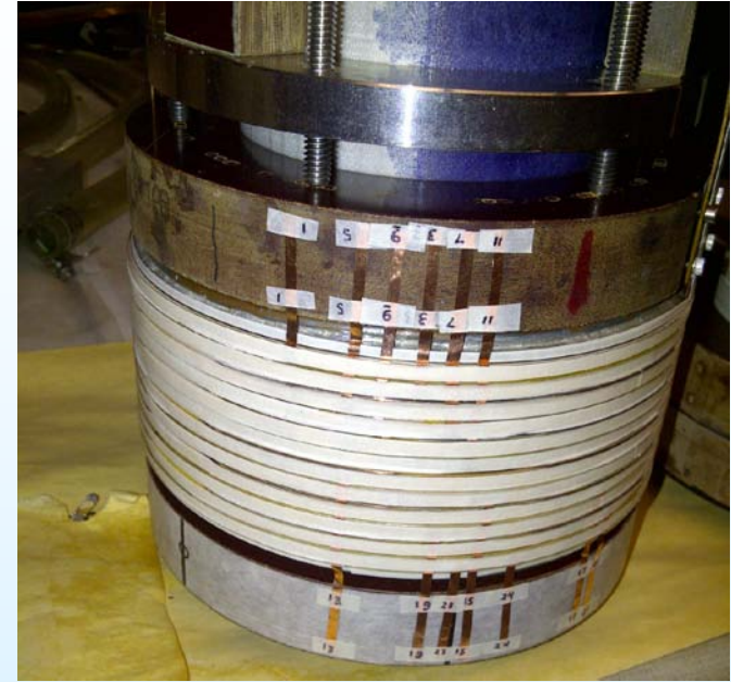
PBL/BNL 100 mm HTS Solenoid Test for Muon Collider
