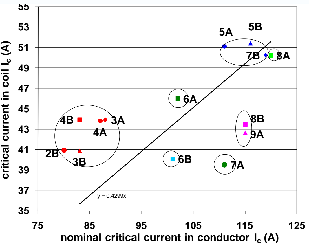
Correlation between 2G Coil Ic and Wire Ic at 77 K
