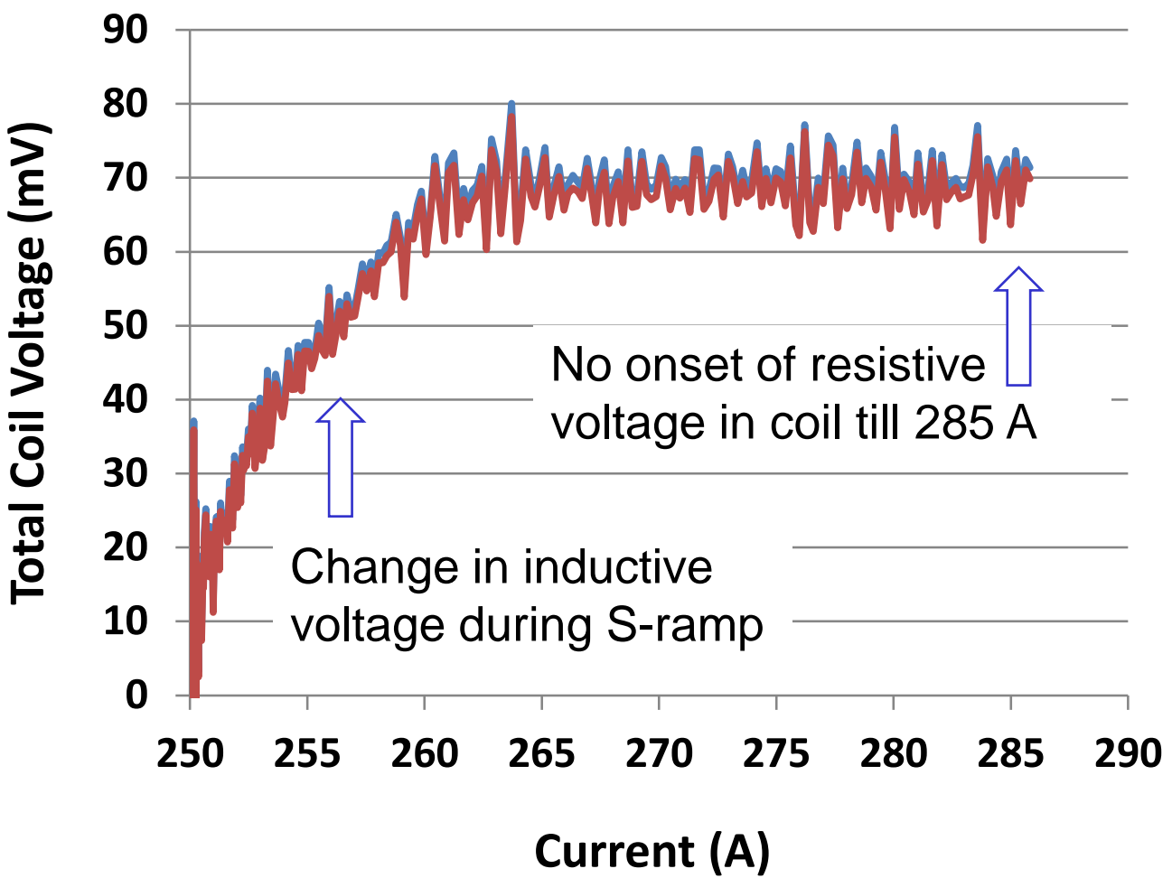
Total Coil Voltage
