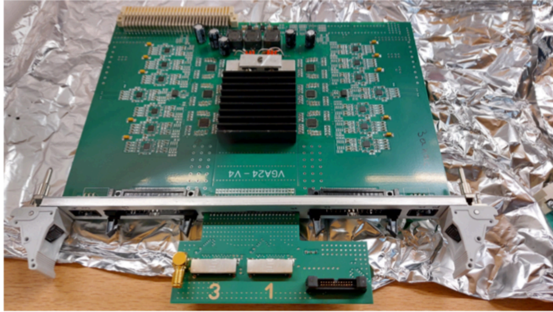
VGA board + Adaptor card for input micro coaxial cables
