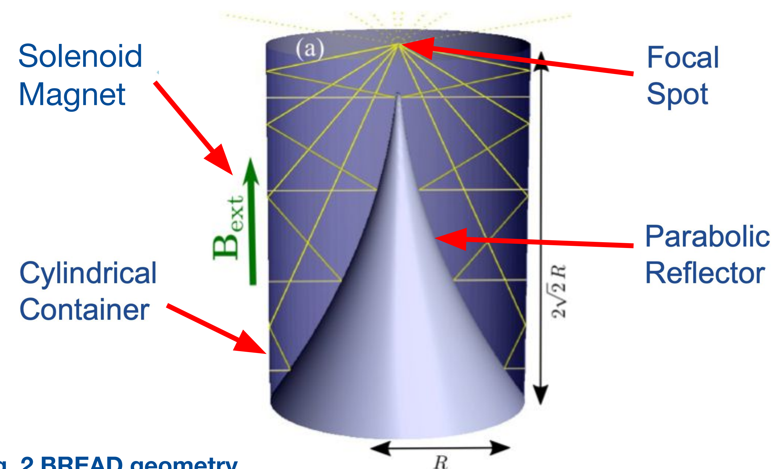
Fig. 2 BREAD geometry.
