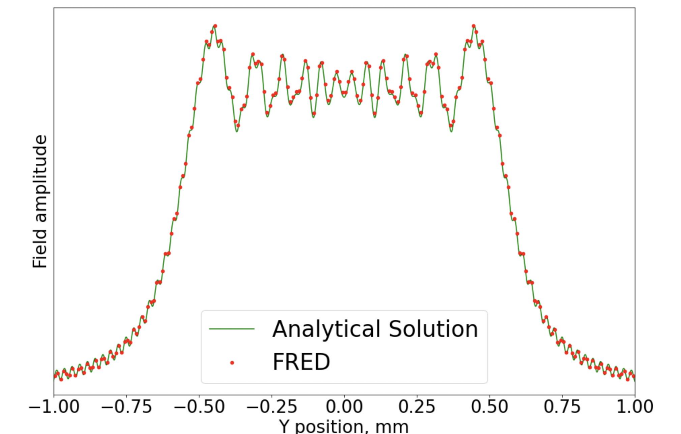
Fig. 4 Diffraction pattern 50 mm behind a 60 \mu\text{m} x 1.3 mm single slit along the long direction of the slit at a wavelength of 0.63 \mu\text{m} .
