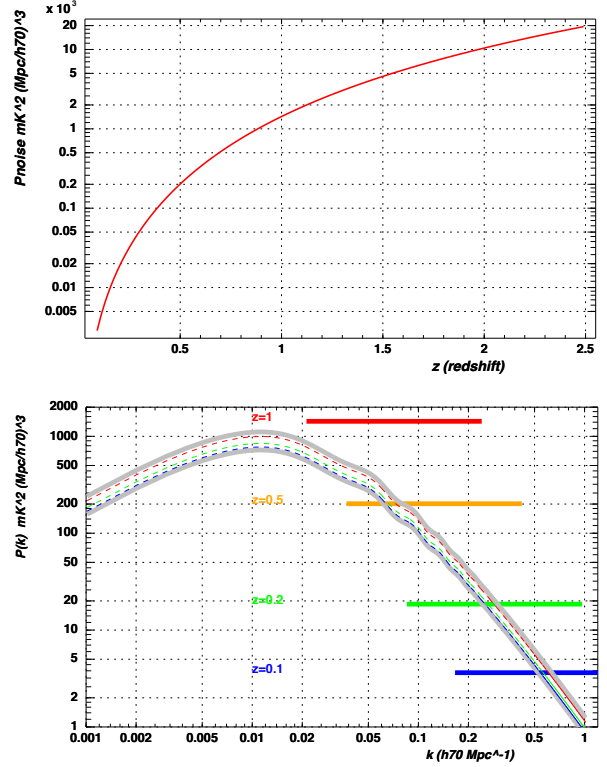
Figure 2. Top: White noise power spectrum P_{\text{noise}}(z) level as a function of redshift for a survey similar to T16DPA with an angular map pixel size of 0.2^{\circ} and 1MHz, and for per pixel noise level \sigma_T^2 = 10\text{mK}^2 . Bottom: Projected noise power spectrum P_{\text{noise}}(k) and the accessible transverse k_{\perp} range for a survey of the NCP region by T16DPA. OP: I'm not sure the top plot is very usefull, everything is said in formula 1 right ?
