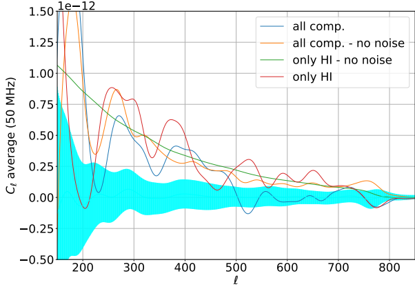
Figure 15. Smoothed cross power spectra averaged over frequencies from bin 3, for different simulation combinations, after foreground subtraction. The cyan band outlines the dispersion around central values of the average of the cross power spectra between maps from the simulation combining all components and noise and the 100 shuffled data cubes.
