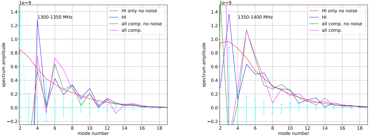
Figure 18. Reconstructed averaged spectra in the two frequency intervals corresponding to bins 2 (left) and 3 (right) from table 4. We compare results obtained from various simulation parameters, from the ideal (only HI sources, no noise) to the complete case. On both sides, the cyan results represent the averages and dispersions from the power spectra from the cross-correlations with a set of 100 shuffled catalogs.
