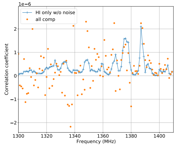
Figure 17. Raw correlation coefficient computed \langle RecSky(\nu) \times Src(\nu) \rangle , for each frequency plane. Blue curve (and crosses) correspond to the case where only H_I sources were contributing to the simulated visibilities, while orange circles correspond to the case where visibilities were computed from all sky components (foregrounds and H_I sources) and include 5mK noise.
