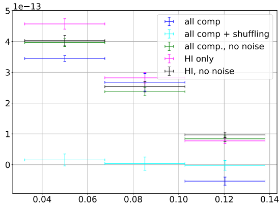
Figure 16. Average of the cross-correlation C_\ell in the interval \ell \in [250, 500] for each of the redshift bins defined in table 4
