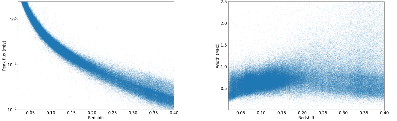
Figure B2. 21 cm flux and frequency width as a function of redshift for our simulated HI source set extrapolated from the SDSS catalogs.
