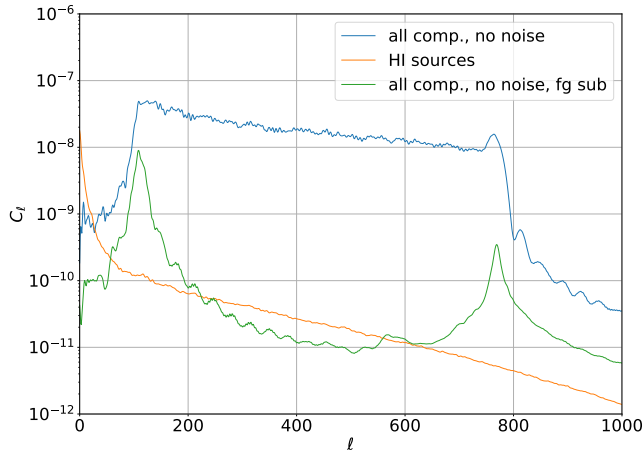
Figure 13. Average of auto-correlation spectra ( C_\ell ) for frequencies between 1350 and 1375 MHz. Blue and green curves correspond to the sky cubes with all components, with no noise added on visibilities, before (blue) and after (green) foreground subtraction (using polynomial fit in frequency domain). The orange curve is the auto-correlation spectrum from the corresponding source cube.
