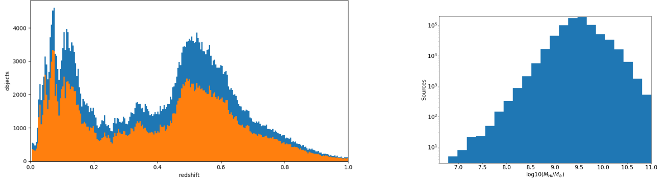
Figure B1. Redshift (left) and HI Mass (extrapolated from optical photometry) distributions from the SDSS catalog sources use in our simulations. The orange distribution correspond to our final source selection.
