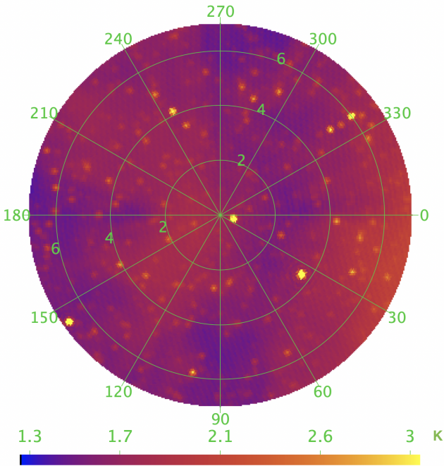
Figure 1. Foreground map of a circular area of 7 deg. radius region around the NCP at 1350 MHz, smoothed with a 15arcmin resolution gaussian beam. Haslam map of diffuse emission at 408 MHz as well as NVSS radiosources, extrapolated to 1350 MHz with a spectral index \beta = -2 have been co-added. The color scale corresponds to temperature in Kelvin.
