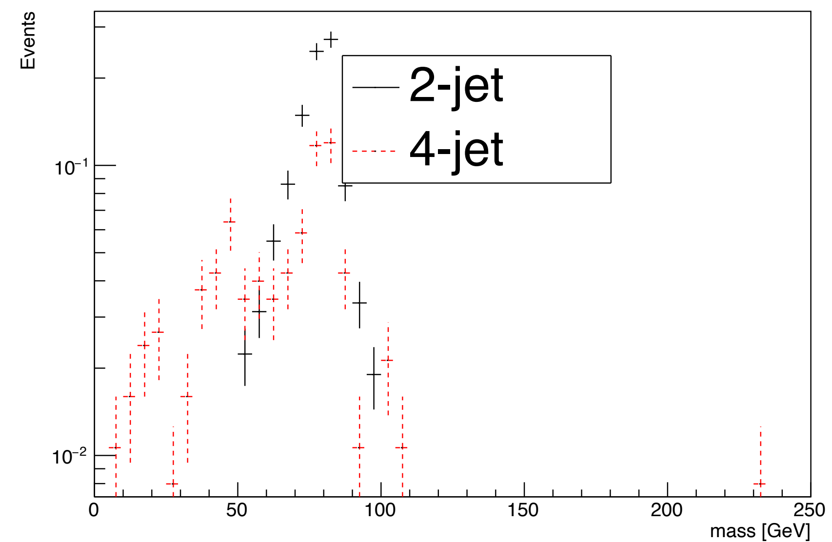
Only hadronic decays allowed 2-jet
