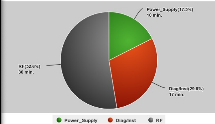
SYSTEMS Downtime refined by LINAC, Beam_Inhibit_Failure from 5/6/2022 08:00:00 to 5/13/2022 08:00:00 (168.0 hrs.)
