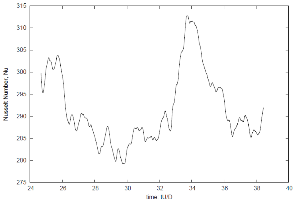
Figure 9: Nusselt number fluctuates for about 5% at Re = 10K after long run time insert and the pipe wall.
