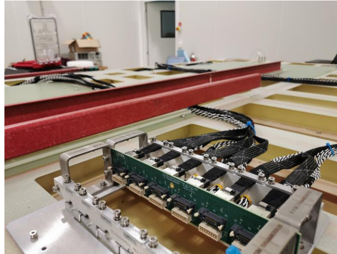
Check tine guides
