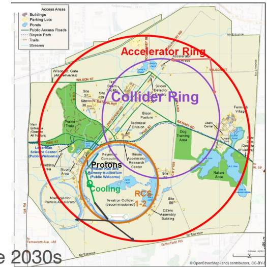
A 6-10 TeV Muon collider can fit on Fermilab site
