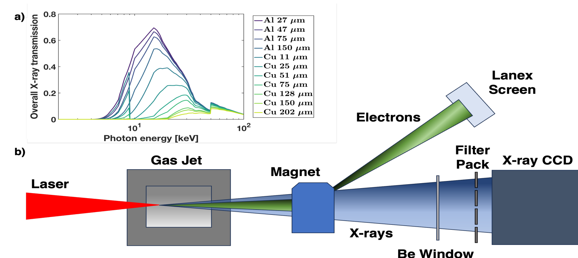
Figure 1: (a) Transmission curves for each filter, including the quantum efficiency of the camera. (b) Top-down view of the experimental setup with the density gradient and subsequent streaking motion illustrated via color gradients, towards the direction of the lighter color.
