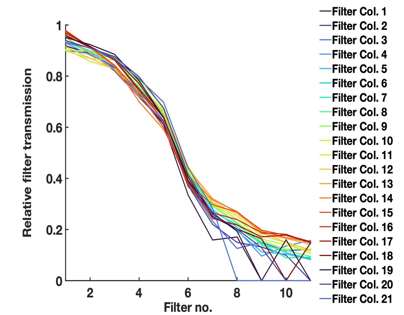
Figure 4: Relative transmission through the filters of each column, with missing or blocked filters counted as zeros.
