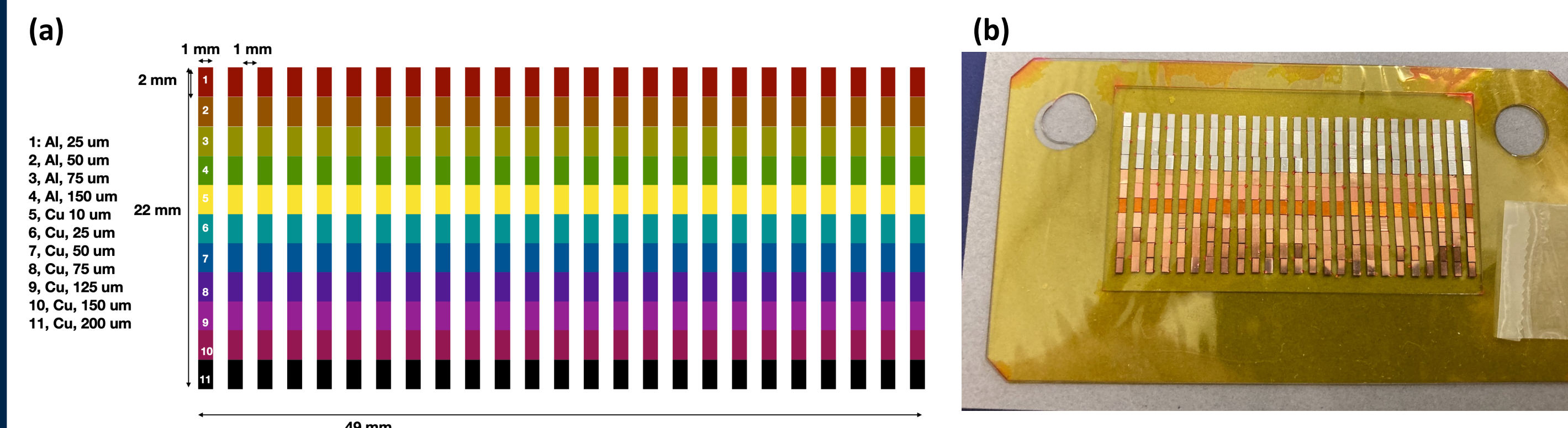
Figure 2: (a) Color-coded filter pack schematic listing the thickness, position, and material of each filter. Each column is identical and contains aluminum and copper filters. (b) Physical version of the filter pack used in the experiment.
