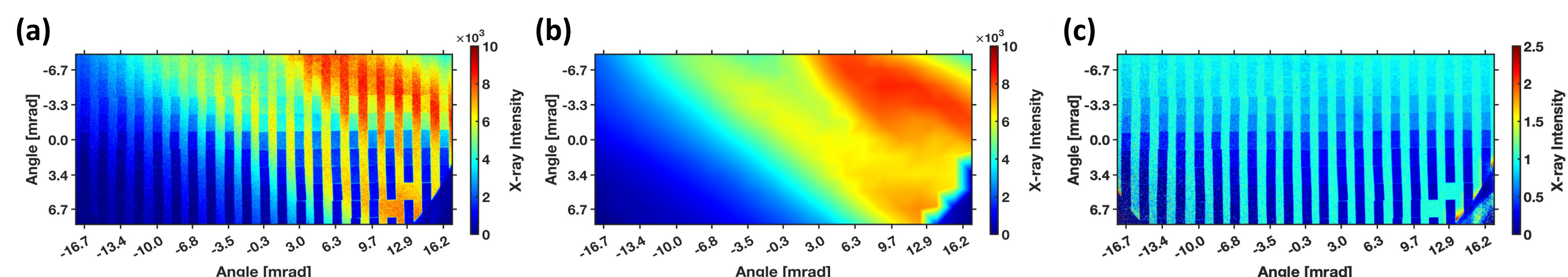
Figure 3: (a) Original image showing raw X-ray counts. (b) Interpolated spatial profile of the streaked X-rays. (c) Flattened spatial profile without nonuniformities.
