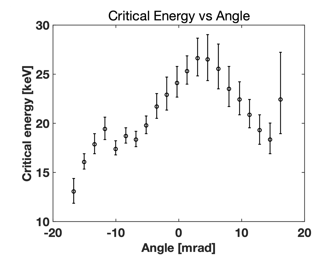
Figure 6: Critical energy versus angle showing the change in energy as the X-rays streak across the camera.
