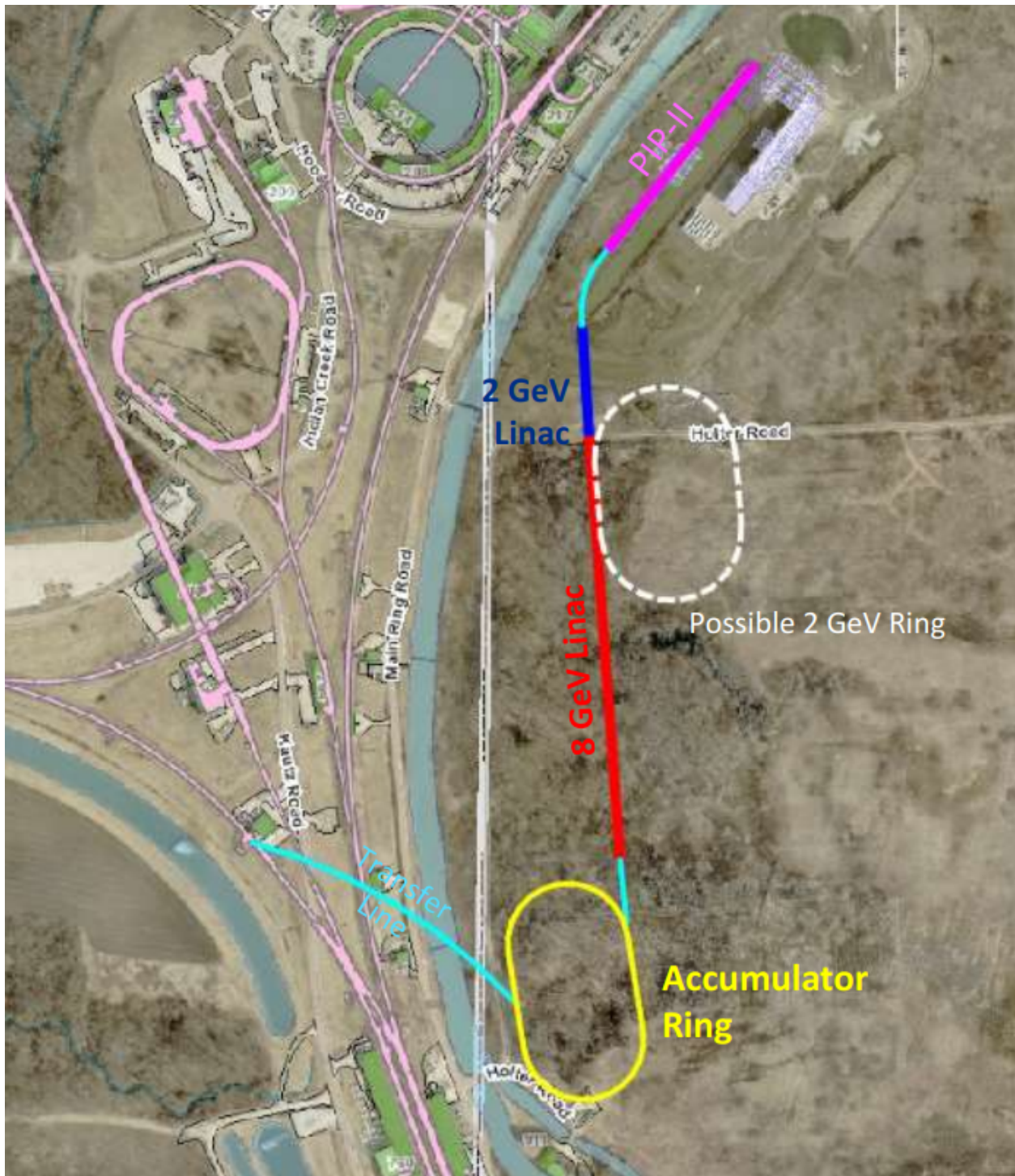
Figure 10: Schematic overview of a possible layout for an 8 GeV Linac PIU scenario. Following the PIP-II linac, a transport directs the beam into a 2 GeV linac extension ( 100 m) which is followed by an 350m Linac that accelerates the beam to 8 GeV. This is followed by a short transport that injects the 8 GeV beam into an Accumulator Ring. A transfer line ( 320 m long) would transport the accumulated 8 GeV protons into the Recycler Ring at RR-62, or the Main Injector at MI-62. A 2 GeV storage Ring could be added to accumulate beam from the 2 GeV linac for use in low-energy intensity frontier experiments.
