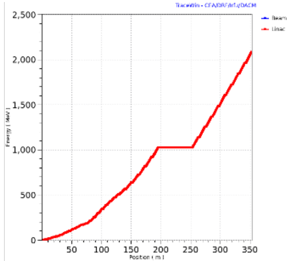
Figure 15: Evolution of the beam energy along the PIP-II linac and 2 GeV extension.
