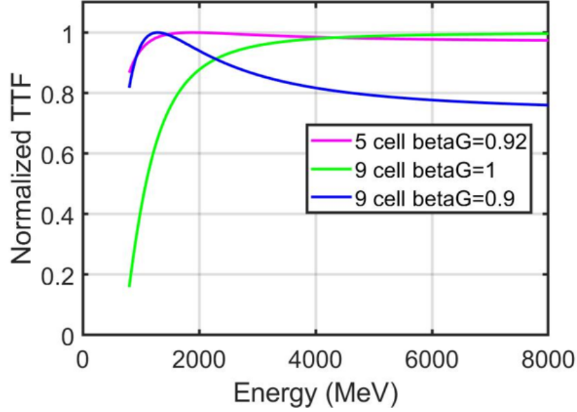
Figure 17: Transit time factors for a \beta = 0.92 650 MHz 5-cell cavity (as in PIP-II and the 2 GeV extension), a \beta = 1 1.3 GHz 9-cell cavity (as in E-XFEL and LCLS-II), and a potential \beta = 0.9 1.3 GHz 9-cell cavity.
