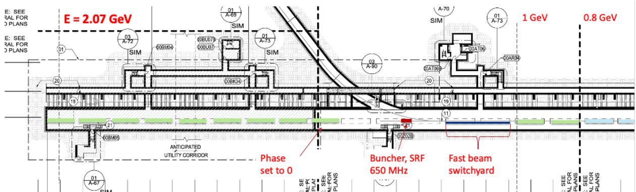
Figure 13: Layout of the 2 GeV extension with beam running from right to left. Cryomodules included in the upgrade are shown in light green, while the PIP-II baseline cryomodules are light blue.
