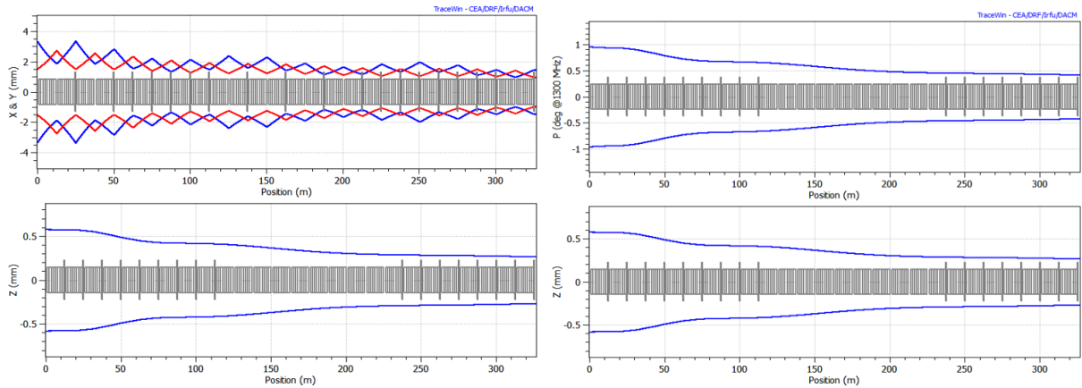
Figure 18: Optics for the 2→8 GeV linac based on a 31.5 MV/m accelerating gradient.
