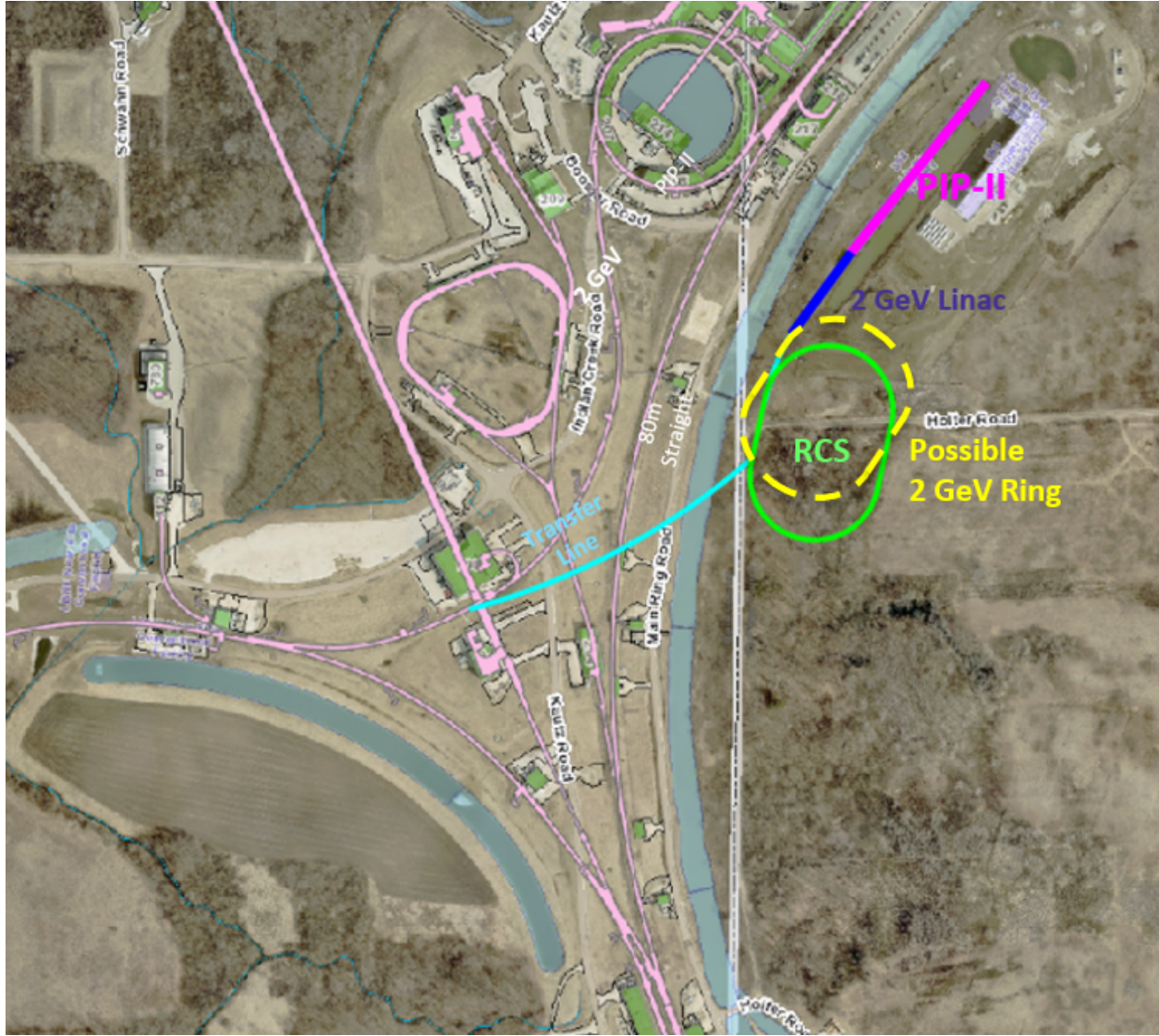
Figure 9: Schematic overview of a possible PIU scenario layout for an RCS accelerator. The PIP-II Linac leads into an extension that accelerates the beam to 2 GeV. A transport line injects that beam into the 8 GeV RCS accelerator. 8 GeV beam from the RCS is transported through a new transfer line into the Booster to MI transport (MI-8) for injection into the Recycler Ring at RR-10. The transfer line is 300 m long and is followed by 220 m of transport using the MI-8 line. The 2 GeV beam could instead be directed into an accumulator ring (shown in yellow) and transferred to the RCS after accumulation. The 2 GeV ring could also provide beam to a 2 GeV experimental program.
