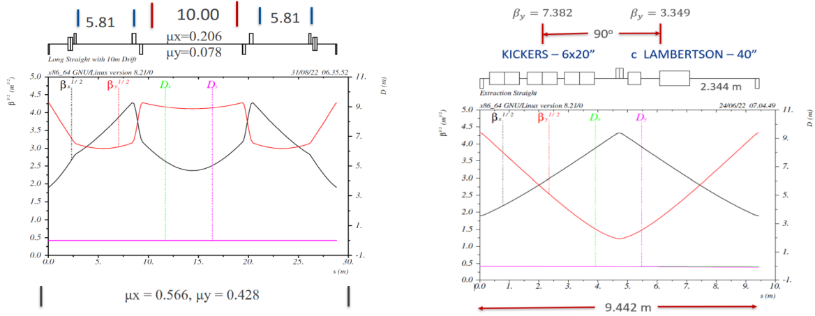
(a) The PAR injection lattice with a 10 meter straight. (b) The PAR extraction lattice with 3 sets of short kickers.
