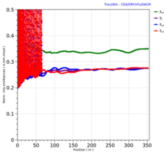
Figure 14: Evolution of the beam emittances along the linac with 2 GeV extension.
