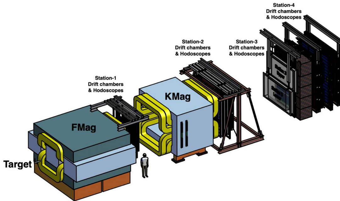
Figure 1. The spectrometer layout in the lower level of NM4 which was repurposed from the SeaQuest experiment for E1039 SpinQuest. Beam is traveling from left to right in the image. FMag and KMag are two large electromagnets. FMag is a closed aperture solid iron magnet to focus muons downstream and absorb beam protons which did not interact with the target. KMag is a large open aperture magnet to measure muon momenta.
