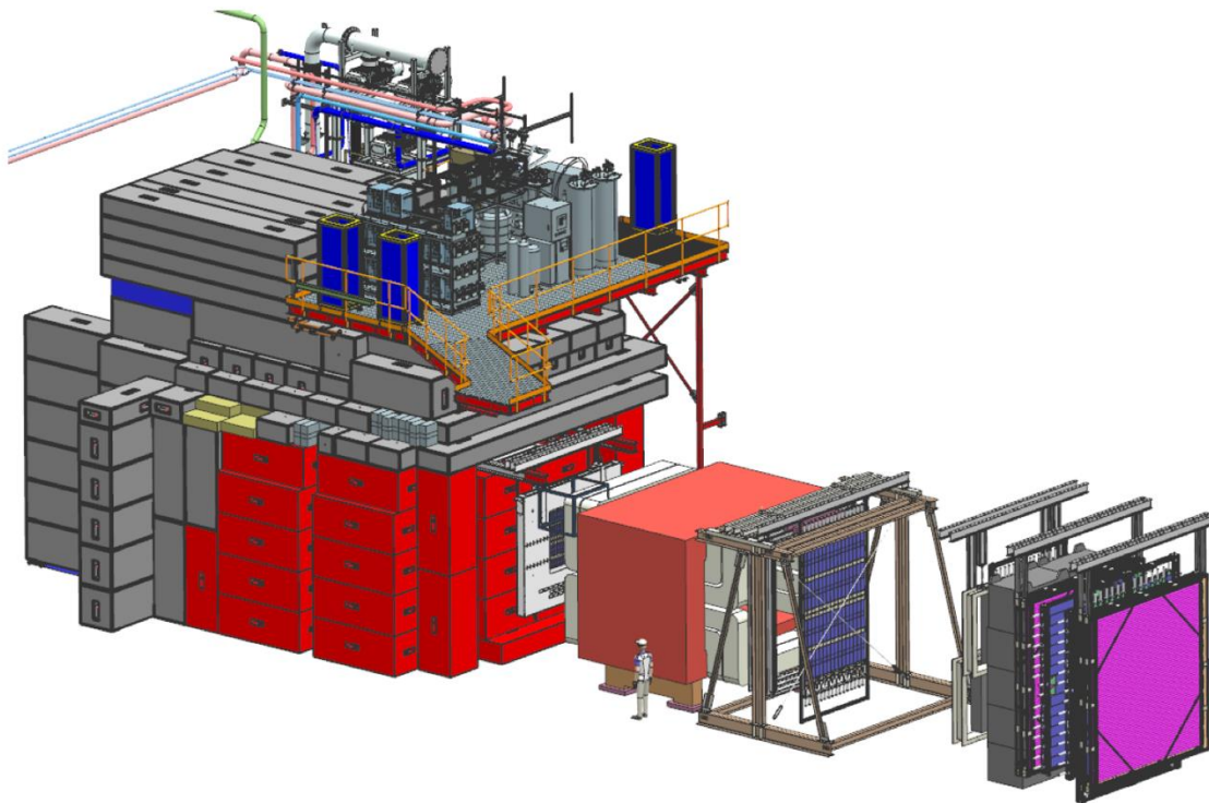
Figure 2. The target Cave and spectrometer looking from down stream. The red shielding blocks are surrounding FMag. Pictured on the upper level is the cryogenics platform for manufacturing liquid helium installed for E1039.
