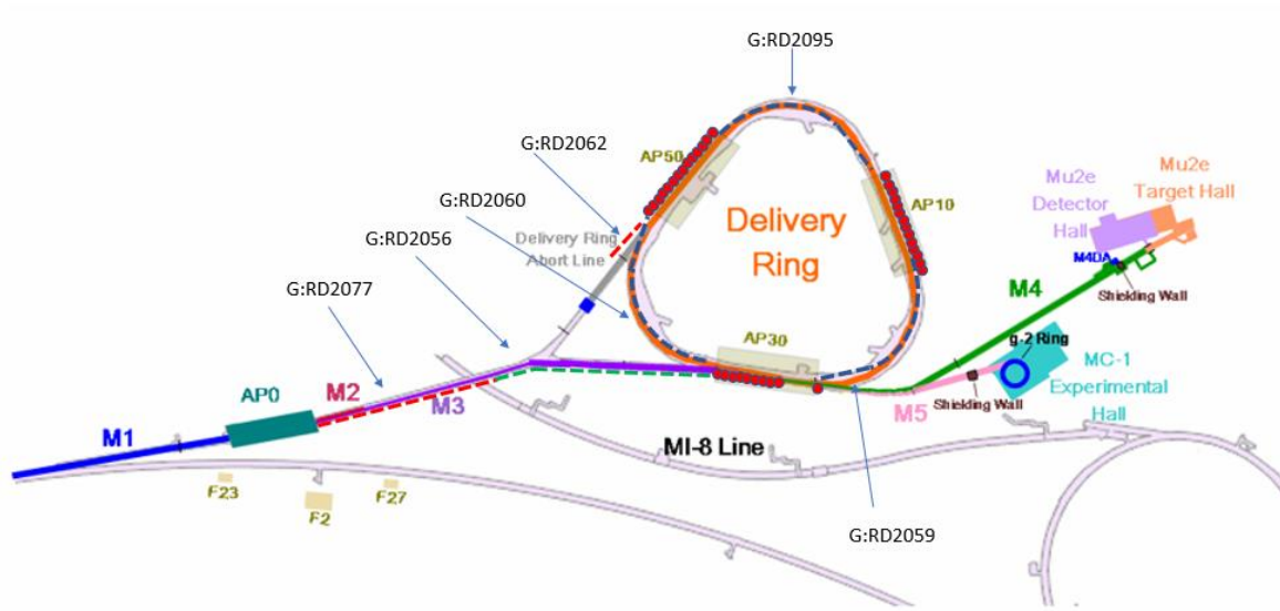
Figure 7: Locations of credited Chipmunk detectors
