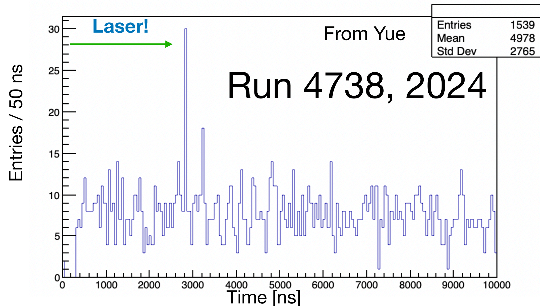
(LAPPDDataTimeStampUL-LAPPDDataBeamgateUL)*3.125 (LAPPDDataTimeStampUL=0 && LAPPD_ID=0)
