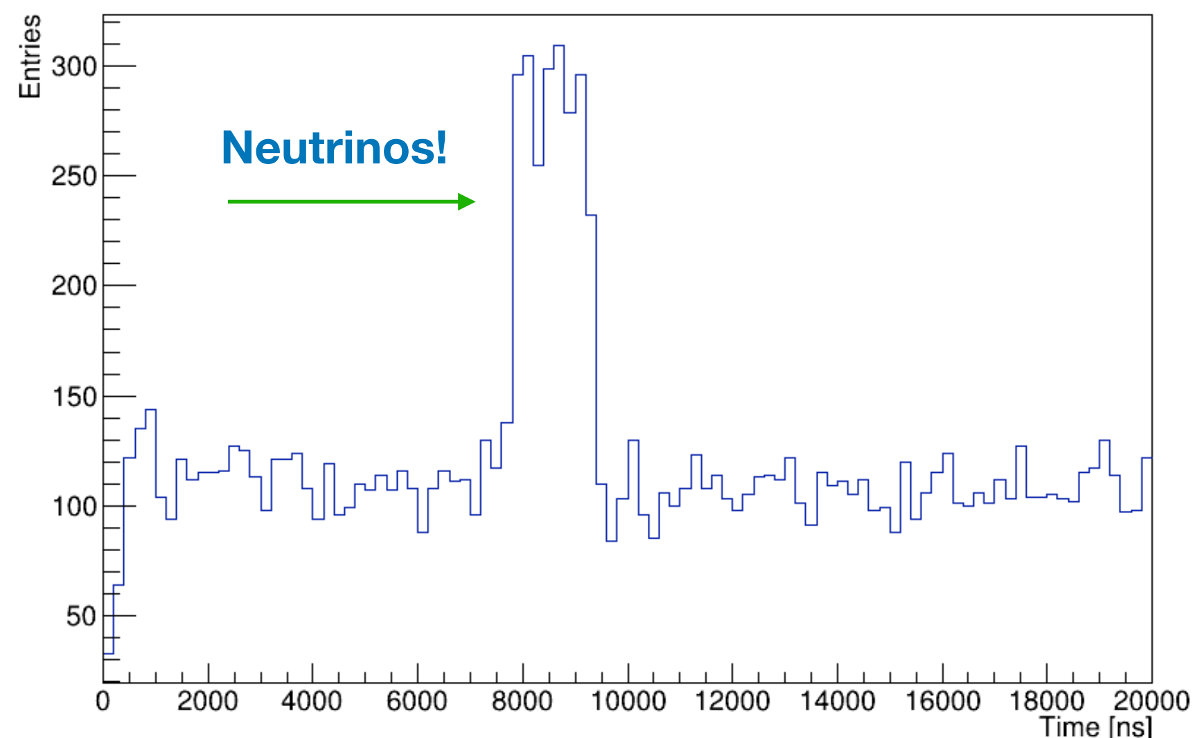
(LAPPDDataTimeStampUL-LAPPDDataBeamgateUL)*3.125 (LAPPDDataTimeStampUL=0 && LAPPD_ID=0)
