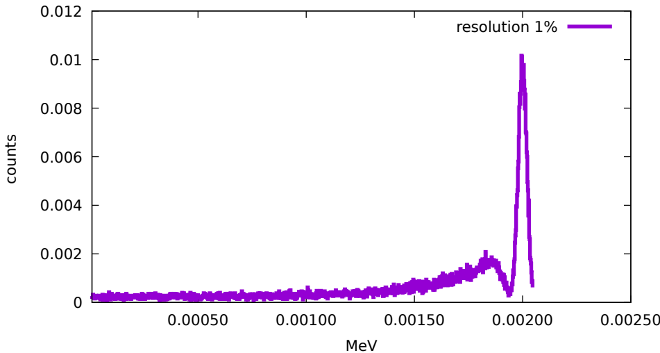
Energy deposited, 2MeV photons from centre of TPC
