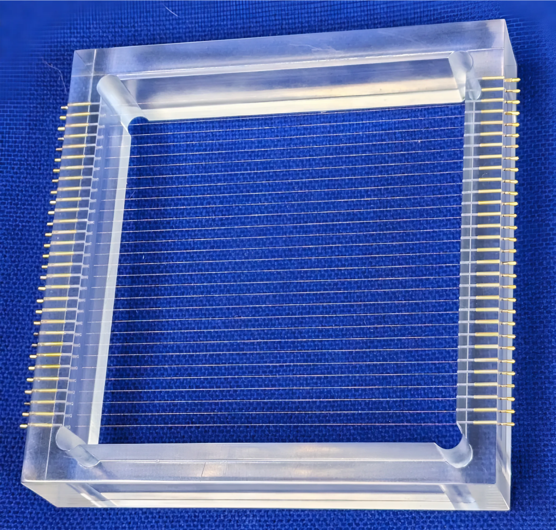
Setup for testing crimping pins based on machined plexiglass frame
