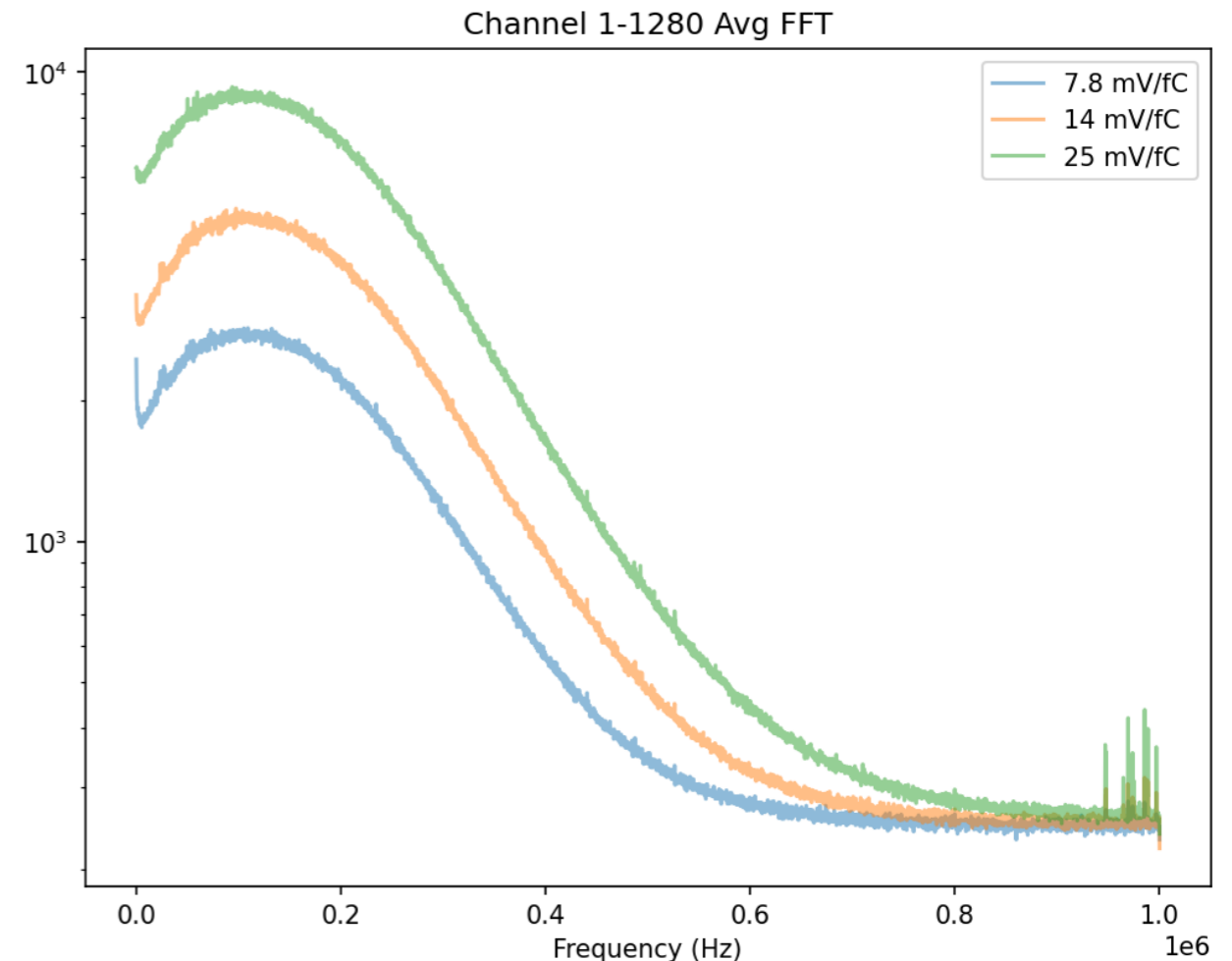
Average FFT of all channels under various gain settings.
